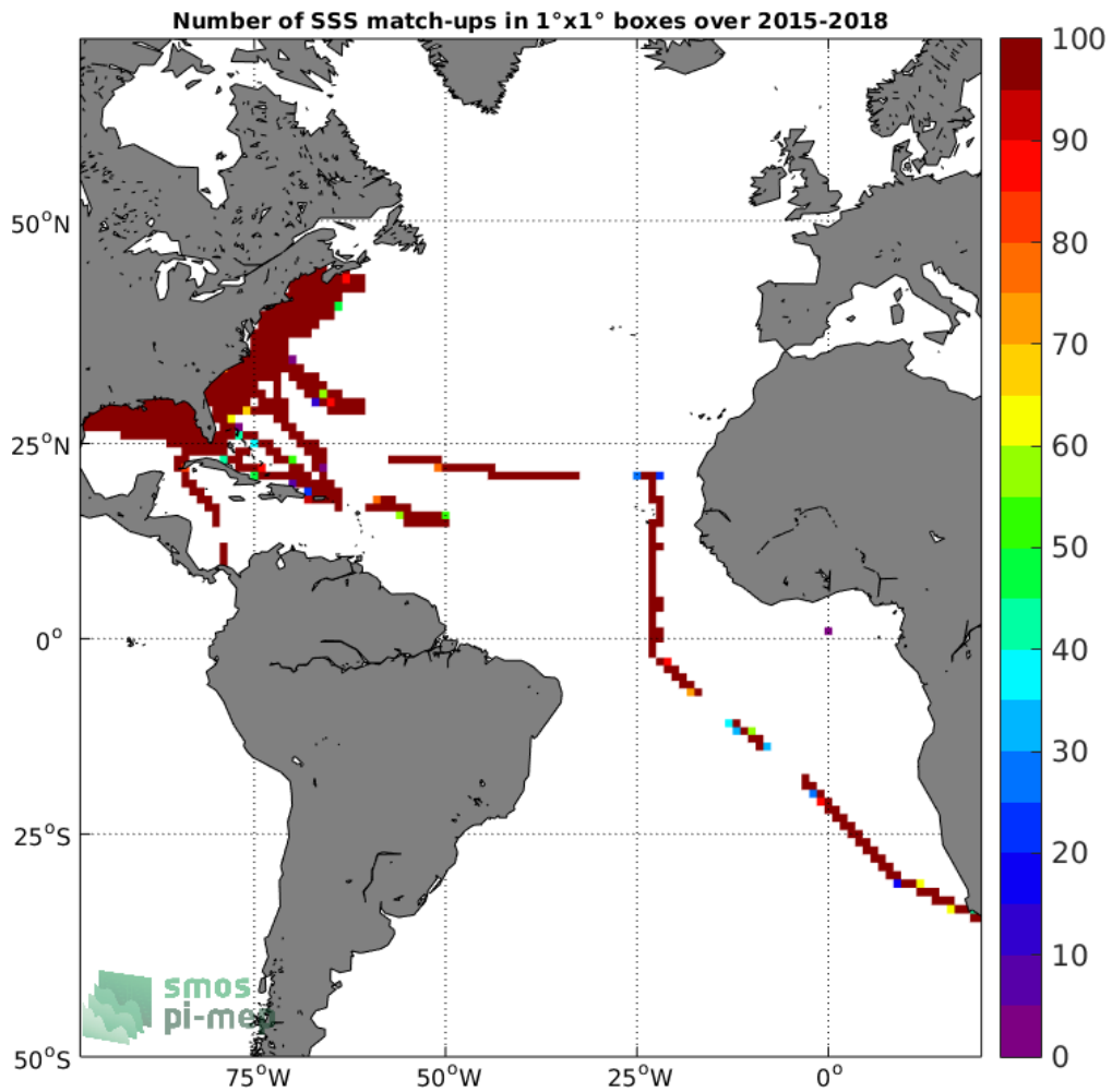
Figure 4: Number of SSS match-ups between TSG-SAMOS SSS and the SMAP-L3-JPL-V4.2-8DAY-RUNNING-60KM SSS product for the Atlantic Ocean Pi-MEP region over 1°x1° boxes and for the full satellite product period.
