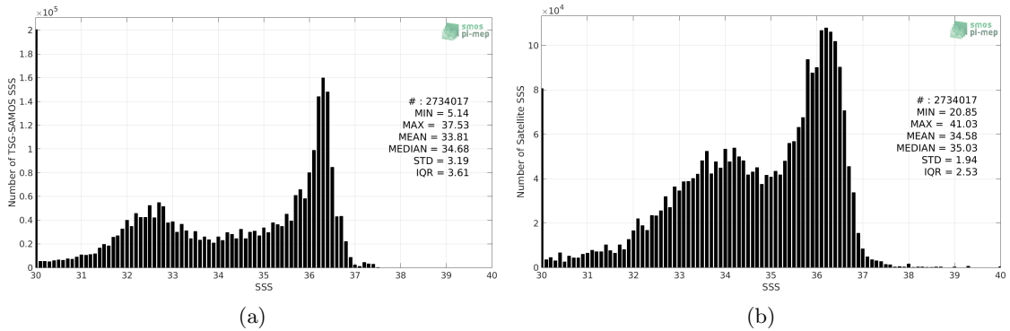
Figure 2: Histograms of SSS from TSG-SAMOS (a) and SMAP-L3-JPL-V4.2-8DAY-RUNNING-60KM (b) considering all match-up pairs per bins of 0.1 over the Atlantic Ocean Pi-MEP region and for the full satellite product period.
