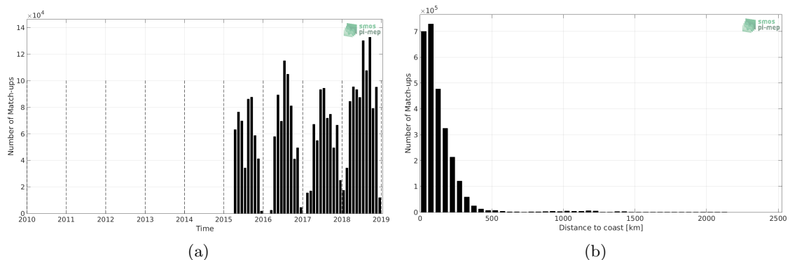
Figure 1: Number of match-ups between TSG-SAMOS and SMAP-L3-JPL-V4.2-8DAY-RUNNING-60KM SSS as a function of time (a) and as function of the distance to coast (b) over the Atlantic Ocean Pi-MEP region and for the full satellite product period.
