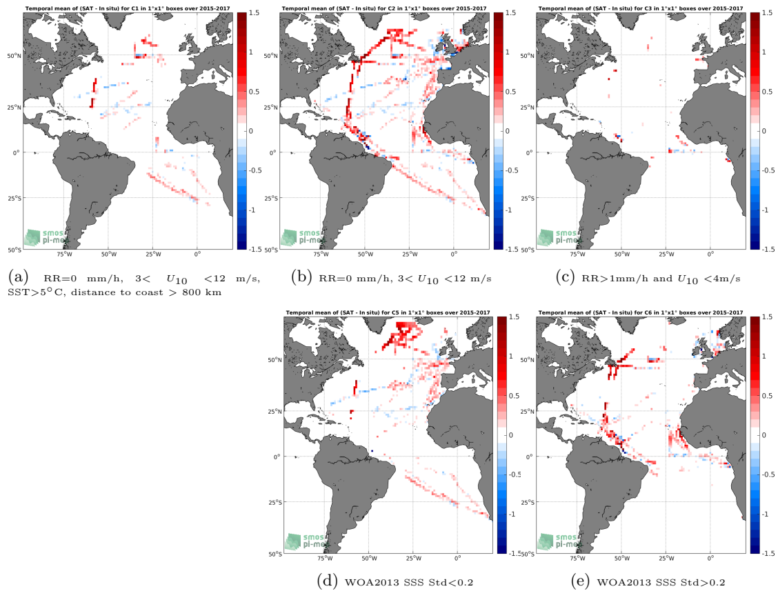
Figure 12: Temporal mean gridded over spatial boxes of size 1^\circ \times 1^\circ of \Delta SSS (SMAP-L3-JPL-V4.2-8DAY-RUNNING-60KM - TSG-GOSUD-Research-vessel) for 5 different subdatasets corresponding to:RR=0 mm/h, 3 < U_{10} < 12 m/s, SST >5^\circ\text{C} , distance to coast > 800 km (a), RR=0 mm/h, 3 < U_{10} < 12 m/s (b), RR >1 mm/h and U_{10} < 4 m/s (c), WOA2013 SSS Std <0.2 (d), WOA2013 SSS Std >0.2 (e).
