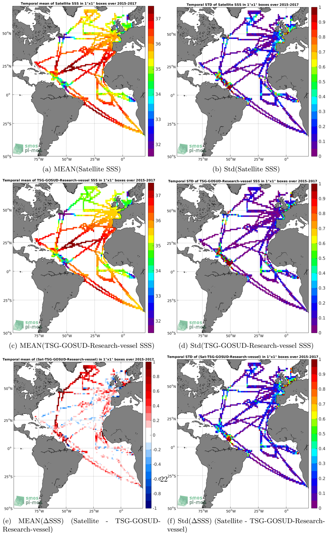
Figure 6: Temporal mean (left) and Std (right) of SSS from SMAP-L3-JPL-V4.2-8DAY-RUNNING-60KM (top), TSG-GOSUD-Research-vessel (middle), and of ΔSSS (Satellite - TSG-GOSUD-Research-vessel). Only match-up pairs are used to generate these maps.
