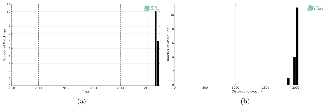
Figure 1: Number of match-ups between Sea mammals and SMAP-L3-JPL-V4.2-8DAY-RUNNING-60KM SSS as a function of time (a) and as function of the distance to coast (b) over the Atlantic Ocean Pi-MEP region and for the full satellite product period.
