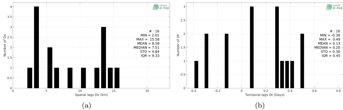
Figure 5: Histograms of the spatial (a) and temporal (b) lags between the time of the Sea mammals measurements and the date of the corresponding SMAP-L3-JPL-V4.2-8DAY-RUNNING-60KM SSS product.
