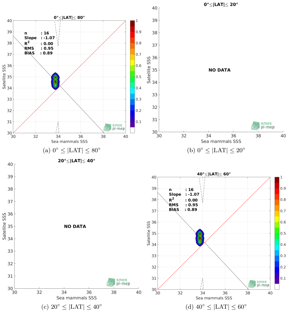
Figure 9: Contour maps of the concentration of SMAP-L3-JPL-V4.2-8DAY-RUNNING-60KM SSS (y-axis) versus Sea mammals SSS (x-axis) at match-up pairs for different latitude bands. For each plot, the red line shows x=y . The black thin and dashed lines indicate a linear fit through the data cloud and the \pm 95\% confidence levels, respectively. The number match-up pairs n , the slope and R^2 coefficient of the linear fit, the root mean square (RMS) and the mean bias between satellite and in situ data are indicated for each latitude band in each plots.
