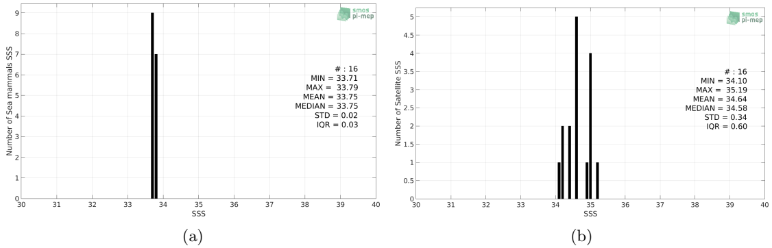
Figure 2: Histograms of SSS from Sea mammals (a) and SMAP-L3-JPL-V4.2-8DAY-RUNNING-60KM (b) considering all match-up pairs per bins of 0.1 over the Atlantic Ocean Pi-MEP region and for the full satellite product period.
