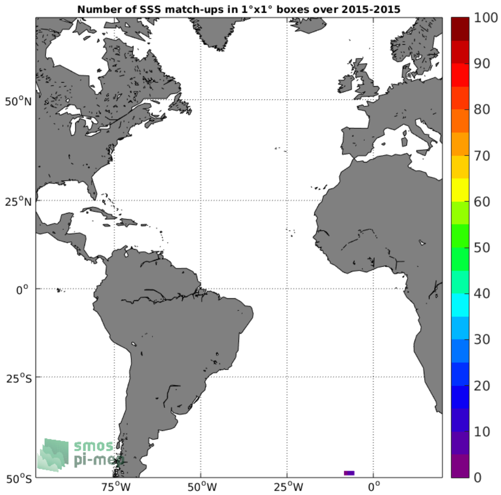
Figure 4: Number of SSS match-ups between Sea mammals SSS and the SMAP-L3-JPL-V4.2-8DAY-RUNNING-60KM SSS product for the Atlantic Ocean Pi-MEP region over 1°x1° boxes and for the full satellite product period.
