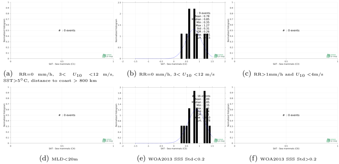
Figure 13: Normalized histogram of \Delta SSS (SMAP-L3-JPL-V4.2-8DAY-RUNNING-60KM - Sea mammals) for 6 different subdatasets corresponding to: RR=0 mm/h, 3 < U_{10} < 12 m/s, SST >5^{\circ} C, distance to coast > 800 km (a), RR=0 mm/h, 3 < U_{10} < 12 m/s (b), RR >1 mm/h and U_{10} < 4 m/s (c), MLD <20 m (d), WOA2013 SSS Std <0.2 (e), WOA2013 SSS Std >0.2 (f).
