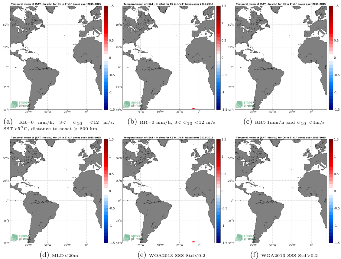
Figure 12: Temporal mean gridded over spatial boxes of size 1^\circ \times 1^\circ of \Delta SSS (SMAP-L3-JPL-V4.2-8DAY-RUNNING-60KM - Sea mammals) for 6 different subdatasets corresponding to:RR=0 mm/h, 3 < U_{10} < 12 m/s, SST >5^\circ C, distance to coast > 800 km (a), RR=0 mm/h, 3 < U_{10} < 12 m/s (b), RR >1 mm/h and U_{10} < 4 m/s (c),MLD <20 m (d),WOA2013 SSS Std <0.2 (e),WOA2013 SSS Std >0.2 (f).
