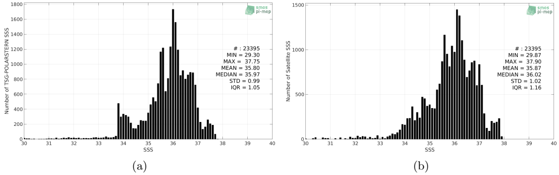
Figure 2: Histograms of SSS from TSG-POLARSTERN (a) and SMAP-L3-JPL-V4.2-MONTHLY-60KM (b) considering all match-up pairs per bins of 0.1 over the Atlantic Ocean Pi-MEP region and for the full satellite product period.
