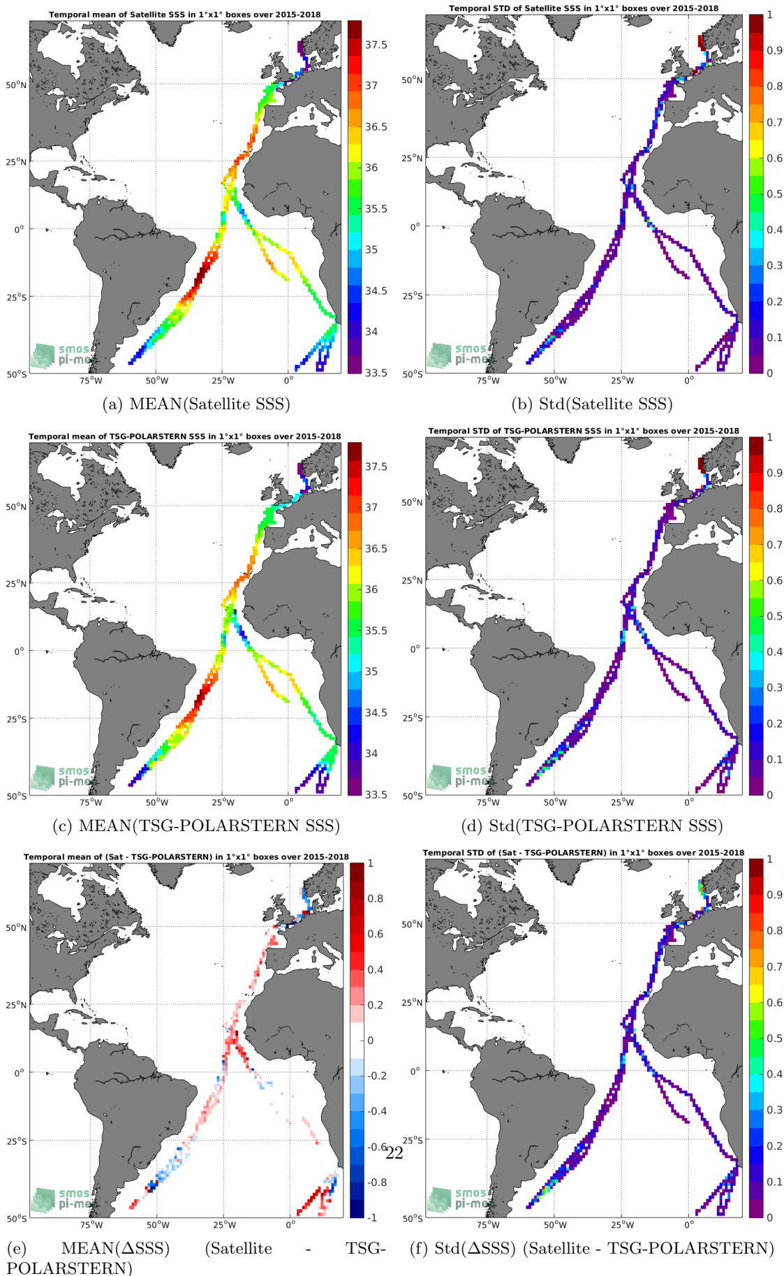
Figure 6: Temporal mean (left) and Std (right) of SSS from SMAP-L3-JPL-V4.2-MONTHLY-60KM (top), TSG-POLARSTERN (middle), and of \Delta SSS (Satellite - TSG-POLARSTERN). Only match-up pairs are used to generate these maps.
