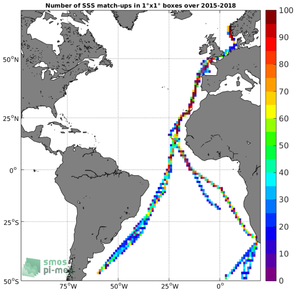
Figure 4: Number of SSS match-ups between TSG-POLARSTERN SSS and the SMAP-L3-JPL-V4.2-MONTHLY-60KM SSS product for the Atlantic Ocean Pi-MEP region over 1°x1° boxes and for the full satellite product period.
