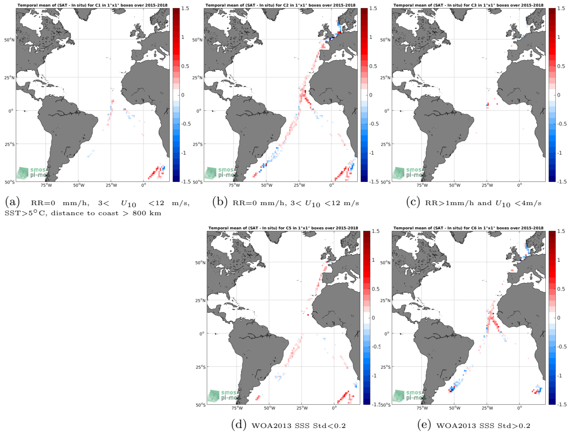
Figure 12: Temporal mean gridded over spatial boxes of size 1^\circ \times 1^\circ of \Delta SSS (SMAP-L3-JPL-V4.2-MONTHLY-60KM - TSG-POLARSTERN) for 5 different subdatasets corresponding to:RR=0 mm/h, 3 < U_{10} < 12 m/s, SST >5^\circ\text{C} , distance to coast > 800 km (a), RR=0 mm/h, 3 < U_{10} < 12 m/s (b), RR >1 mm/h and U_{10} < 4 m/s (c), WOA2013 SSS Std <0.2 (d), WOA2013 SSS Std >0.2 (e).
