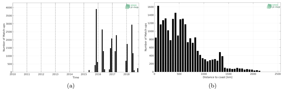
Figure 1: Number of match-ups between TSG-POLARSTERN and SMAP-L3-JPL-V4.2-MONTHLY-60KM SSS as a function of time (a) and as function of the distance to coast (b) over the Atlantic Ocean Pi-MEP region and for the full satellite product period.
