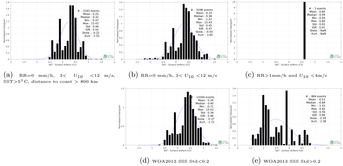
Figure 12: Normalized histogram of \Delta SSS (SMAP-L3-JPL-V4.2-MONTHLY-60KM - Surface drifters) for 5 different subdatasets corresponding to: RR=0 mm/h, 3 < U_{10} < 12 m/s, SST > 5°C, distance to coast > 800 km (a), RR=0 mm/h, 3 < U_{10} < 12 m/s (b), RR > 1mm/h and U_{10} < 4 m/s (c), WOA2013 SSS Std < 0.2 (d), WOA2013 SSS Std > 0.2 (e).
