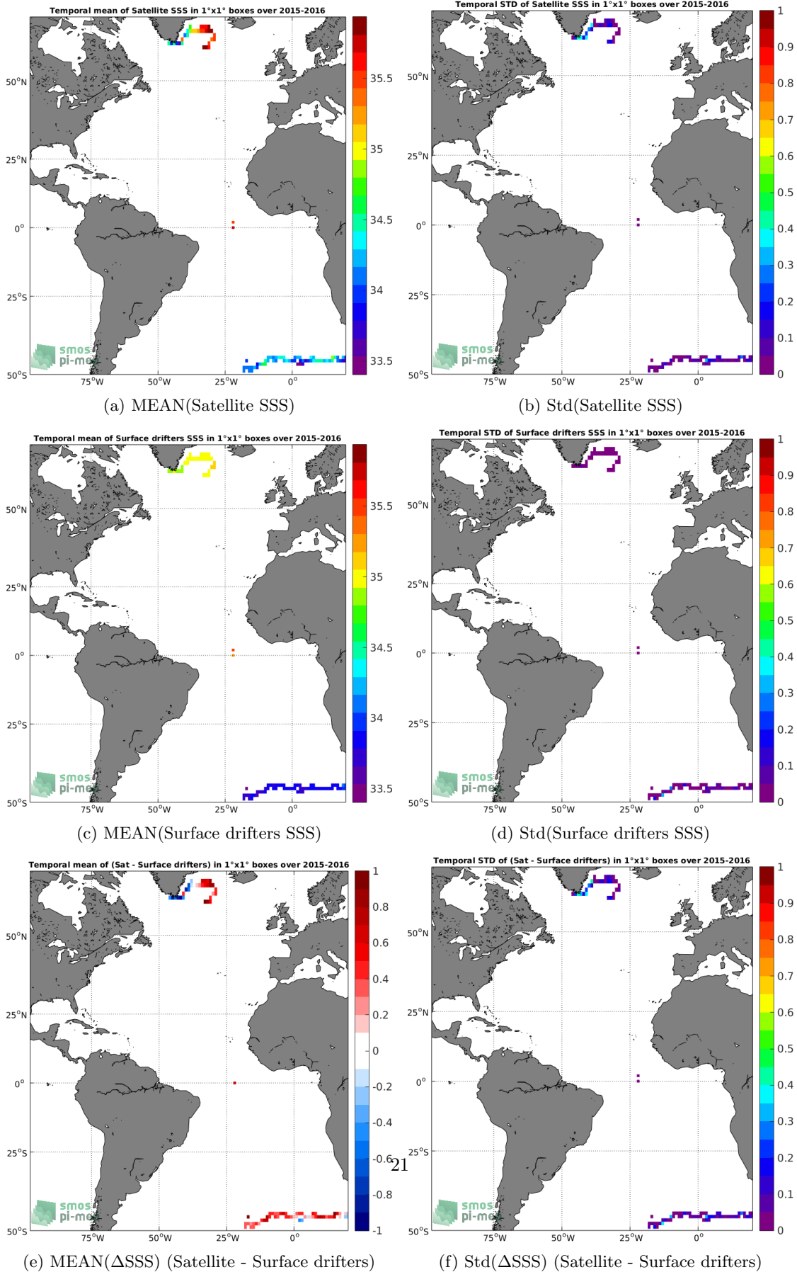
Figure 5: Temporal mean (left) and Std (right) of SSS from SMAP-L3-JPL-V4.2-MONTHLY-60KM (top), Surface drifters (middle), and of \Delta SSS (Satellite - Surface drifters). Only match-up pairs are used to generate these maps.
