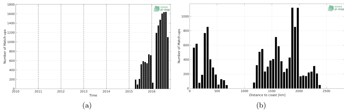
Figure 1: Number of match-ups between Surface drifters and SMAP-L3-JPL-V4.2-MONTHLY-60KM SSS as a function of time (a) and as function of the distance to coast (b) over the Atlantic Ocean Pi-MEP region and for the full satellite product period.
