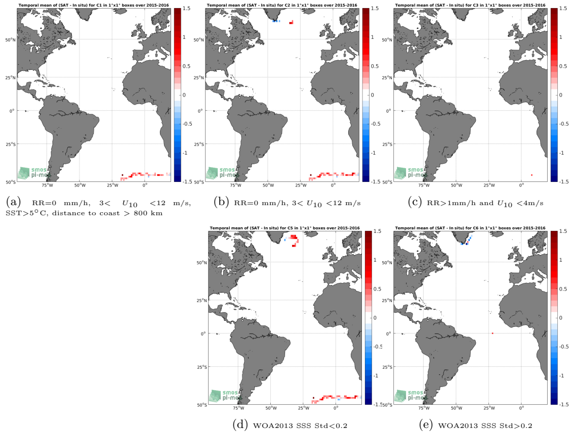
Figure 11: Temporal mean gridded over spatial boxes of size 1^\circ \times 1^\circ of \Delta SSS (SMAP-L3-JPL-V4.2-MONTHLY-60KM - Surface drifters) for 5 different subdatasets corresponding to:RR=0 mm/h, 3 < U_{10} < 12 m/s, SST >5^\circ\text{C} , distance to coast > 800 km (a), RR=0 mm/h, 3 < U_{10} < 12 m/s (b), RR >1 mm/h and U_{10} < 4 m/s (c), WOA2013 SSS Std <0.2 (d), WOA2013 SSS Std >0.2 (e).
