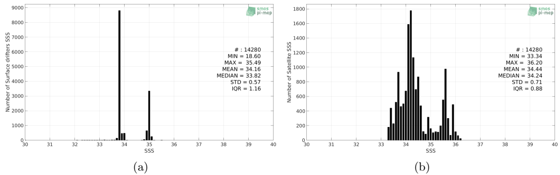
Figure 2: Histograms of SSS from Surface drifters (a) and SMAP-L3-JPL-V4.2-MONTHLY-60KM (b) considering all match-up pairs per bins of 0.1 over the Atlantic Ocean Pi-MEP region and for the full satellite product period.
