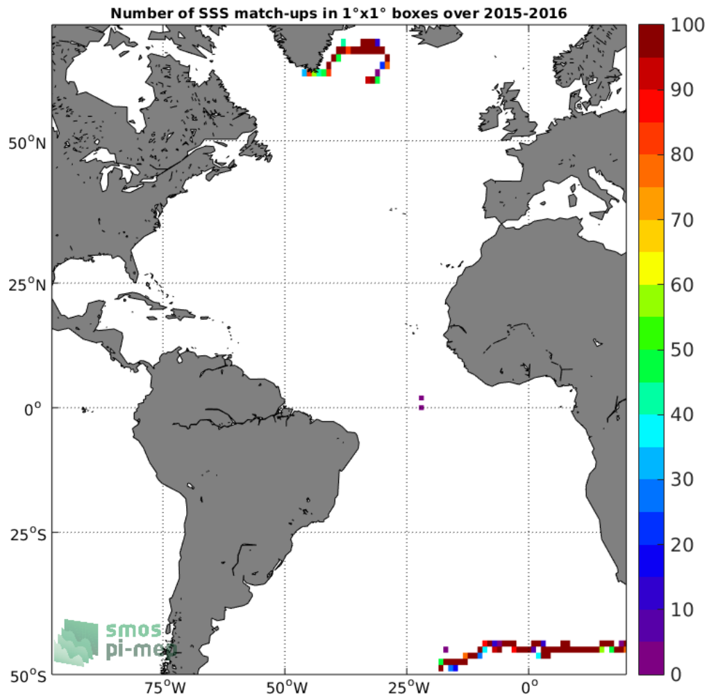
Figure 3: Number of SSS match-ups between Surface drifters SSS and the SMAP-L3-JPL-V4.2-MONTHLY-60KM SSS product for the Atlantic Ocean Pi-MEP region over 1°x1° boxes and for the full satellite product period.
