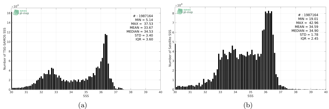
Figure 2: Histograms of SSS from TSG-SAMOS (a) and SMAP-L3-JPL-V4-MONTHLY-60KM (b) considering all match-up pairs per bins of 0.1 over the Atlantic Ocean Pi-MEP region and for the full satellite product period.
