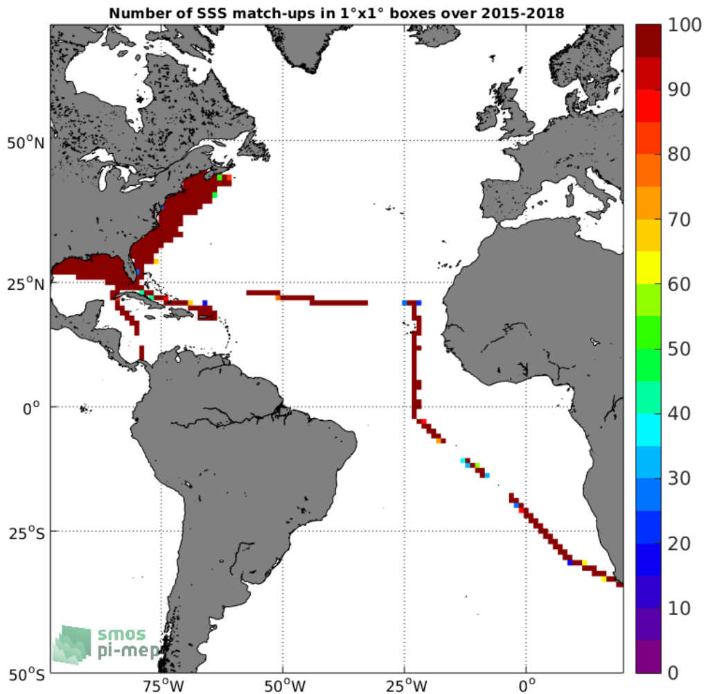
Figure 4: Number of SSS match-ups between TSG-SAMOS SSS and the SMAP-L3-JPL-V4-MONTHLY-60KM SSS product for the Atlantic Ocean Pi-MEP region over 1°x1° boxes and for the full satellite product period.
