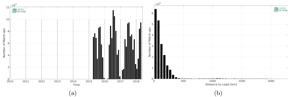
Figure 1: Number of match-ups between TSG-SAMOS and SMAP-L3-JPL-V4-MONTHLY-60KM SSS as a function of time (a) and as function of the distance to coast (b) over the Atlantic Ocean Pi-MEP region and for the full satellite product period.
