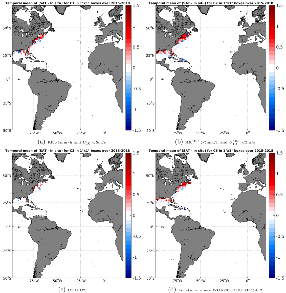
Figure 12: Temporal mean gridded over spatial boxes of size 1^\circ \times 1^\circ of \Delta SSS (SMAP-L3-JPL-V4-MONTHLY-60KM - TSG-SAMOS) for 4 different subdatasets corresponding to:RR > 1 mm/h and U_{10} < 5 m/s (a), RR^{10d} > 5 mm/h and U_{10}^{10d} < 5 m/s (b), C1 U C2 (c),Locations where WOA2013 SSS STD > 0.2 (d).
