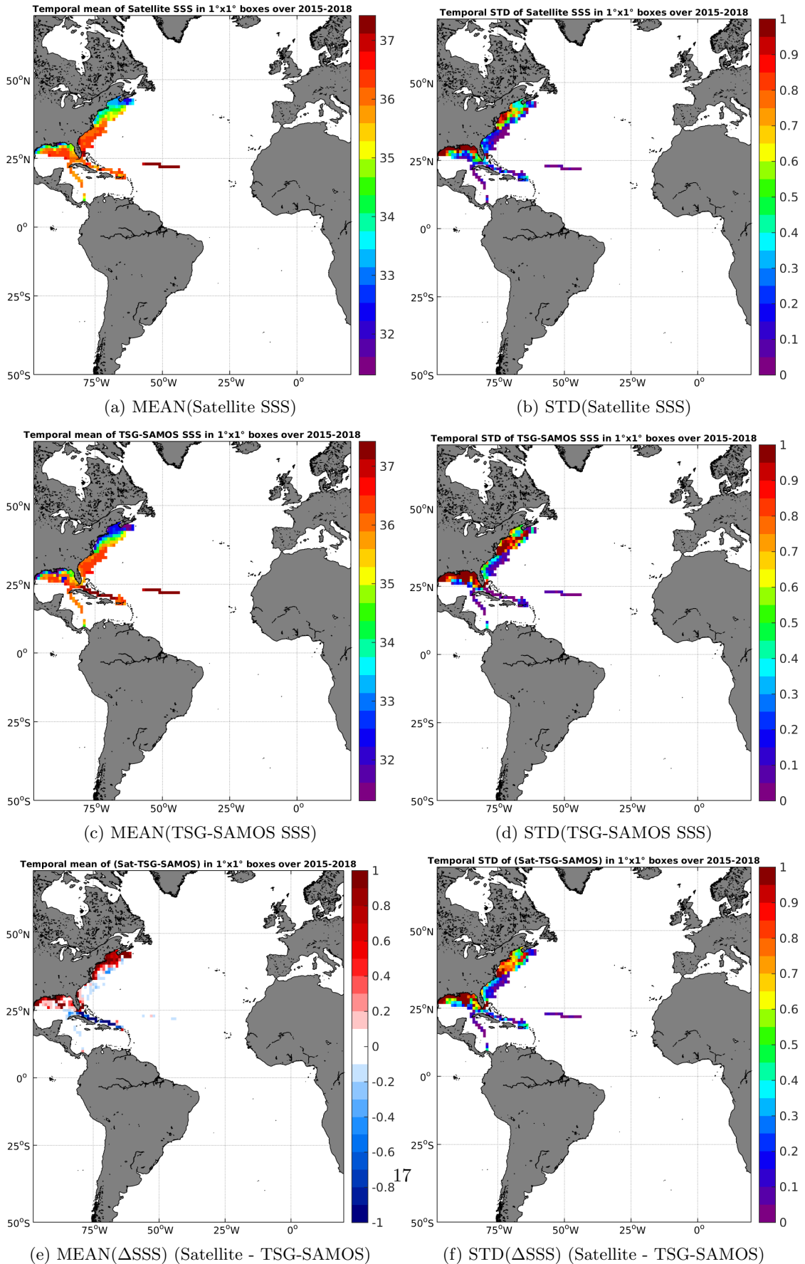
Figure 6: Temporal mean (left) and STD (right) of SSS from SMAP-L3-JPL-V4-MONTHLY-60KM (top), TSG-SAMOS (middle), and of \Delta SSS (Satellite - TSG-SAMOS). Only match-up pairs are used to generate these maps.
