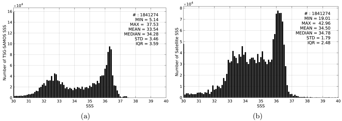
Figure 2: Histograms of SSS from TSG-SAMOS (a) and SMAP-L3-JPL-V4-MONTHLY-60KM (b) considering all match-up pairs per bins of 0.1 over the Atlantic Ocean Pi-MEP region and for the full satellite product period.
