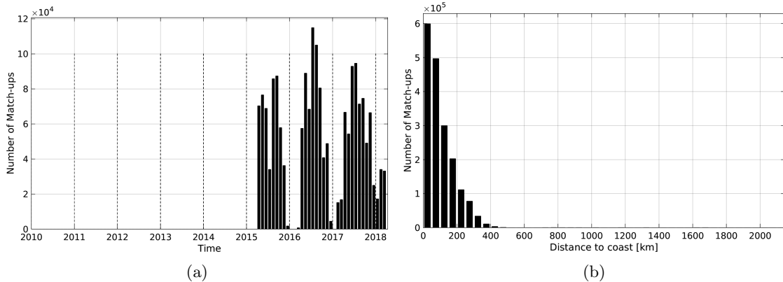
Figure 1: Number of match-ups between TSG-SAMOS and SMAP-L3-JPL-V4-MONTHLY-60KM SSS as a function of time (a) and as function of the distance to coast (b) over the Atlantic Ocean Pi-MEP region and for the full satellite product period.
