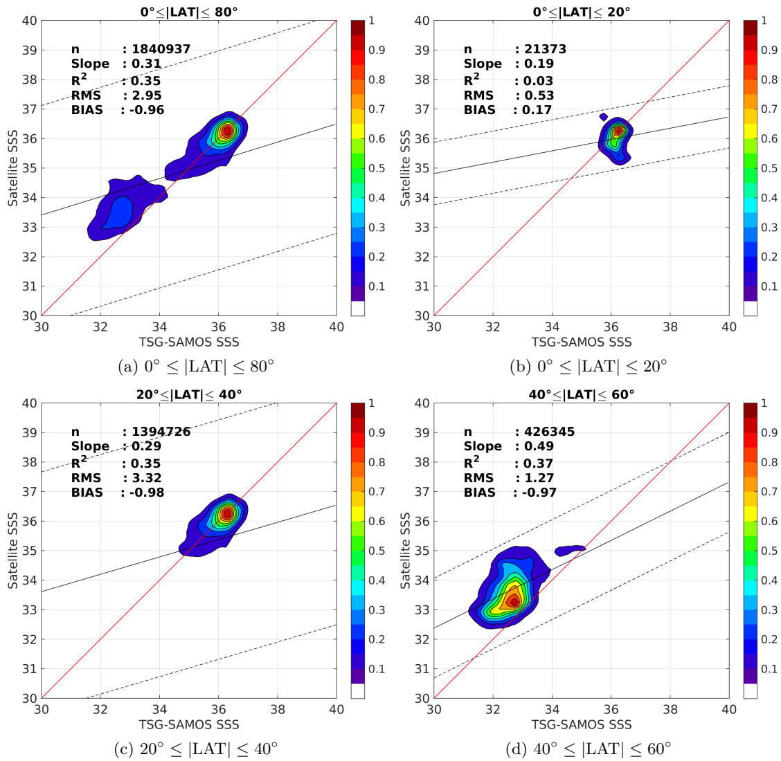
Figure 9: Contour maps of the concentration of SMAP-L3-JPL-V4-MONTHLY-60KM SSS (y-axis) versus TSG-SAMOS SSS (x-axis) at match-up pairs for different latitude bands. For each plot, the red line shows x=y . The black thin and dashed lines indicate a linear fit through the data cloud and the \pm 95\% confidence levels, respectively. The number match-up pairs n , the slope and R^2 coefficient of the linear fit, the root mean square (RMS) and the mean bias between satellite and in situ data are indicated for each latitude band in each plots.
