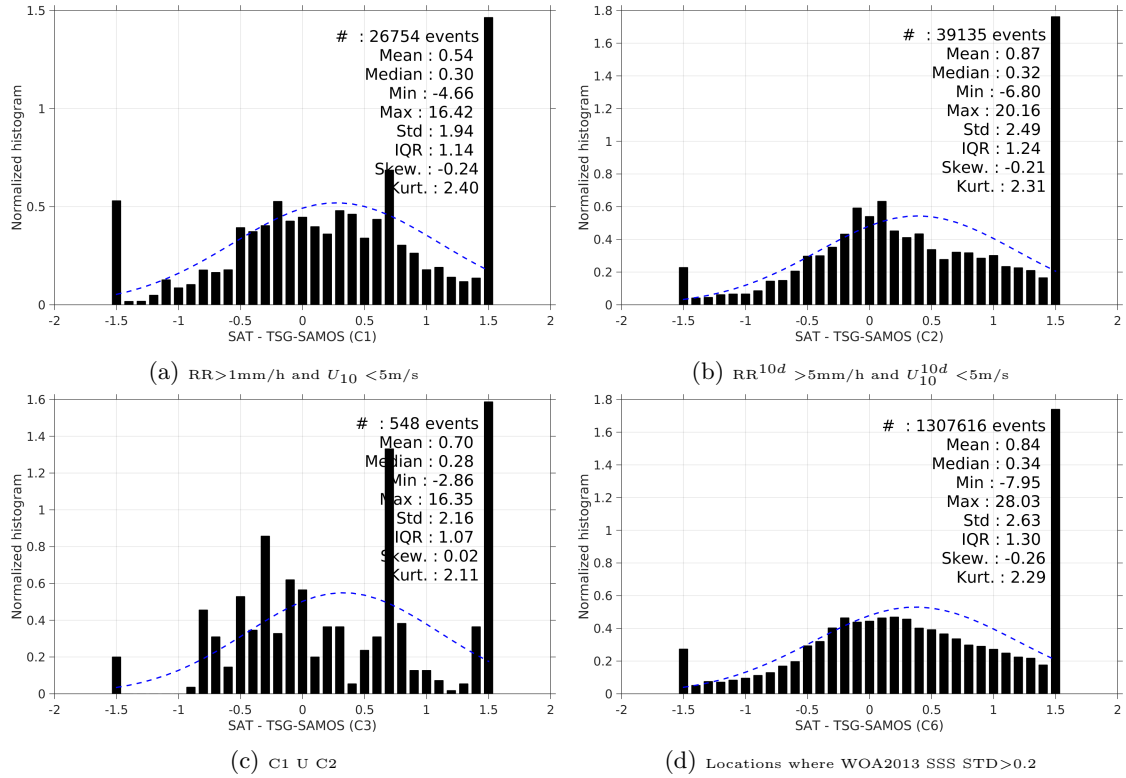
Figure 13: Normalized histogram of \Delta\text{SSS} (SMAP-L3-JPL-V4-MONTHLY-60KM - TSG-SAMOS) for 6 different subdatasets corresponding to: RR > 1mm/h and U_{10} < 5\text{m/s} (a), \text{RR}^{10d} > 5\text{mm/h} and U_{10}^{10d} < 5\text{m/s} (b), C1 U C2 (c), Locations where WOA2013 SSS STD > 0.2 (d).
