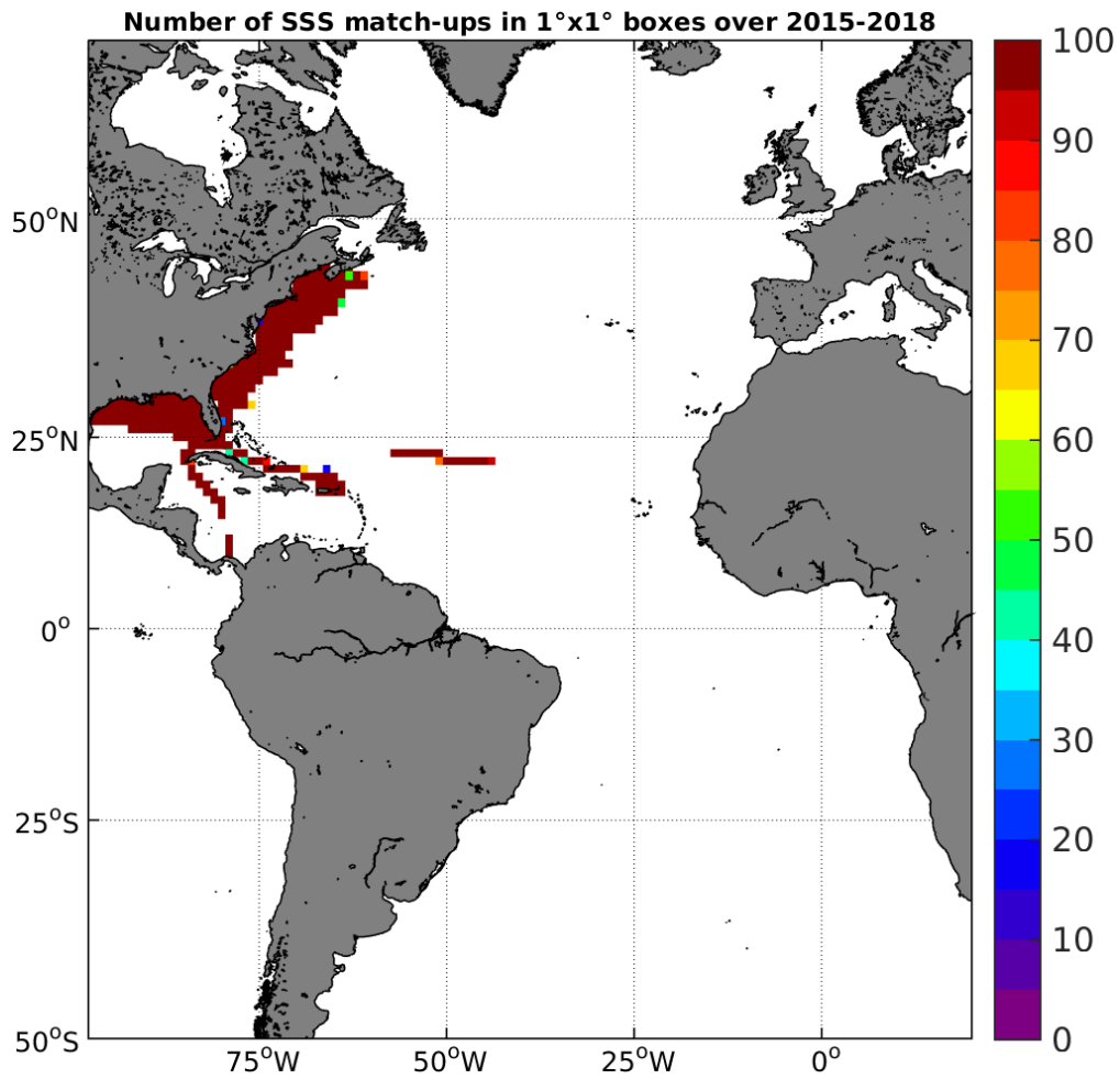
Figure 4: Number of SSS match-ups between TSG-SAMOS SSS and the SMAP-L3-JPL-V4-MONTHLY-60KM SSS product for the Atlantic Ocean Pi-MEP region over 1°x1° boxes and for the full satellite product period.
