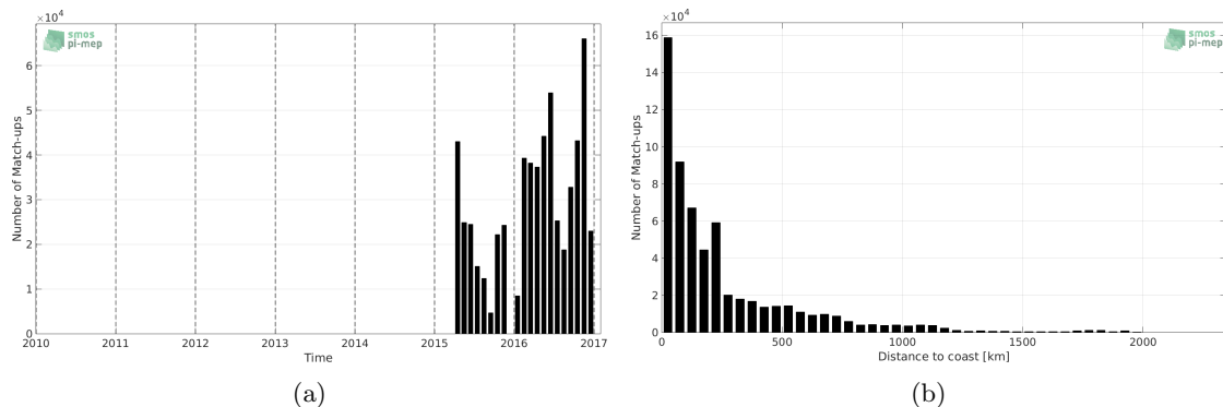
Figure 1: Number of match-ups between TSG-GOSUD-Research-vessel and SMAP-L3-JPL-V4-MONTHLY-60KM SSS as a function of time (a) and as function of the distance to coast (b) over the Atlantic Ocean Pi-MEP region and for the full satellite product period.
