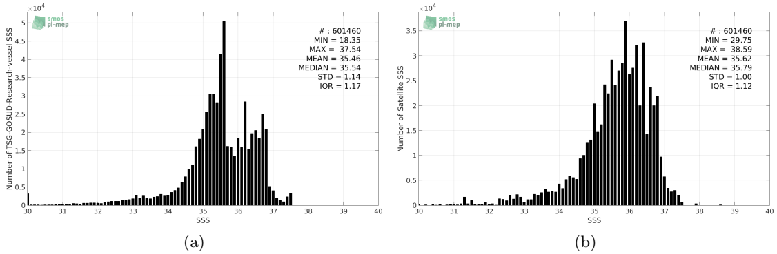
Figure 2: Histograms of SSS from TSG-GOSUD-Research-vessel (a) and SMAP-L3-JPL-V4-MONTHLY-60KM (b) considering all match-up pairs per bins of 0.1 over the Atlantic Ocean Pi-MEP region and for the full satellite product period.
