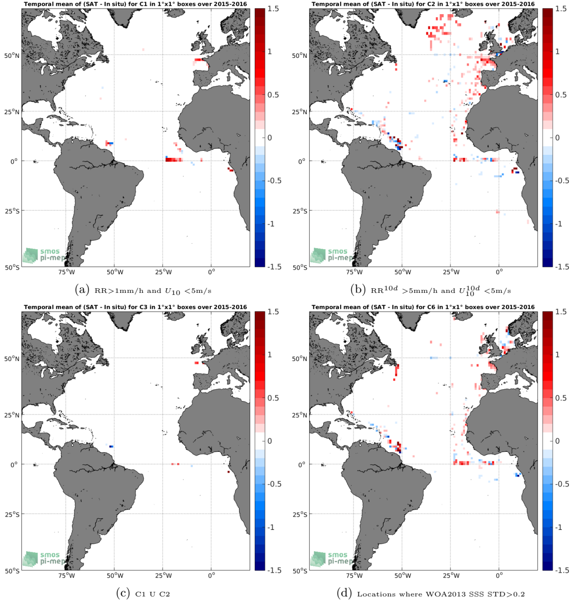
Figure 12: Temporal mean gridded over spatial boxes of size 1^\circ \times 1^\circ of \Delta SSS (SMAP-L3-JPL-V4-MONTHLY-60KM - TSG-GOSUD-Research-vessel) for 4 different subdatasets corresponding to: RR > 1\text{mm/h} and U_{10} < 5\text{m/s} (a), RR^{10d} > 5\text{mm/h} and U_{10}^{10d} < 5\text{m/s} (b), C1 U C2 (c), Locations where WOA2013 SSS STD > 0.2 (d).
