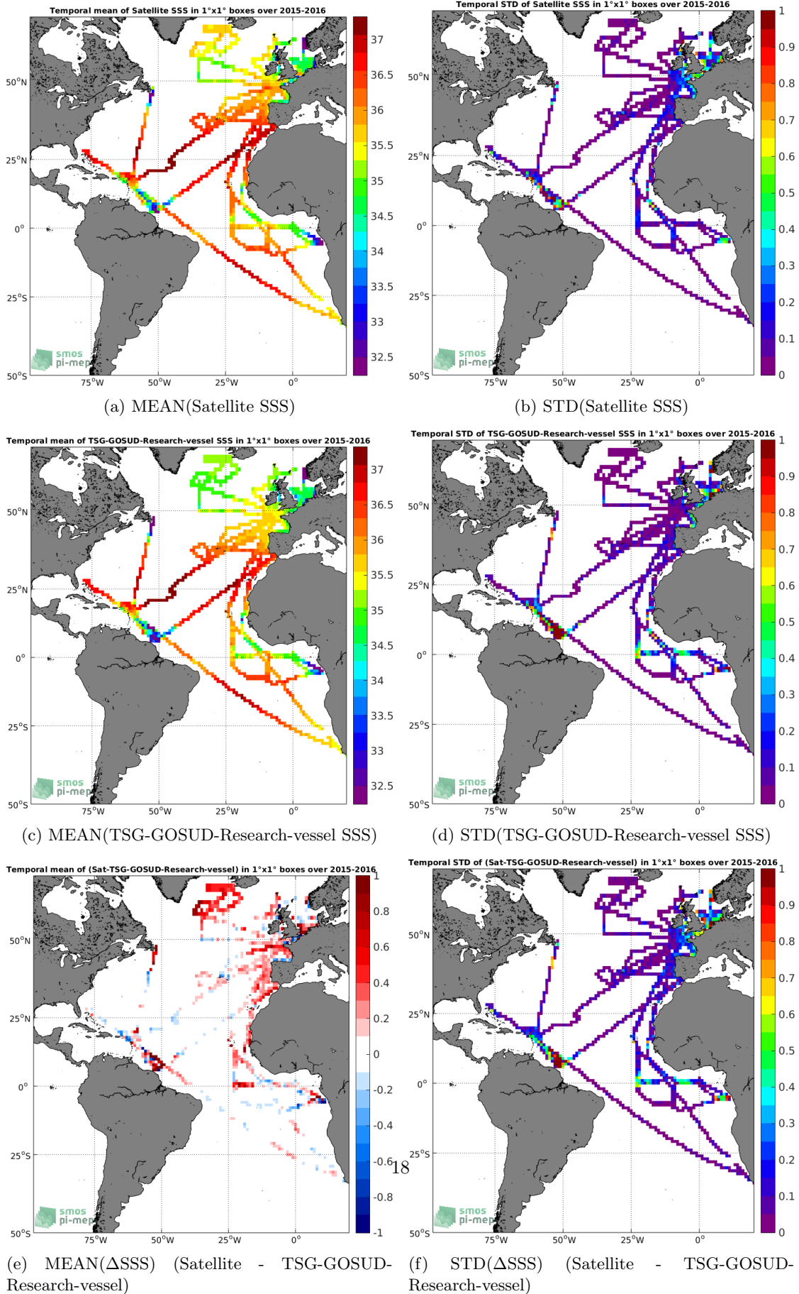
Figure 6: Temporal mean (left) and STD (right) of SSS from SMAP-L3-JPL-V4-MONTHLY-60KM (top), TSG-GOSUD-Research-vessel (middle), and of \Delta SSS (Satellite - TSG-GOSUD-Research-vessel). Only match-up pairs are used to generate these maps.
