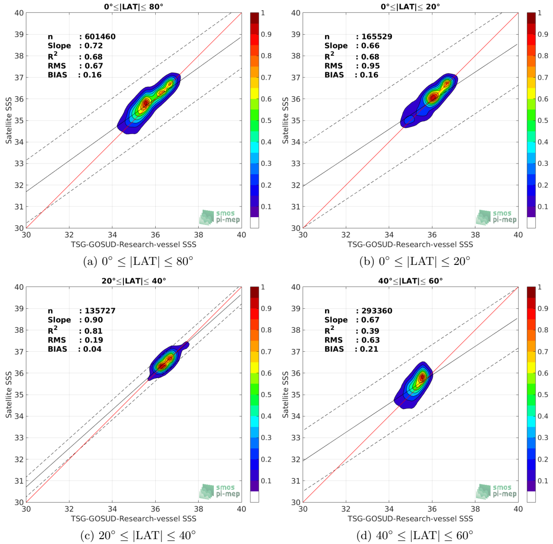
Figure 9: Contour maps of the concentration of SMAP-L3-JPL-V4-MONTHLY-60KM SSS (y-axis) versus TSG-GOSUD-Research-vessel SSS (x-axis) at match-up pairs for different latitude bands. For each plot, the red line shows x=y . The black thin and dashed lines indicate a linear fit through the data cloud and the \pm 95\% confidence levels, respectively. The number match-up pairs n , the slope and R^2 coefficient of the linear fit, the root mean square (RMS) and the mean bias between satellite and in situ data are indicated for each latitude band in each plots.
