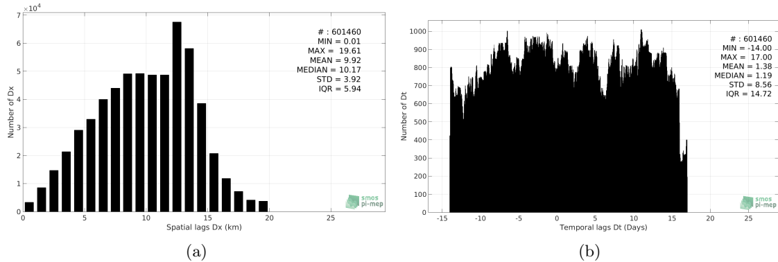
Figure 5: Histograms of the spatial (a) and temporal (b) lags between the time of the TSG-GOSUD-Research-vessel measurements and the date of the corresponding SMAP-L3-JPL-V4-MONTHLY-60KM SSS product.
