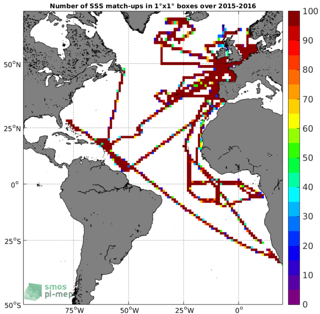
Figure 4: Number of SSS match-ups between TSG-GOSUD-Research-vessel SSS and the SMAP-L3-JPL-V4-MONTHLY-60KM SSS product for the Atlantic Ocean Pi-MEP region over 1°x1° boxes and for the full satellite product period.
