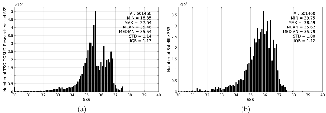
Figure 2: Histograms of SSS from TSG-GOSUD-Research-vessel (a) and SMAP-L3-JPL-V4-MONTHLY-60KM (b) considering all match-up pairs per bins of 0.1 over the Atlantic Ocean Pi-MEP region and for the full satellite product period.
