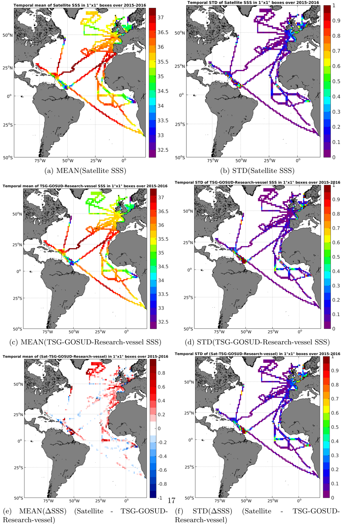
Figure 6: Temporal mean (left) and STD (right) of SSS from SMAP-L3-JPL-V4-MONTHLY-60KM (top), TSG-GOSUD-Research-vessel (middle), and of \Delta SSS (Satellite - TSG-GOSUD-Research-vessel). Only match-up pairs are used to generate these maps.
