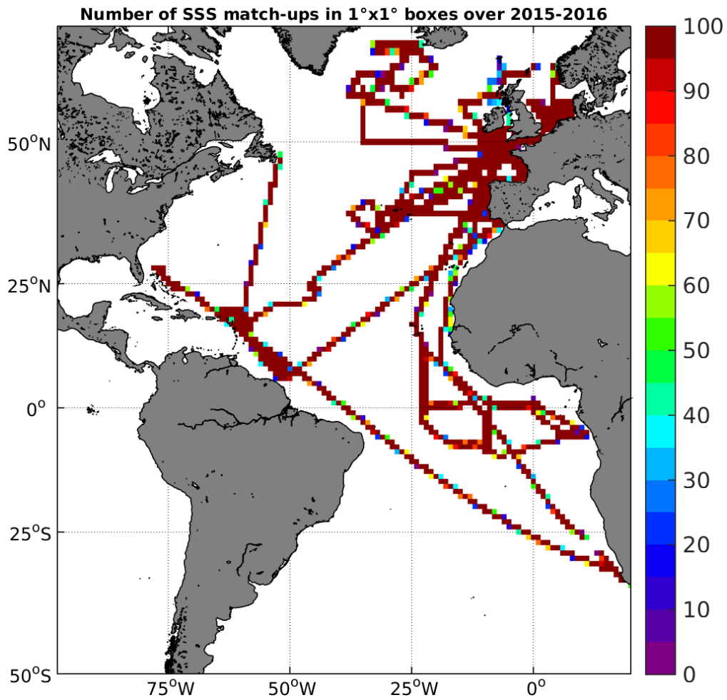
Figure 4: Number of SSS match-ups between TSG-GOSUD-Research-vessel SSS and the SMAP-L3-JPL-V4-MONTHLY-60KM SSS product for the Atlantic Ocean Pi-MEP region over 1°x1° boxes and for the full satellite product period.
