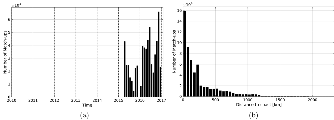
Figure 1: Number of match-ups between TSG-GOSUD-Research-vessel and SMAP-L3-JPL-V4-MONTHLY-60KM SSS as a function of time (a) and as function of the distance to coast (b) over the Atlantic Ocean Pi-MEP region and for the full satellite product period.
