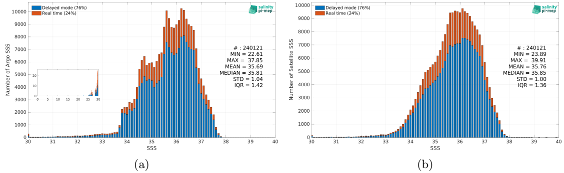
Figure 2: Histograms of SSS from Argo (a) and SMAP SSS L2-AVERAGED v5 (RSS) (b) considering all match-up pairs per bins of 0.1 over the Atlantic Ocean Pi-MEP region and for the full satellite product period.
