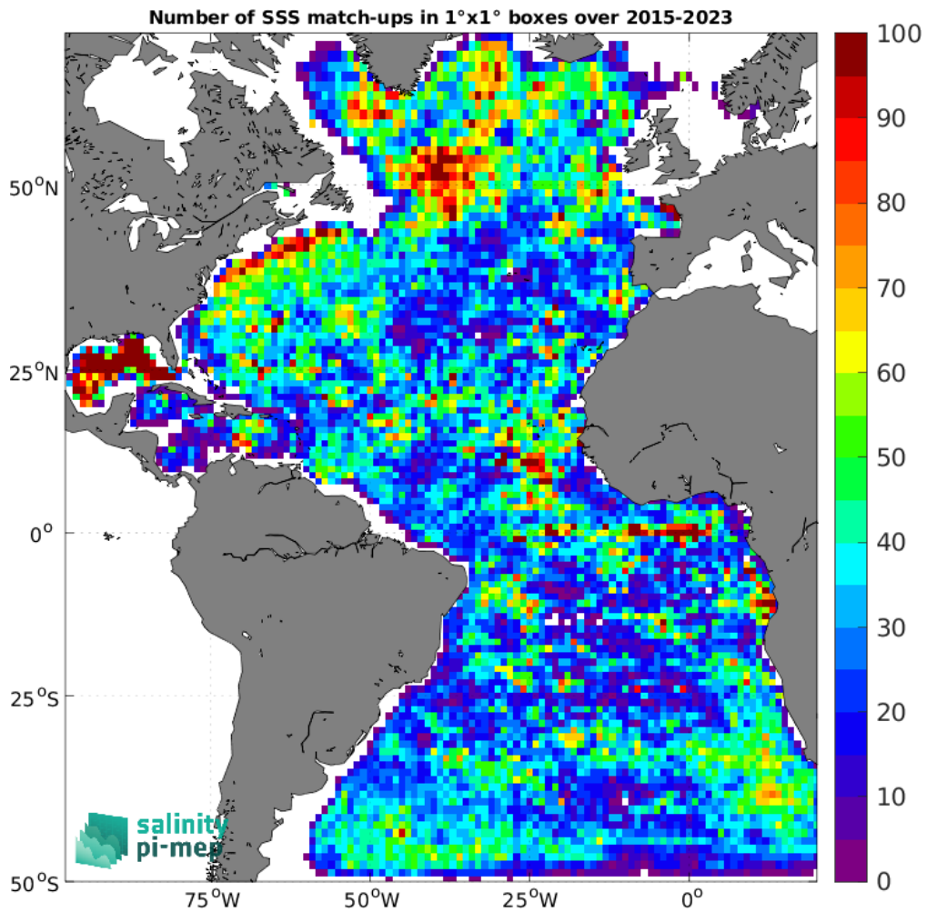
Figure 4: Number of SSS match-ups between Argo SSS and the SMAP SSS L2-AVERAGED v5 (RSS) SSS product for the Atlantic Ocean Pi-MEP region over 1^\circ \times 1^\circ boxes and for the full satellite product period.
