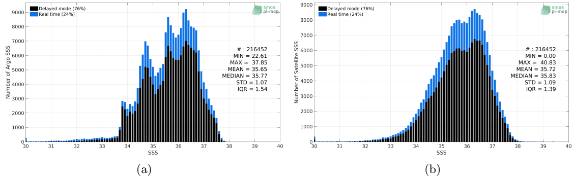
Figure 2: Histograms of SSS from Argo (a) and SMAP SSS L2-AVERAGED v5.0 (JPL) (b) considering all match-up pairs per bins of 0.1 over the Atlantic Ocean Pi-MEP region and for the full satellite product period.
