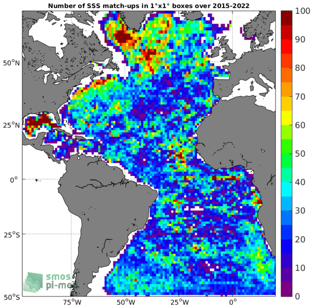
Figure 4: Number of SSS match-ups between Argo SSS and the SMAP SSS L2-AVERAGED v5.0 (JPL) SSS product for the Atlantic Ocean Pi-MEP region over 1°×1° boxes and for the full satellite product period.
