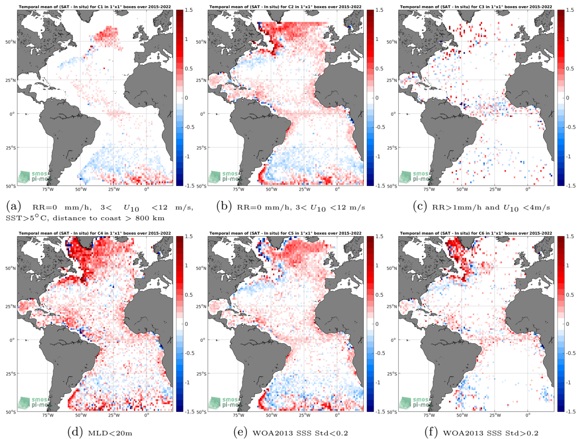
Figure 12: Temporal mean gridded over spatial boxes of size 1^\circ \times 1^\circ of \Delta SSS (SMAP SSS L2-AVERAGED v5.0 (JPL) - Argo) for 6 different subdatasets corresponding to:RR=0 mm/h, 3 < U_{10} < 12 m/s, SST > 5^\circ\text{C} , distance to coast > 800 km (a), RR=0 mm/h, 3 < U_{10} < 12 m/s (b), RR > 1 mm/h and U_{10} < 4 m/s (c),MLD < 20 m (d),WOA2013 SSS Std < 0.2 (e),WOA2013 SSS Std > 0.2 (f).
