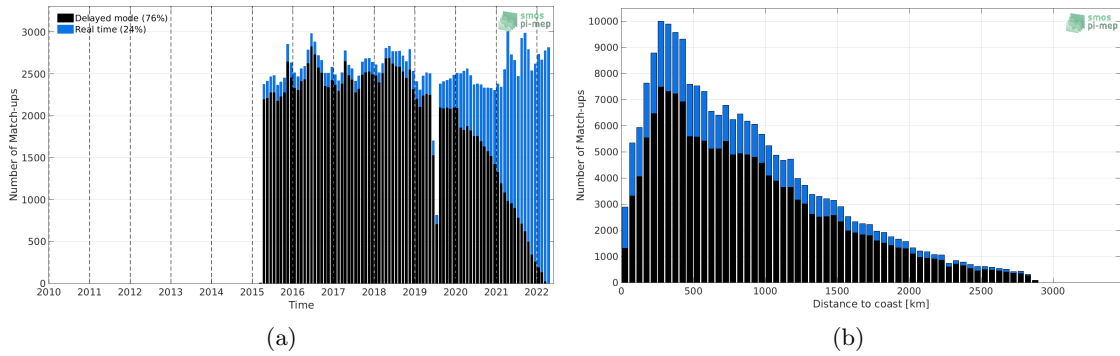
Figure 1: Number of match-ups between Argo and SMAP SSS L2-AVERAGED v5.0 (JPL) SSS as a function of time (a) and as function of the distance to coast (b) over the Atlantic Ocean Pi-MEP region and for the full satellite product period.
