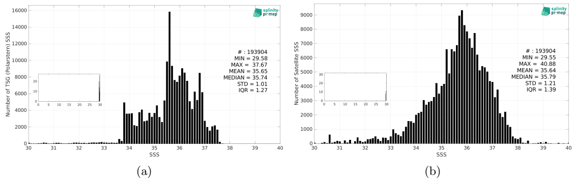
Figure 3: Histograms of SSS from TSG (Polarstern) (a) and SMAP SSS L2 v6 (RSS) (b) considering all match-up pairs per bins of 0.1 over the Atlantic Ocean Pi-MEP region and for the full satellite product period.
