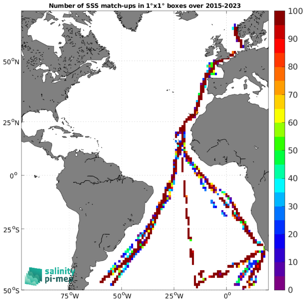
Figure 5: Number of SSS match-ups between TSG (Polarstern) SSS and the SMAP SSS L2 v6 (RSS) SSS product for the Atlantic Ocean Pi-MEP region over 1°×1° boxes and for the full satellite product period.
