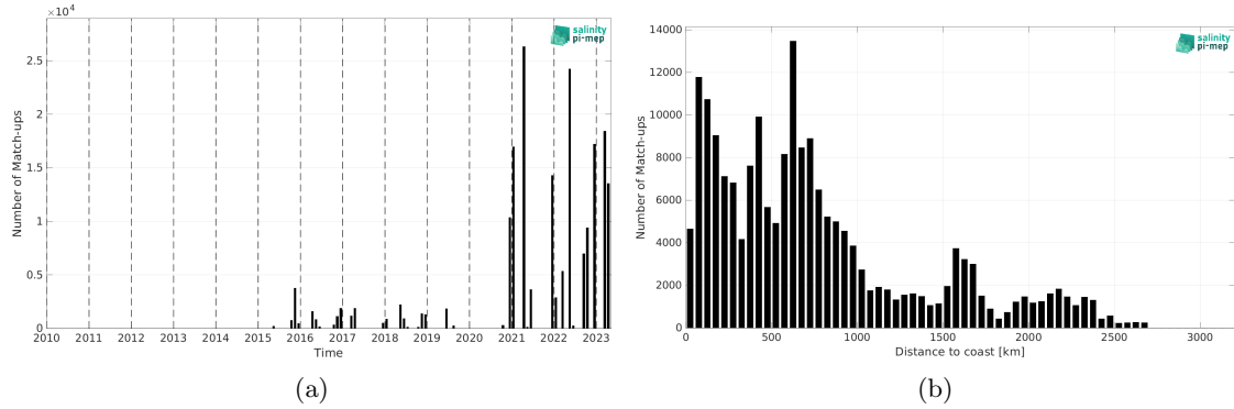
Figure 2: Number of match-ups between TSG (Polarstern) and SMAP SSS L2 v6 (RSS) SSS as a function of time (a) and as function of the distance to coast (b) over the Atlantic Ocean Pi-MEP region and for the full satellite product period.
