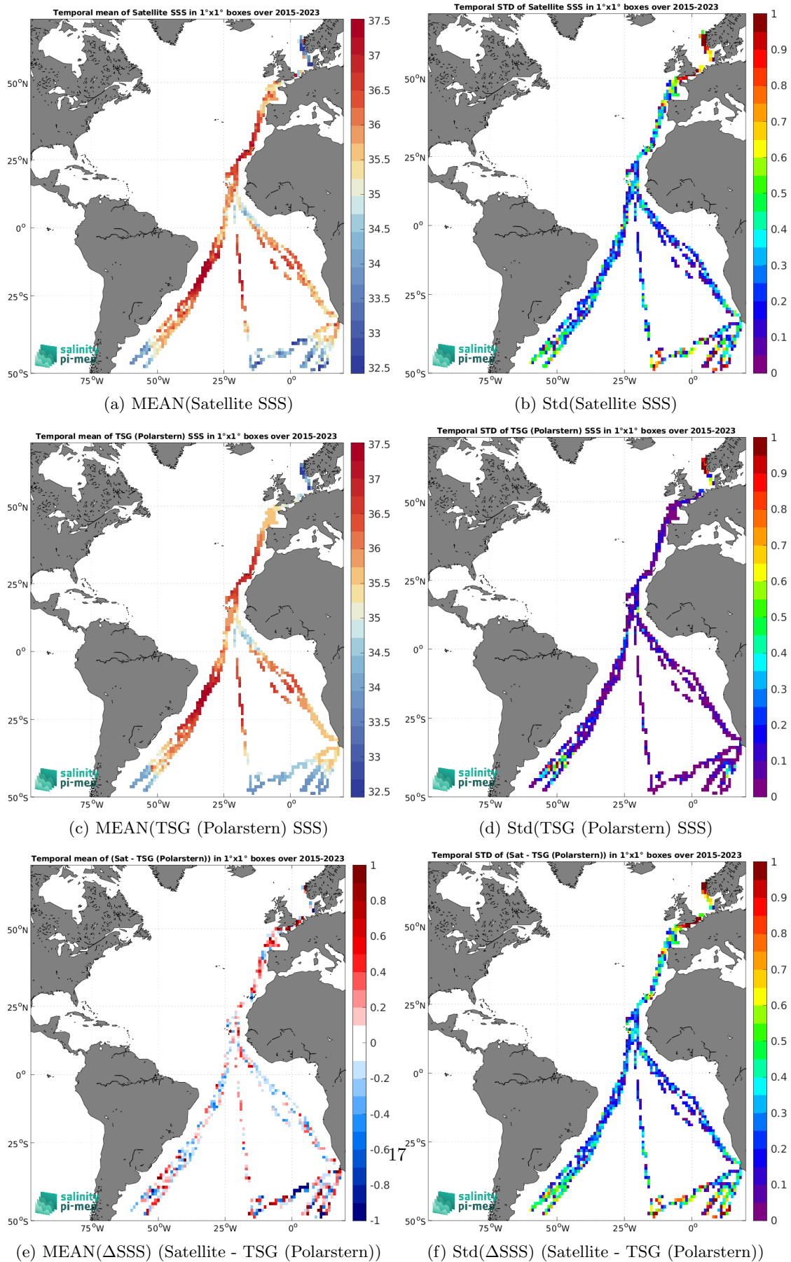
Figure 7: Temporal mean (left) and Std (right) of SSS from SMAP SSS L2 v6 (RSS) (top), TSG (Polarstern) (middle), and of \Delta SSS (Satellite - TSG (Polarstern)). Only match-up pairs are used to generate these maps.
