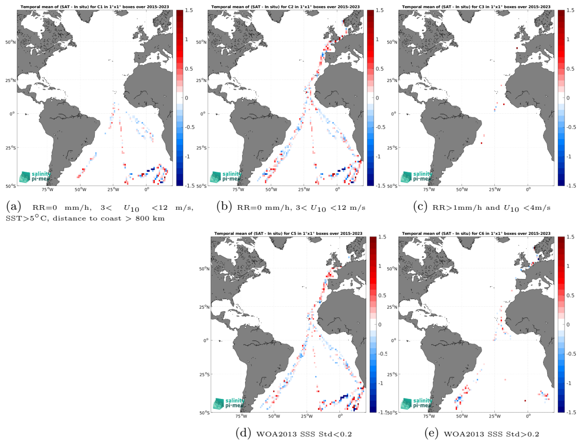
Figure 14: Temporal mean gridded over spatial boxes of size 1^\circ \times 1^\circ of \Delta\text{SSS} (SMAP SSS L2 v6 (RSS) - TSG (Polarstern)) for 5 different subdatasets corresponding to:RR=0 mm/h, 3 < U_{10} < 12 m/s, SST >5^\circ\text{C} , distance to coast > 800 km (a), RR=0 mm/h, 3 < U_{10} < 12 m/s (b), RR >1 mm/h and U_{10} < 4 m/s (c), WOA2013 SSS Std <0.2 (d), WOA2013 SSS Std >0.2 (e).
