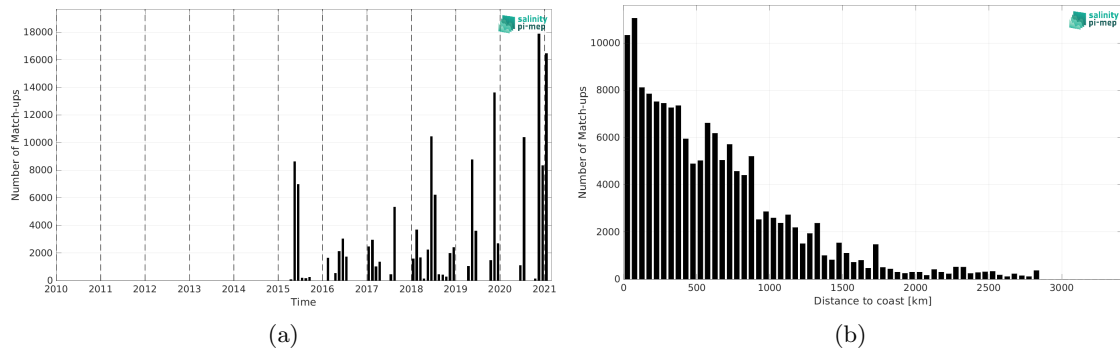
Figure 2: Number of match-ups between TSG (GOSUD-Sailing-ship) and SMAP SSS L2 v6 (RSS) SSS as a function of time (a) and as function of the distance to coast (b) over the Atlantic Ocean Pi-MEP region and for the full satellite product period.
