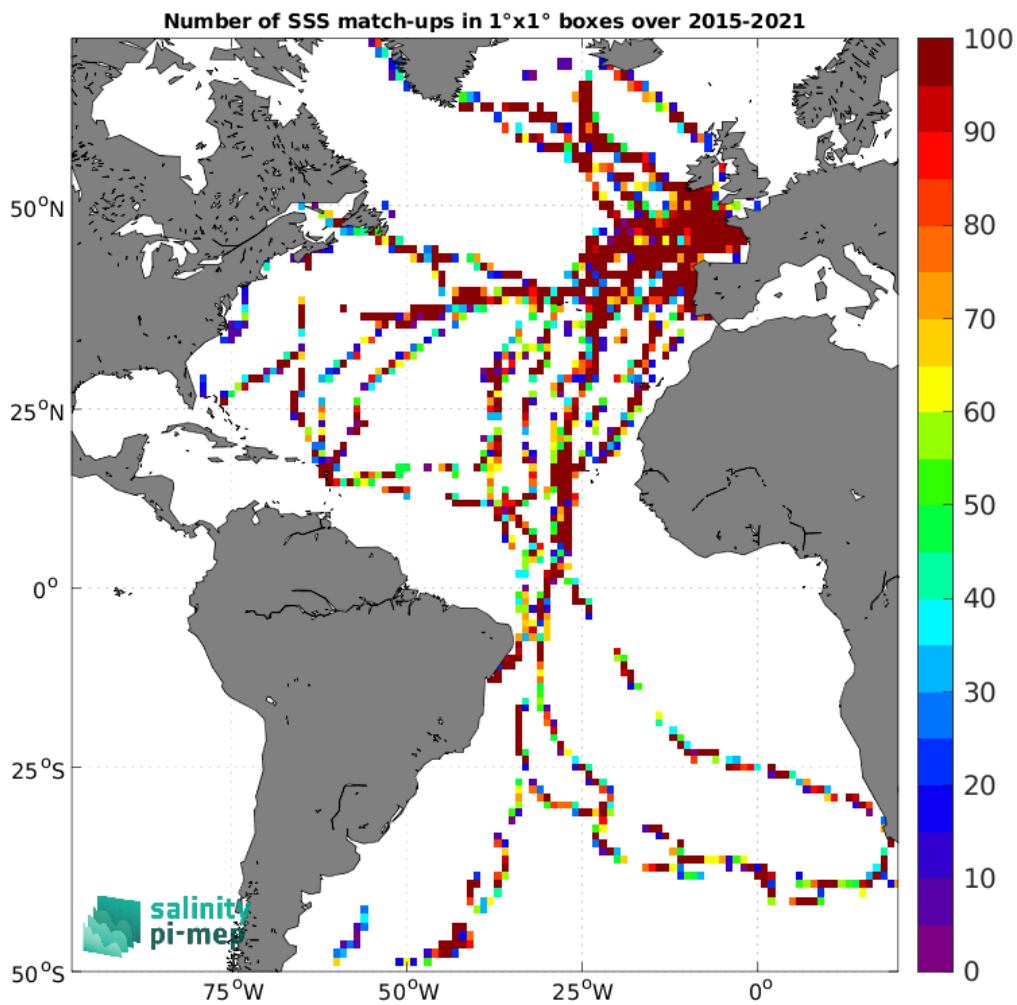
Figure 5: Number of SSS match-ups between TSG (GOSUD-Sailing-ship) SSS and the SMAP SSS L2 v6 (RSS) SSS product for the Atlantic Ocean Pi-MEP region over 1°x1° boxes and for the full satellite product period.
