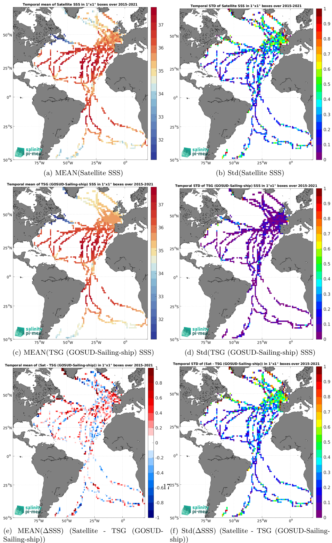
Figure 7: Temporal mean (left) and Std (right) of SSS from SMAP SSS L2 v6 (RSS) (top), TSG (GOSUD-Sailing-ship) (middle), and of \Delta SSS (Satellite - TSG (GOSUD-Sailing-ship)). Only match-up pairs are used to generate these maps.
