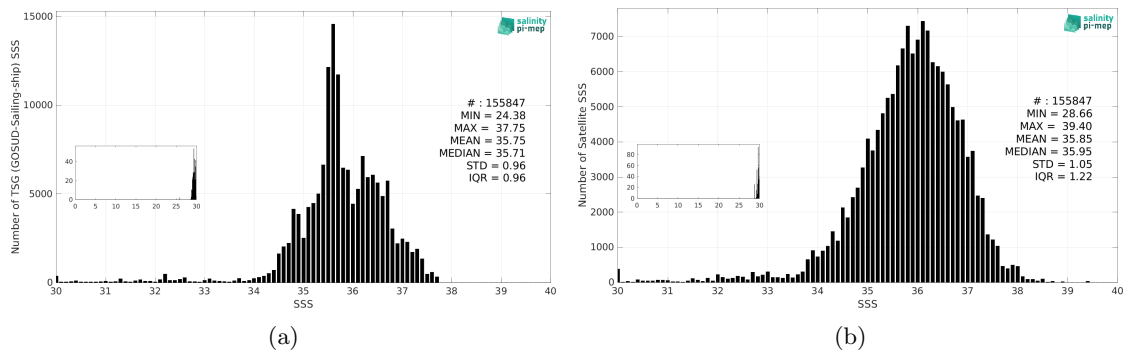
Figure 3: Histograms of SSS from TSG (GOSUD-Sailing-ship) (a) and SMAP SSS L2 v6 (RSS) (b) considering all match-up pairs per bins of 0.1 over the Atlantic Ocean Pi-MEP region and for the full satellite product period.
