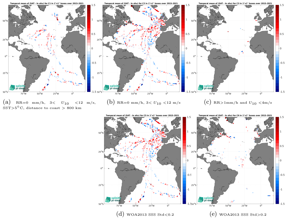
Figure 14: Temporal mean gridded over spatial boxes of size 1^\circ \times 1^\circ of \Delta\text{SSS} (SMAP SSS L2 v6 (RSS) - TSG (GOSUD-Sailing-ship)) for 5 different subdatasets corresponding to:RR=0 mm/h, 3 < U_{10} < 12 m/s, SST>5°C, distance to coast > 800 km (a), RR=0 mm/h, 3 < U_{10} < 12 m/s (b), RR>1mm/h and U_{10} < 4 m/s (c), WOA2013 SSS Std<0.2 (d), WOA2013 SSS Std>0.2 (e).
