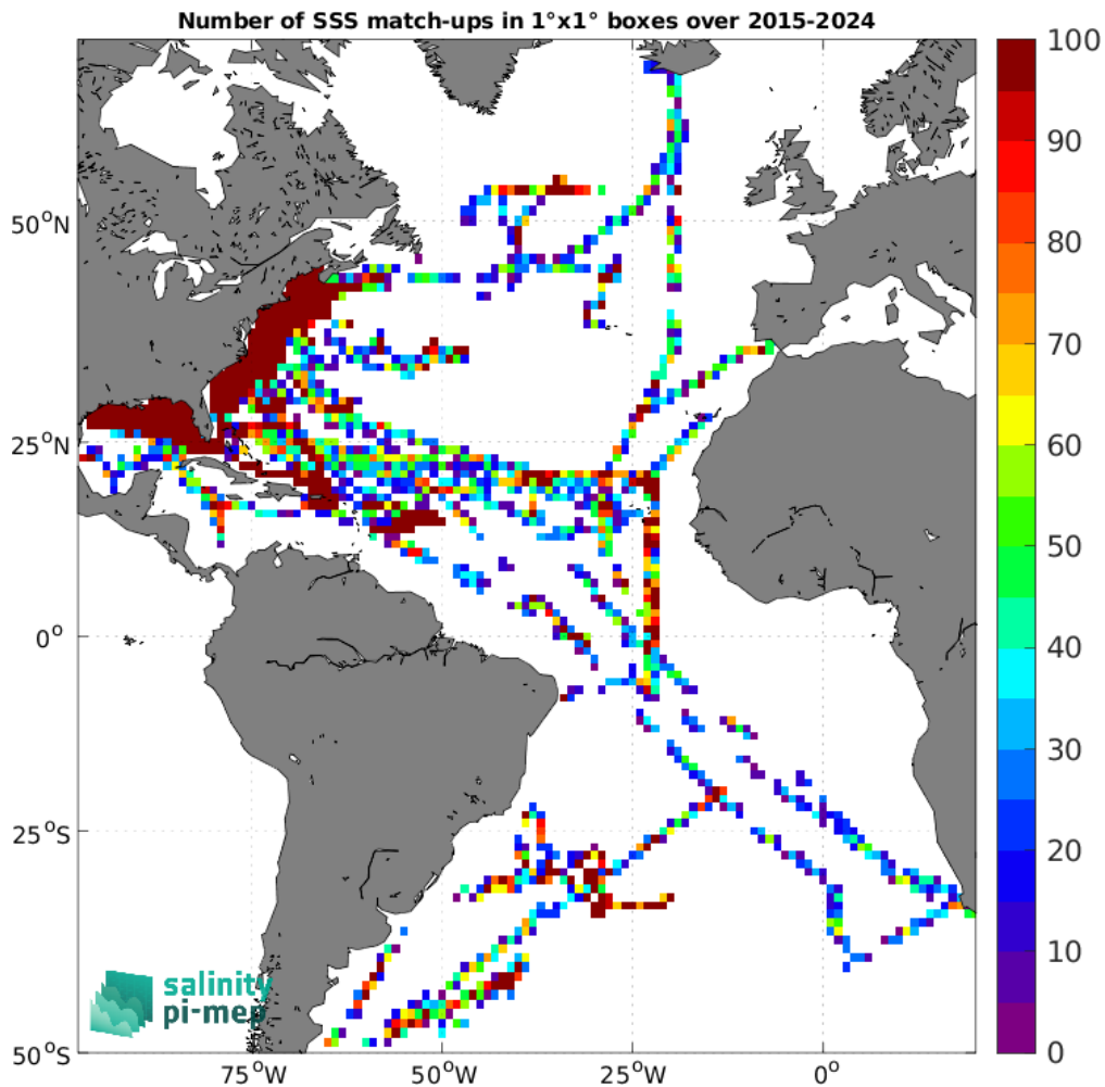
Figure 5: Number of SSS match-ups between TSG (SAMOS) SSS and the SMAP SSS L2 v6 - 40 km (RSS) SSS product for the Atlantic Ocean Pi-MEP region over 1^\circ \times 1^\circ boxes and for the full satellite product period.
