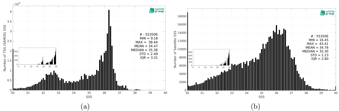
Figure 3: Histograms of SSS from TSG (SAMOS) (a) and SMAP SSS L2 v6 - 40 km (RSS) (b) considering all match-up pairs per bins of 0.1 over the Atlantic Ocean Pi-MEP region and for the full satellite product period.
