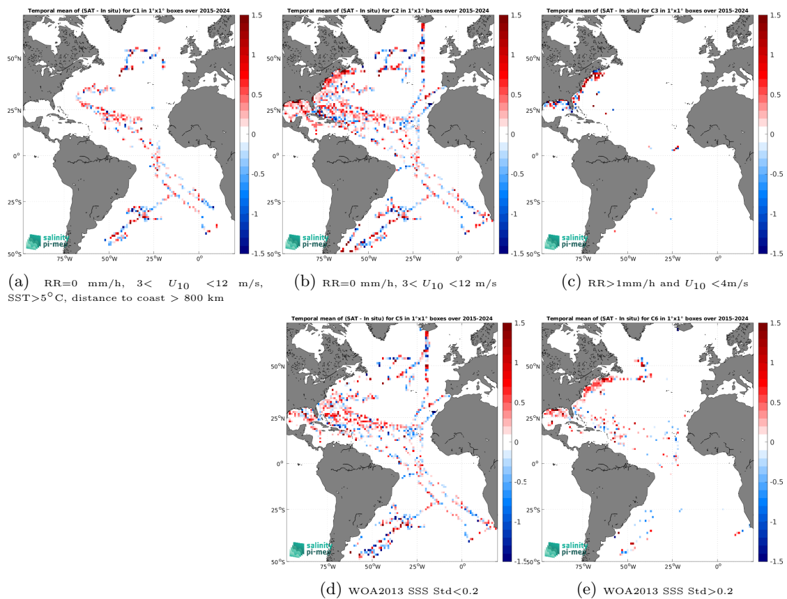
Figure 14: Temporal mean gridded over spatial boxes of size 1^\circ \times 1^\circ of \Delta\text{SSS} (SMAP SSS L2 v6 - 40 km (RSS) - TSG (SAMOS)) for 5 different subdatasets corresponding to:RR=0 mm/h, 3 < U_{10} < 12 m/s, SST>5°C, distance to coast > 800 km (a), RR=0 mm/h, 3 < U_{10} < 12 m/s (b), RR>1mm/h and U_{10} < 4 m/s (c), WOA2013 SSS Std<0.2 (d), WOA2013 SSS Std>0.2 (e).
