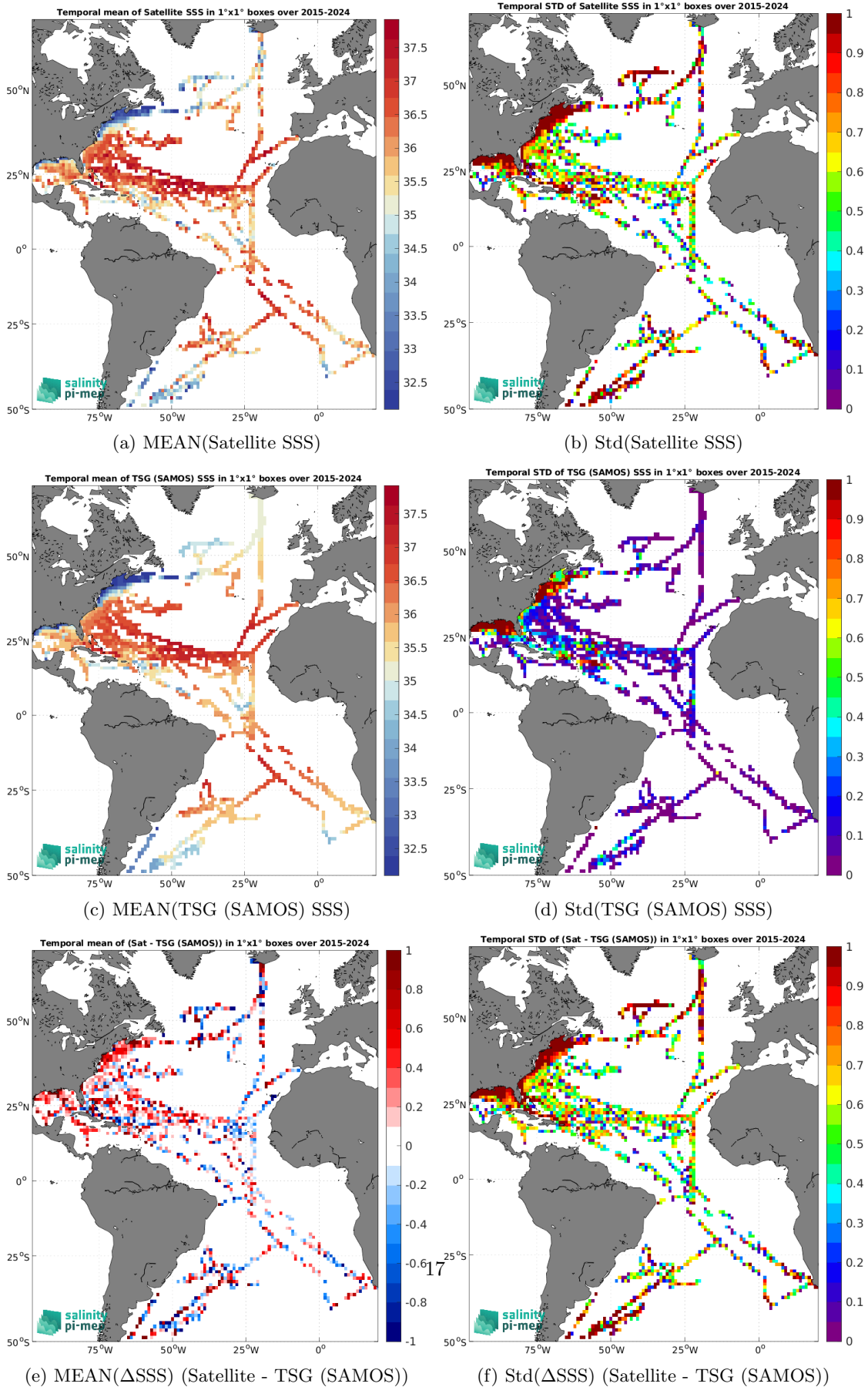
Figure 7: Temporal mean (left) and Std (right) of SSS from SMAP SSS L2 v6 - 40 km (RSS) (top), TSG (SAMOS) (middle), and of \Delta SSS (Satellite - TSG (SAMOS)). Only match-up pairs are used to generate these maps.
