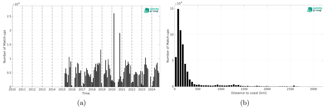
Figure 2: Number of match-ups between TSG (SAMOS) and SMAP SSS L2 v6 - 40 km (RSS) SSS as a function of time (a) and as function of the distance to coast (b) over the Atlantic Ocean Pi-MEP region and for the full satellite product period.
