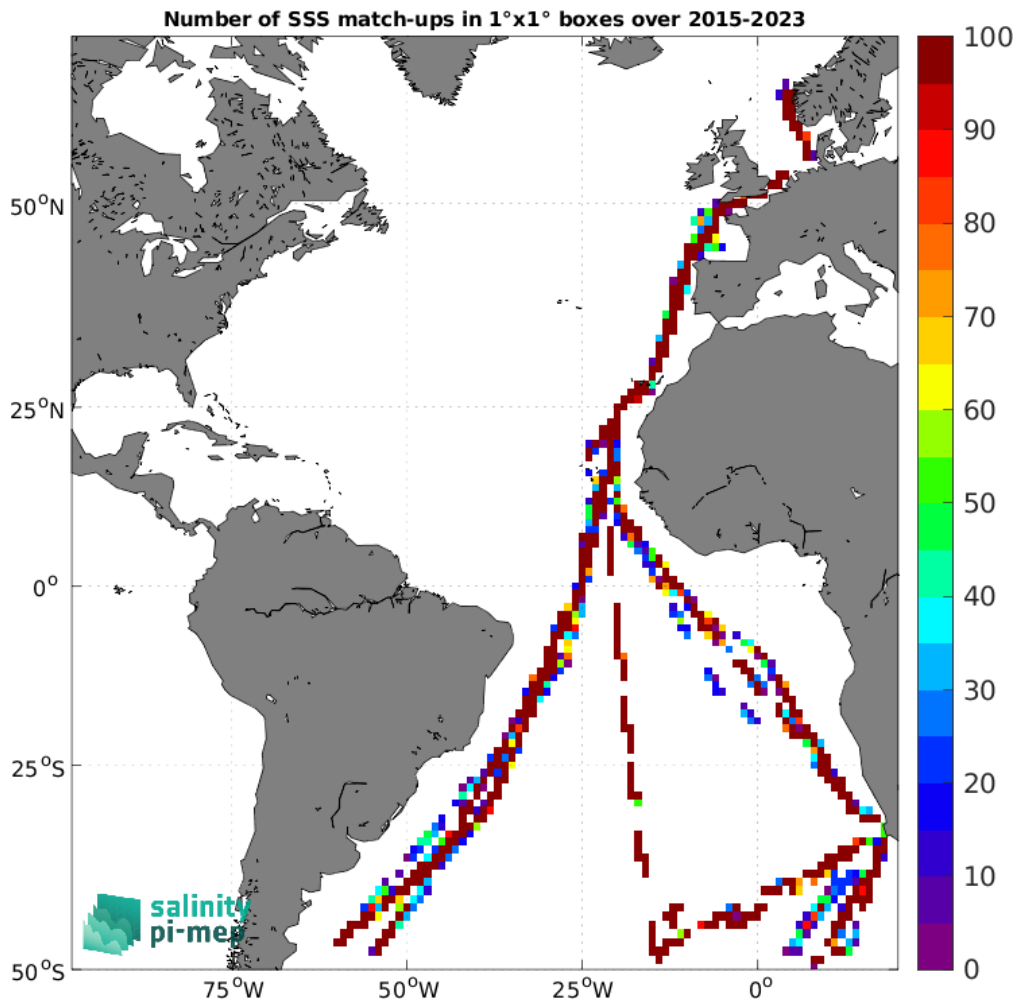
Figure 5: Number of SSS match-ups between TSG (Polarstern) SSS and the SMAP SSS L2 v6 - 40 km (RSS) SSS product for the Atlantic Ocean Pi-MEP region over 1^\circ \times 1^\circ boxes and for the full satellite product period.
