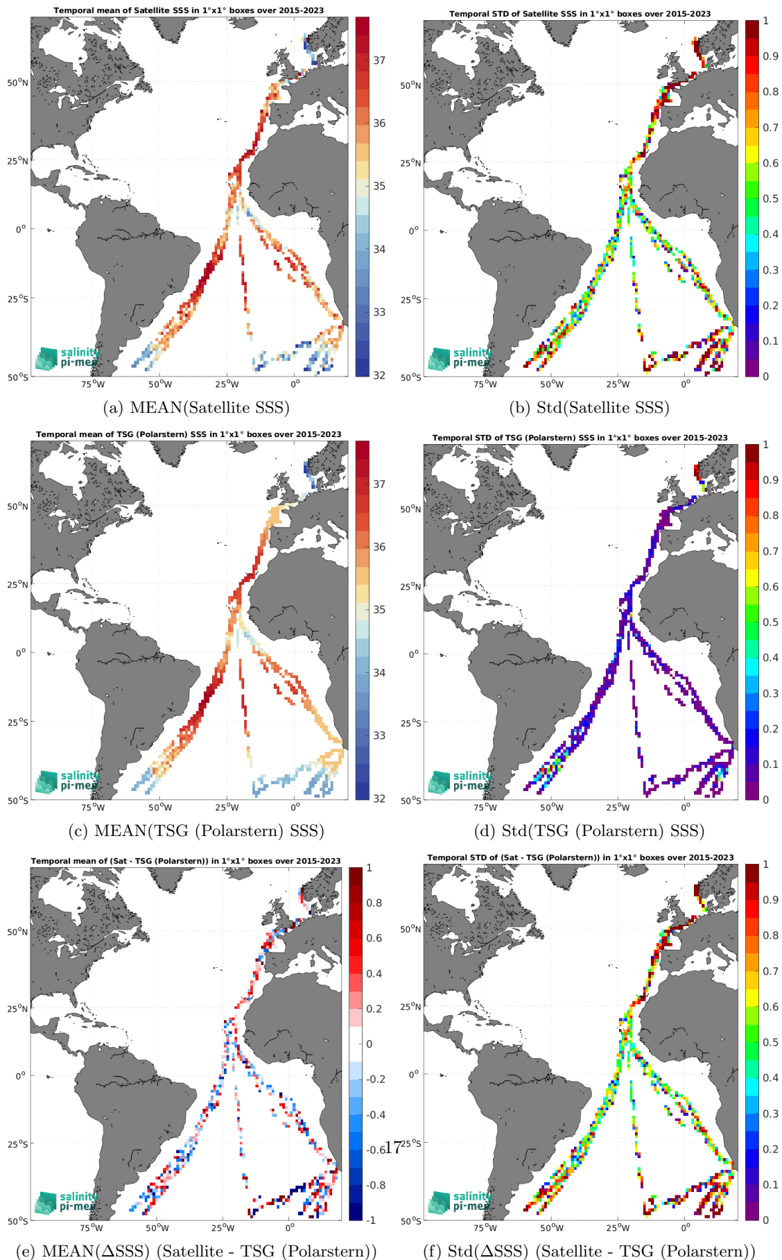
Figure 7: Temporal mean (left) and Std (right) of SSS from SMAP SSS L2 v6 - 40 km (RSS) (top), TSG (Polarstern) (middle), and of \Delta SSS (Satellite - TSG (Polarstern)). Only match-up pairs are used to generate these maps.
