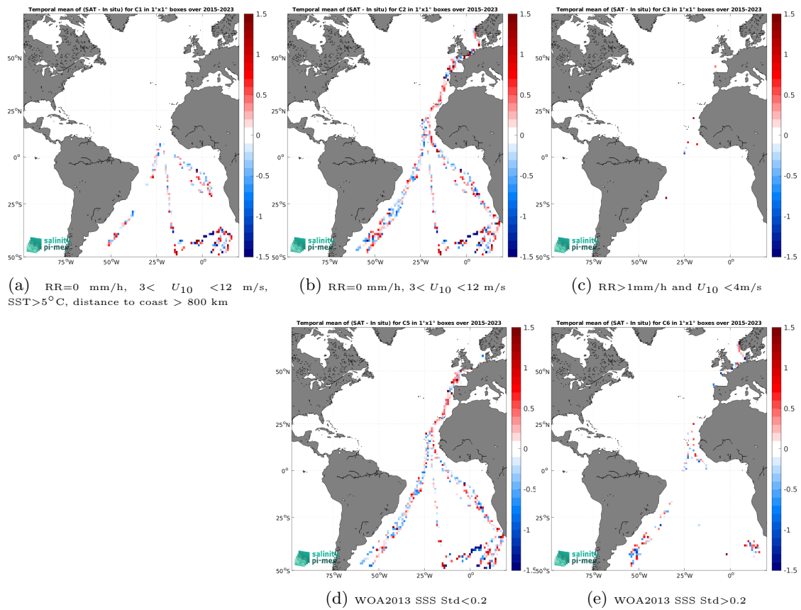
Figure 14: Temporal mean gridded over spatial boxes of size 1^\circ \times 1^\circ of \Delta\text{SSS} (SMAP SSS L2 v6 - 40 km (RSS) - TSG (Polarstern)) for 5 different subdatasets corresponding to:RR=0 mm/h, 3 < U_{10} < 12 m/s, SST>5°C, distance to coast > 800 km (a), RR=0 mm/h, 3 < U_{10} < 12 m/s (b), RR>1mm/h and U_{10} < 4 m/s (c), WOA2013 SSS Std<0.2 (d), WOA2013 SSS Std>0.2 (e).
