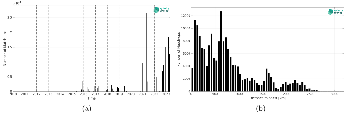
Figure 2: Number of match-ups between TSG (Polarstern) and SMAP SSS L2 v6 - 40 km (RSS) SSS as a function of time (a) and as function of the distance to coast (b) over the Atlantic Ocean Pi-MEP region and for the full satellite product period.
