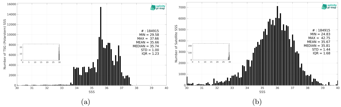
Figure 3: Histograms of SSS from TSG (Polarstern) (a) and SMAP SSS L2 v6 - 40 km (RSS) (b) considering all match-up pairs per bins of 0.1 over the Atlantic Ocean Pi-MEP region and for the full satellite product period.
