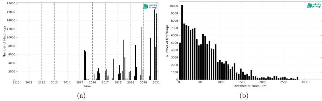
Figure 2: Number of match-ups between TSG (GOSUD-Sailing-ship) and SMAP SSS L2 v6 - 40 km (RSS) SSS as a function of time (a) and as function of the distance to coast (b) over the Atlantic Ocean Pi-MEP region and for the full satellite product period.
