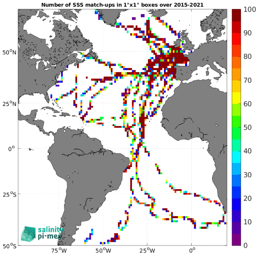
Figure 5: Number of SSS match-ups between TSG (GOSUD-Sailing-ship) SSS and the SMAP SSS L2 v6 - 40 km (RSS) SSS product for the Atlantic Ocean Pi-MEP region over 1°×1° boxes and for the full satellite product period.
