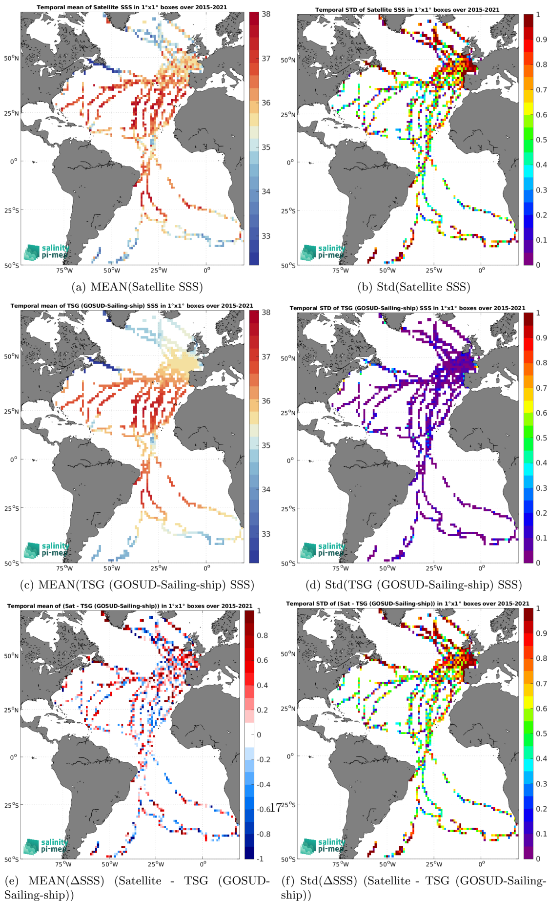
Figure 7: Temporal mean (left) and Std (right) of SSS from SMAP SSS L2 v6 - 40 km (RSS) (top), TSG (GOSUD-Sailing-ship) (middle), and of \Delta SSS (Satellite - TSG (GOSUD-Sailing-ship)). Only match-up pairs are used to generate these maps.
