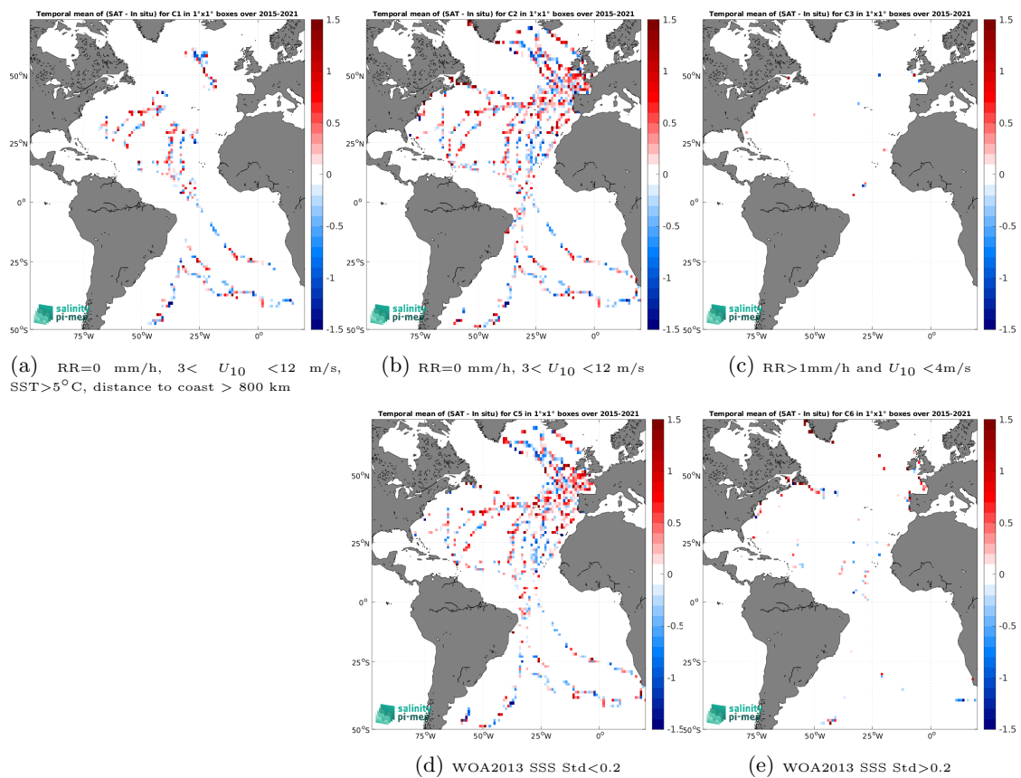
Figure 14: Temporal mean gridded over spatial boxes of size 1^\circ \times 1^\circ of \Delta SSS (SMAP SSS L2 v6 - 40 km (RSS) - TSG (GOSUD-Sailing-ship)) for 5 different subdatasets corresponding to:RR=0 mm/h, 3 < U_{10} < 12 m/s, SST >5^\circ\text{C} , distance to coast > 800 km (a), RR=0 mm/h, 3 < U_{10} < 12 m/s (b), RR >1 mm/h and U_{10} < 4 m/s (c), WOA2013 SSS Std <0.2 (d), WOA2013 SSS Std >0.2 (e).
