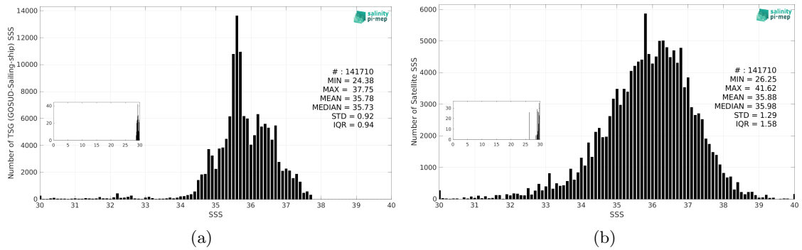
Figure 3: Histograms of SSS from TSG (GOSUD-Sailing-ship) (a) and SMAP SSS L2 v6 - 40 km (RSS) (b) considering all match-up pairs per bins of 0.1 over the Atlantic Ocean Pi-MEP region and for the full satellite product period.
