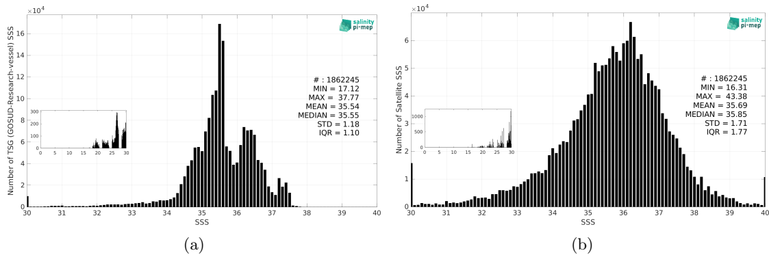
Figure 3: Histograms of SSS from TSG (GOSUD-Research-vessel) (a) and SMAP SSS L2 v6 - 40 km (RSS) (b) considering all match-up pairs per bins of 0.1 over the Atlantic Ocean Pi-MEP region and for the full satellite product period.
