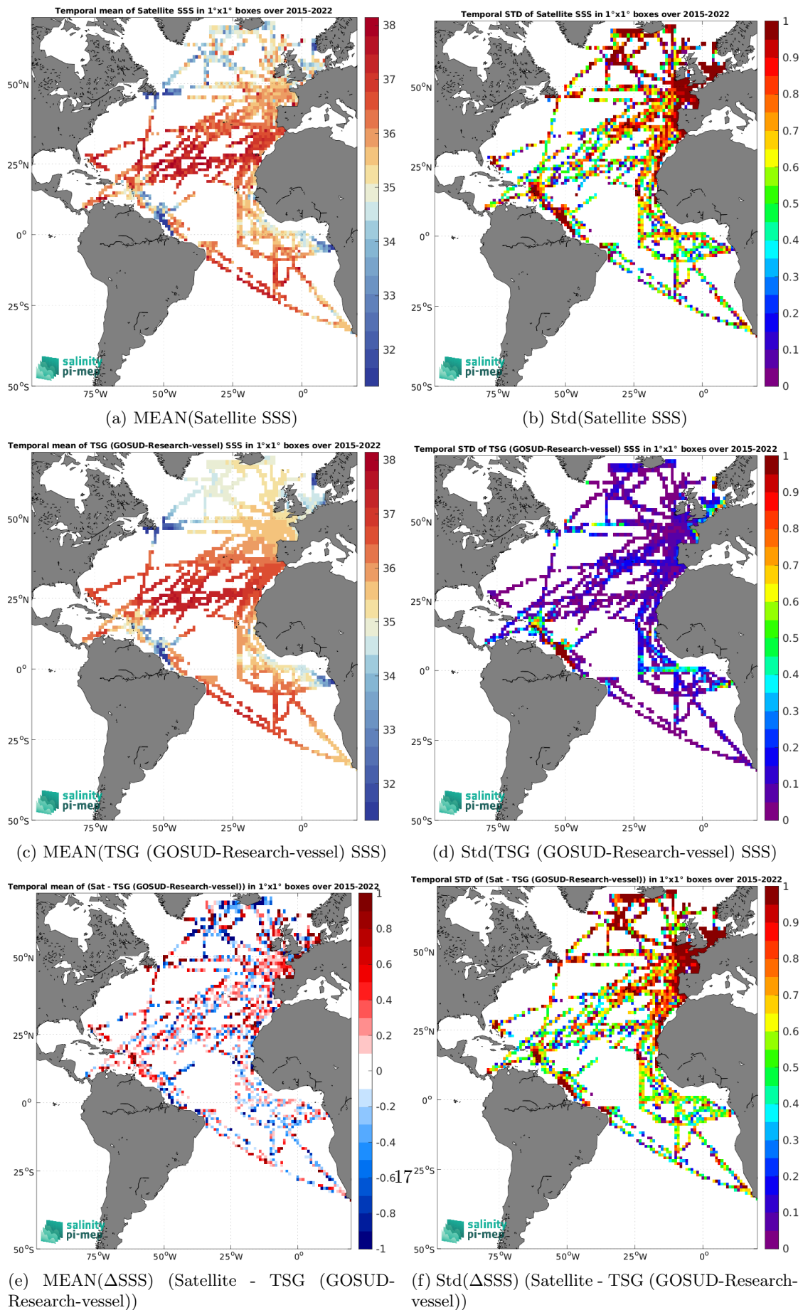
Figure 7: Temporal mean (left) and Std (right) of SSS from SMAP SSS L2 v6 - 40 km (RSS) (top), TSG (GOSUD-Research-vessel) (middle), and of \Delta SSS (Satellite - TSG (GOSUD-Research-vessel)). Only match-up pairs are used to generate these maps.
