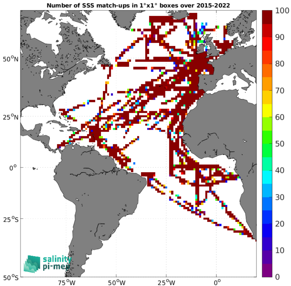
Figure 5: Number of SSS match-ups between TSG (GOSUD-Research-vessel) SSS and the SMAP SSS L2 v6 - 40 km (RSS) SSS product for the Atlantic Ocean Pi-MEP region over 1^\circ \times 1^\circ boxes and for the full satellite product period.
