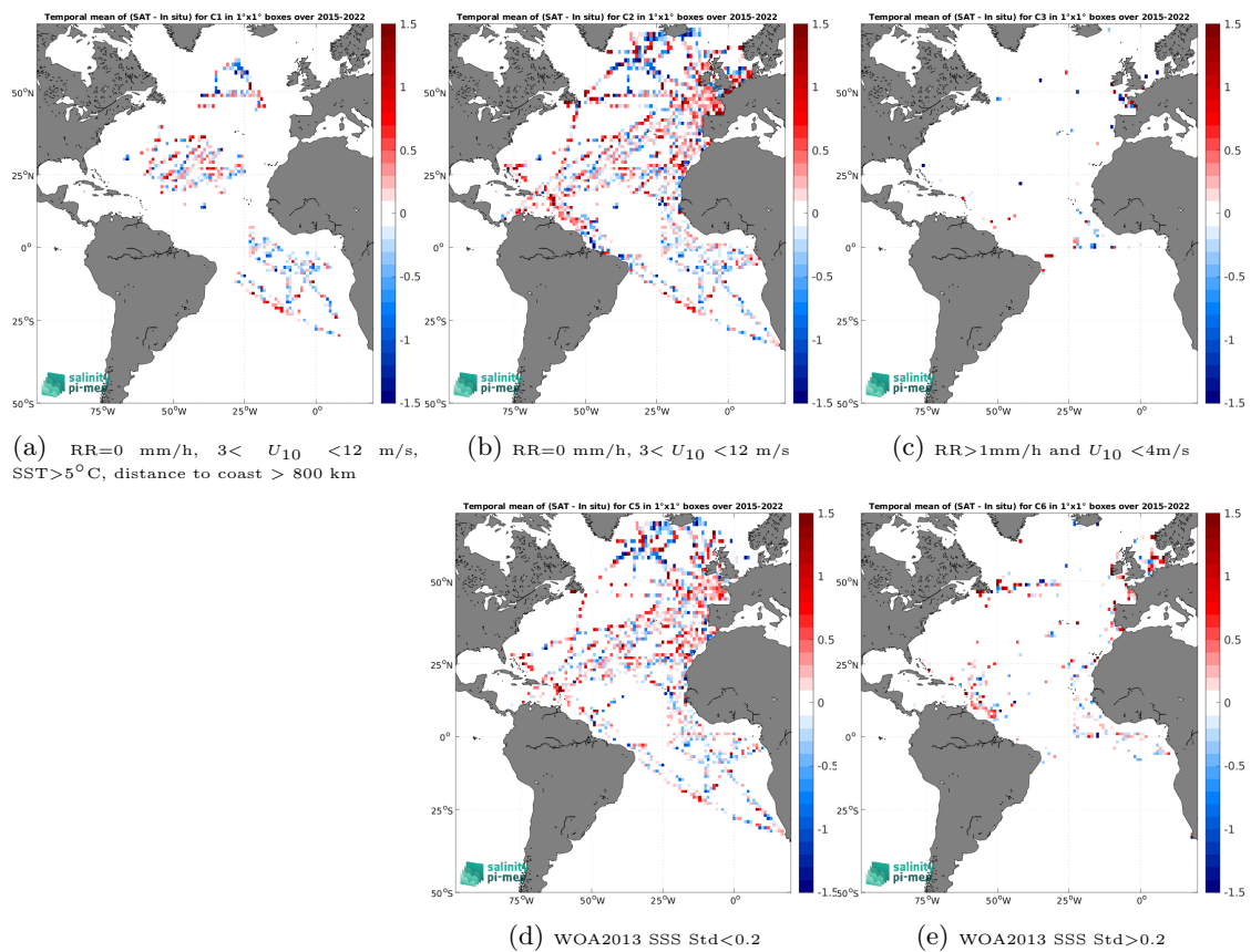
Figure 14: Temporal mean gridded over spatial boxes of size 1^\circ \times 1^\circ of \Delta SSS (SMAP SSS L2 v6 - 40 km (RSS) - TSG (GOSUD-Research-vessel)) for 5 different subdatasets corresponding to:RR=0 mm/h, 3 < U_{10} < 12 m/s, SST >5^\circ\text{C} , distance to coast > 800 km (a), RR=0 mm/h, 3 < U_{10} < 12 m/s (b), RR >1 mm/h and U_{10} < 4 m/s (c), WOA2013 SSS Std <0.2 (d), WOA2013 SSS Std >0.2 (e).
