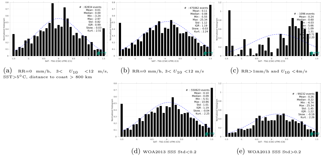
Figure 15: Normalized histogram of \Delta\text{SSS} (SMAP SSS L2 v6 - 40 km (RSS) - TSG (CSIC-UTM)) for 5 different subdatasets corresponding to: RR=0 mm/h, 3 < U_{10} < 12 m/s, SST>5°C, distance to coast > 800 km (a), RR=0 mm/h, 3 < U_{10} < 12 m/s (b), RR>1mm/h and U_{10} < 4 m/s (c), WOA2013 SSS Std<0.2 (d), WOA2013 SSS Std>0.2 (e).
