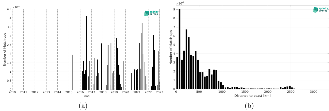
Figure 2: Number of match-ups between TSG (CSIC-UTM) and SMAP SSS L2 v6 - 40 km (RSS) SSS as a function of time (a) and as function of the distance to coast (b) over the Atlantic Ocean Pi-MEP region and for the full satellite product period.
