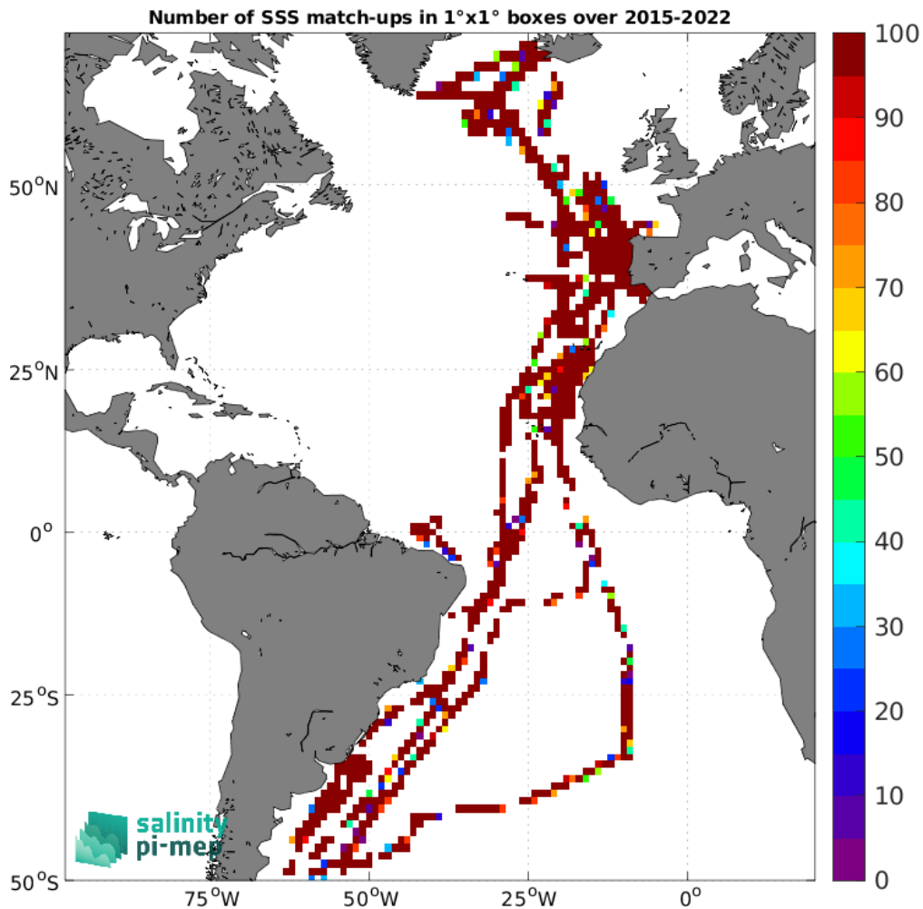
Figure 5: Number of SSS match-ups between TSG (CSIC-UTM) SSS and the SMAP SSS L2 v6 - 40 km (RSS) SSS product for the Atlantic Ocean Pi-MEP region over 1°×1° boxes and for the full satellite product period.
