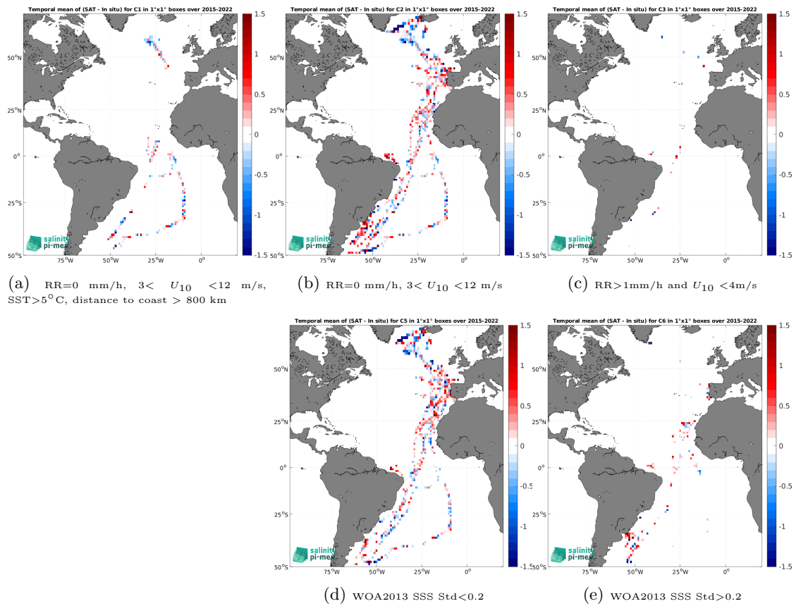
Figure 14: Temporal mean gridded over spatial boxes of size 1^\circ \times 1^\circ of \Delta SSS (SMAP SSS L2 v6 - 40 km (RSS) - TSG (CSIC-UTM)) for 5 different subdatasets corresponding to:RR=0 mm/h, 3 < U_{10} < 12 m/s, SST >5^\circ\text{C} , distance to coast > 800 km (a), RR=0 mm/h, 3 < U_{10} < 12 m/s (b), RR >1 mm/h and U_{10} < 4 m/s (c), WOA2013 SSS Std <0.2 (d), WOA2013 SSS Std >0.2 (e).
