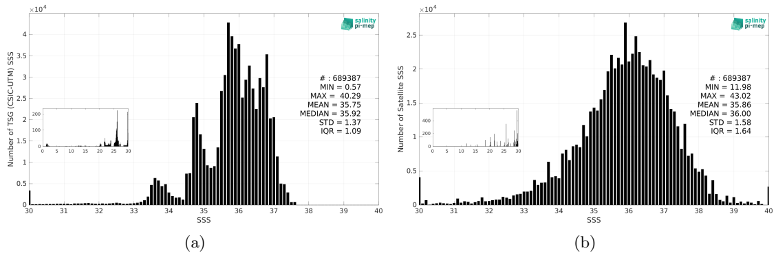
Figure 3: Histograms of SSS from TSG (CSIC-UTM) (a) and SMAP SSS L2 v6 - 40 km (RSS) (b) considering all match-up pairs per bins of 0.1 over the Atlantic Ocean Pi-MEP region and for the full satellite product period.
