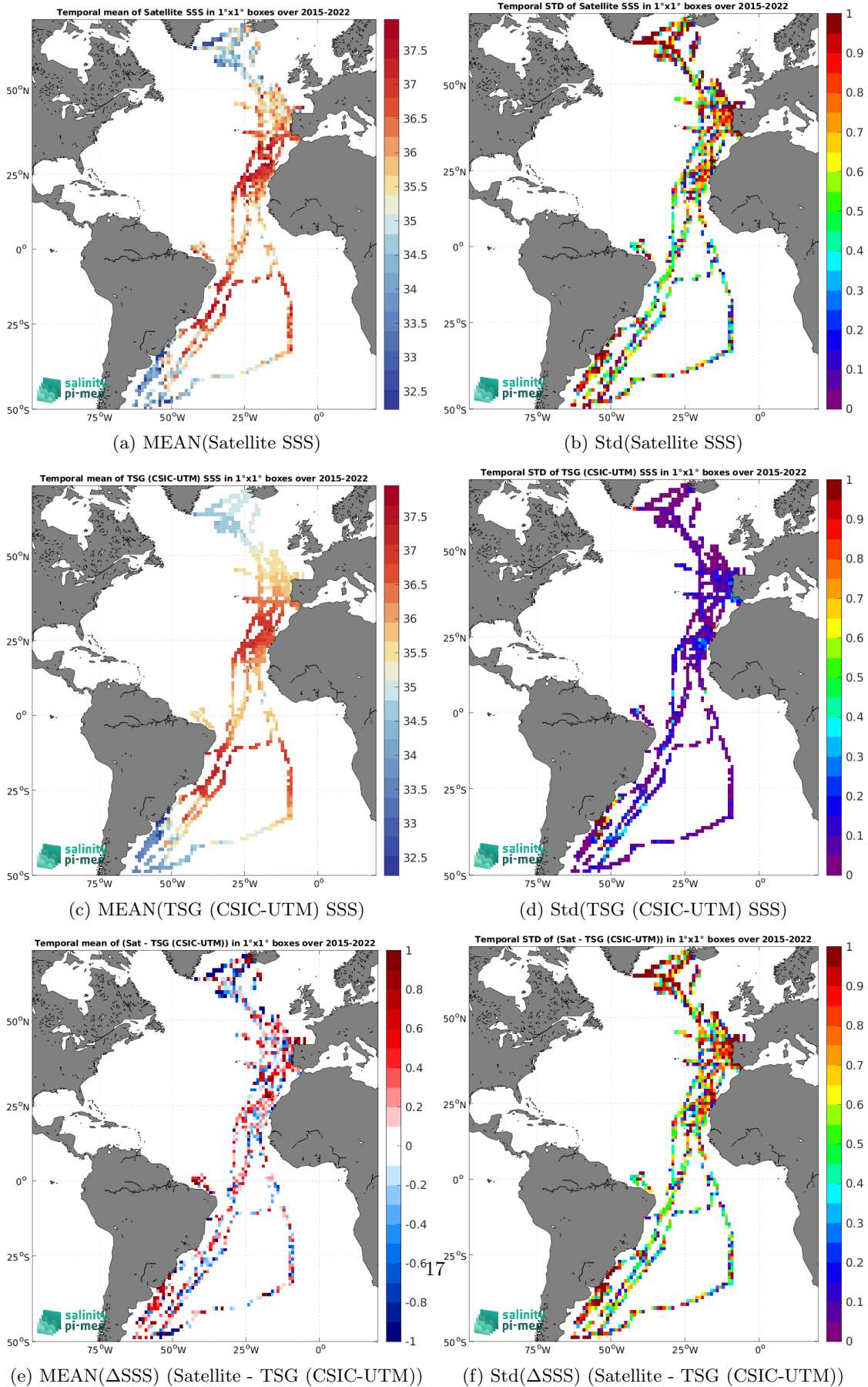
Figure 7: Temporal mean (left) and Std (right) of SSS from SMAP SSS L2 v6 - 40 km (RSS) (top), TSG (CSIC-UTM) (middle), and of \Delta SSS (Satellite - TSG (CSIC-UTM)). Only match-up pairs are used to generate these maps.
