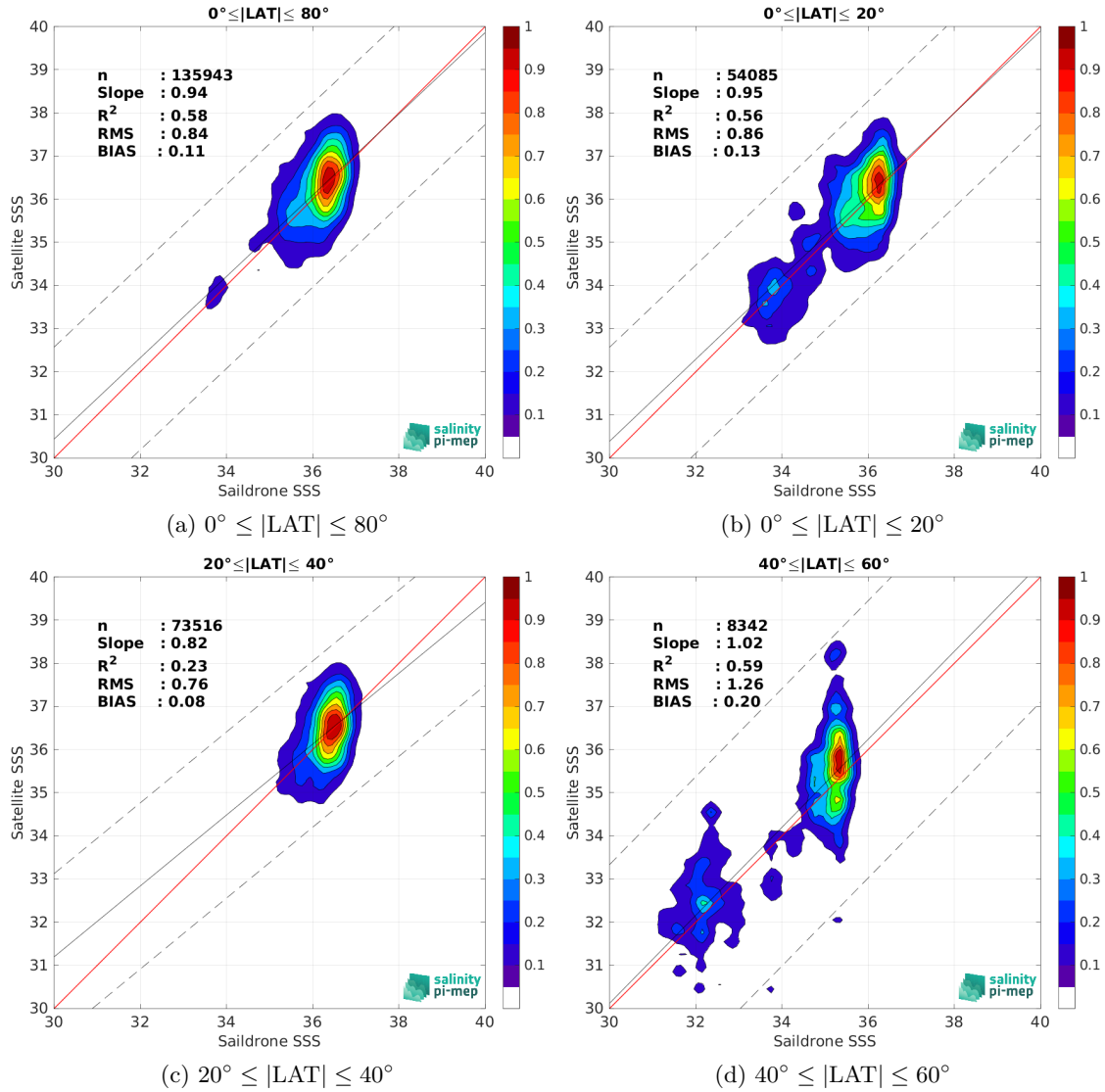
Figure 10: Contour maps of the concentration of SMAP SSS L2 v6 - 40 km (RSS) SSS (y-axis) versus Saildrone SSS (x-axis) at match-up pairs for different latitude bands. For each plot, the red line shows x=y . The black thin and dashed lines indicate a linear fit through the data cloud and the \pm 95\% confidence levels, respectively. The number match-up pairs n , the slope and R^2 coefficient of the linear fit, the root mean square (RMS) and the mean bias between satellite and in situ data are indicated for each latitude band in each plots.
