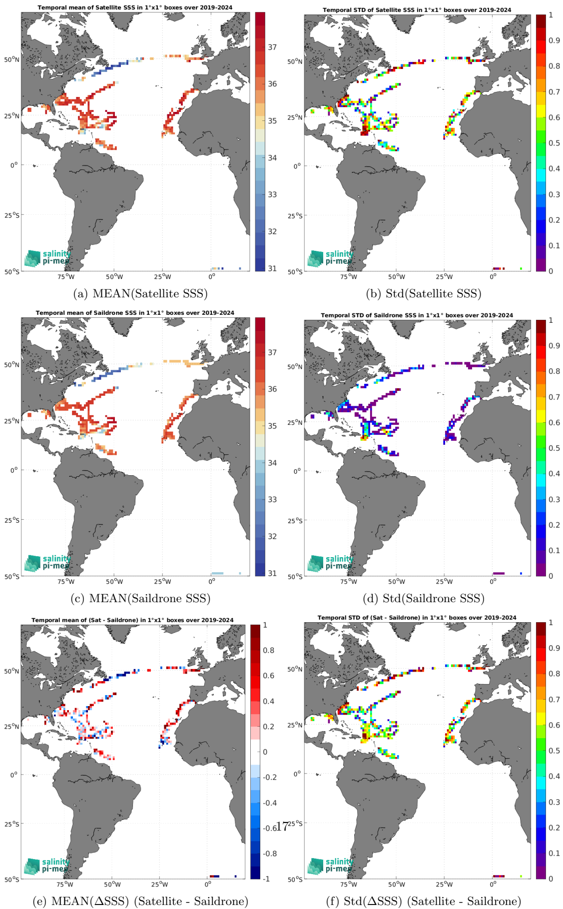
Figure 7: Temporal mean (left) and Std (right) of SSS from SMAP SSS L2 v6 - 40 km (RSS) (top), Saildrone (middle), and of \Delta SSS (Satellite - Saildrone). Only match-up pairs are used to generate these maps.
