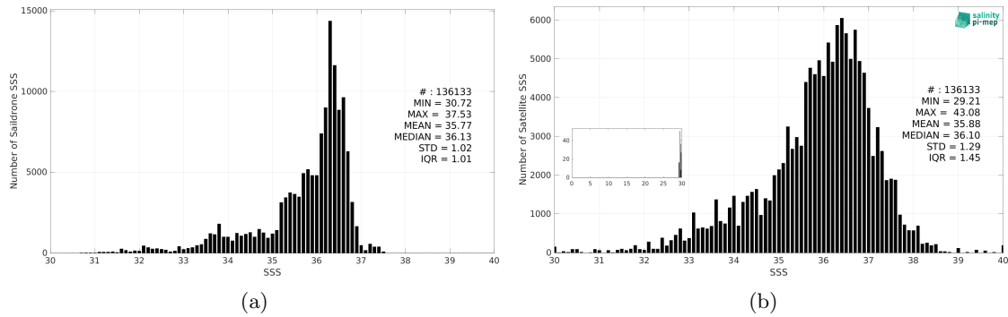
Figure 3: Histograms of SSS from Sairdrone (a) and SMAP SSS L2 v6 - 40 km (RSS) (b) considering all match-up pairs per bins of 0.1 over the Atlantic Ocean Pi-MEP region and for the full satellite product period.
