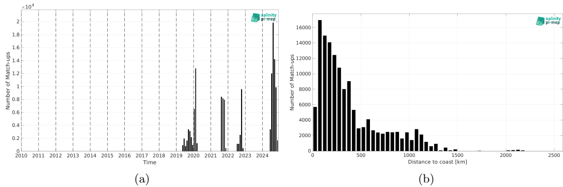
Figure 2: Number of match-ups between Sairdrone and SMAP SSS L2 v6 - 40 km (RSS) SSS as a function of time (a) and as function of the distance to coast (b) over the Atlantic Ocean Pi-MEP region and for the full satellite product period.
