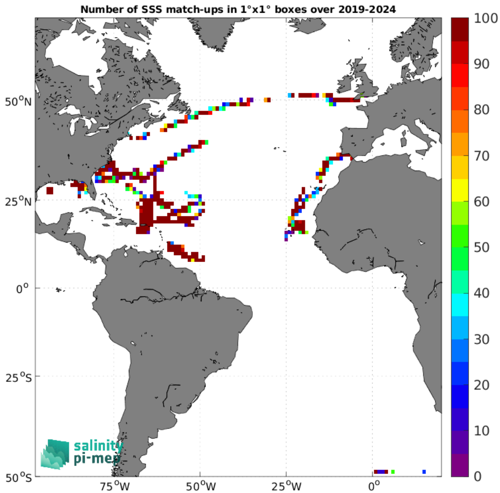
Figure 5: Number of SSS match-ups between Saildrone SSS and the SMAP SSS L2 v6 - 40 km (RSS) SSS product for the Atlantic Ocean Pi-MEP region over 1°x1° boxes and for the full satellite product period.
