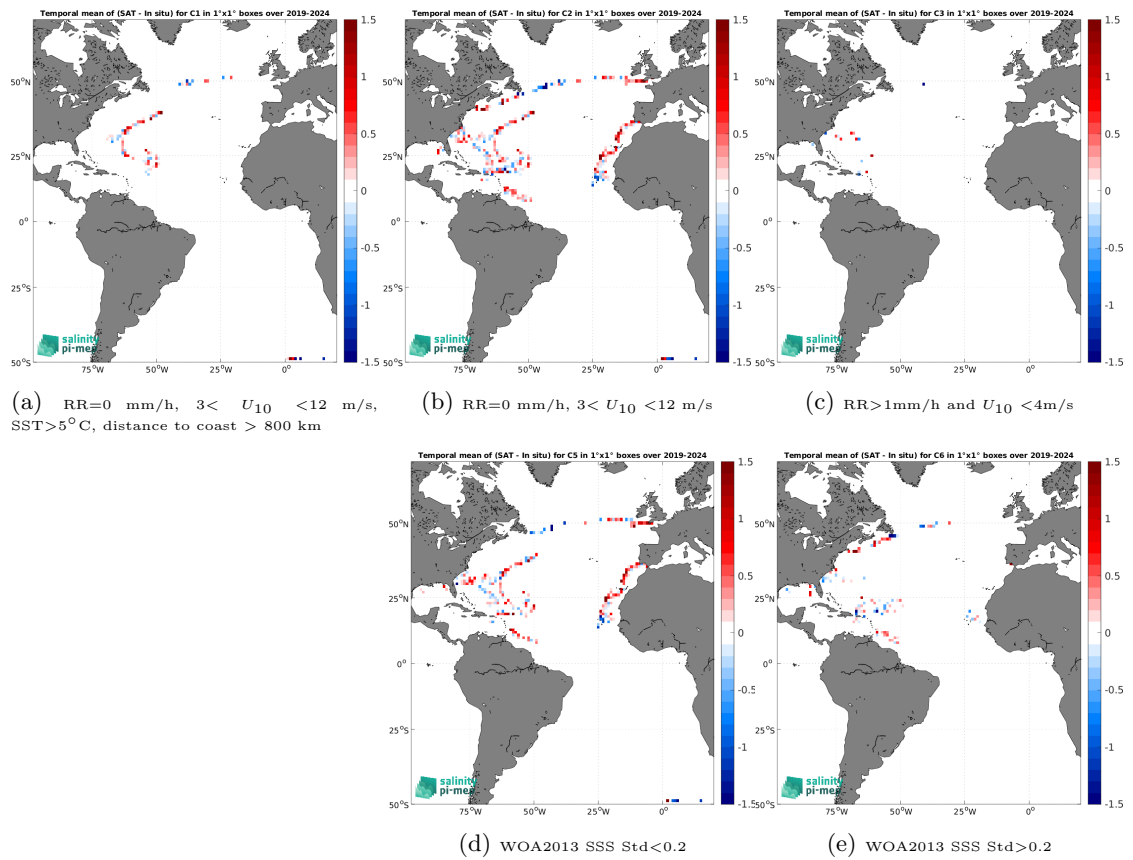
Figure 14: Temporal mean gridded over spatial boxes of size 1^\circ \times 1^\circ of \Delta\text{SSS} (SMAP SSS L2 v6 - 40 km (RSS) - Saldron) for 5 different subdatasets corresponding to:RR=0 mm/h, 3 < U_{10} < 12 m/s, SST>5°C, distance to coast > 800 km (a), RR=0 mm/h, 3 < U_{10} < 12 m/s (b), RR>1mm/h and U_{10} < 4 m/s (c), WOA2013 SSS Std<0.2 (d), WOA2013 SSS Std>0.2 (e).
