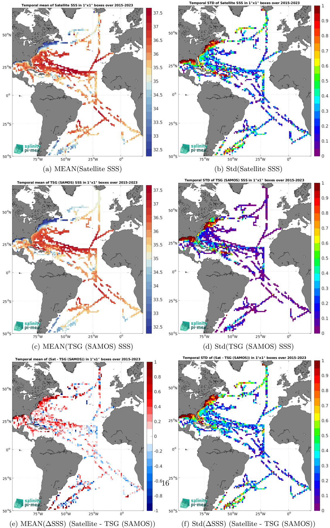
(e) MEAN( \Delta SSS) (Satellite - TSG (SAMOS)) (f) Std( \Delta SSS) (Satellite - TSG (SAMOS)) Figure 6: Temporal mean (left) and Std (right) of SSS from SMAP SSS L2 v5 (RSS) (top), TSG (SAMOS) (middle), and of \Delta SSS (Satellite - TSG (SAMOS)). Only match-up pairs are used to generate these maps.
