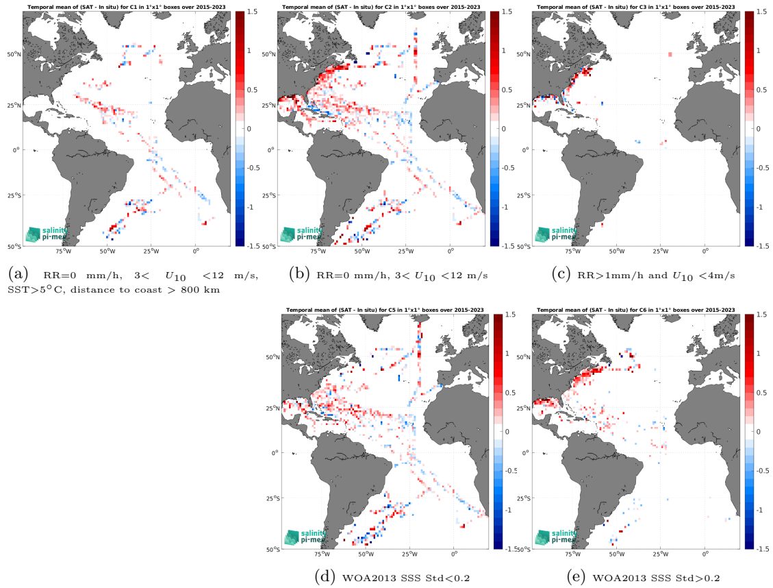
Figure 12: Temporal mean gridded over spatial boxes of size 1^\circ \times 1^\circ of \Delta\text{SSS} (SMAP SSS L2 v5 (RSS) - TSG (SAMOS)) for 5 different subdatasets corresponding to:RR=0 mm/h, 3 < U_{10} < 12 m/s, SST >5^\circ\text{C} , distance to coast > 800 km (a), RR=0 mm/h, 3 < U_{10} < 12 m/s (b), RR >1 mm/h and U_{10} < 4 m/s (c), WOA2013 SSS Std <0.2 (d), WOA2013 SSS Std >0.2 (e).
