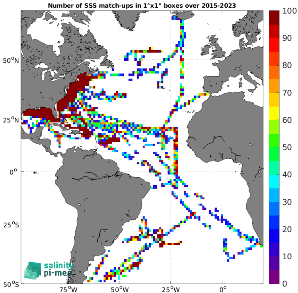
Figure 4: Number of SSS match-ups between TSG (SAMOS) SSS and the SMAP SSS L2 v5 (RSS) SSS product for the Atlantic Ocean Pi-MEP region over 1^{\circ} \times 1^{\circ} boxes and for the full satellite product period.
