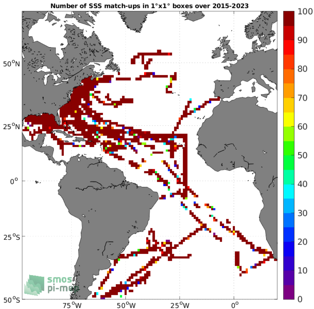
Figure 4: Number of SSS match-ups between TSG (SAMOS) SSS and the SMAP SSS L2 v5 (RSS) SSS product for the Atlantic Ocean Pi-MEP region over 1°x1° boxes and for the full satellite product period.
