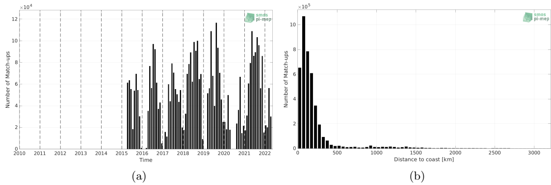
Figure 1: Number of match-ups between TSG (SAMOS) and SMAP SSS L2 v5 (RSS) SSS as a function of time (a) and as function of the distance to coast (b) over the Atlantic Ocean Pi-MEP region and for the full satellite product period.
