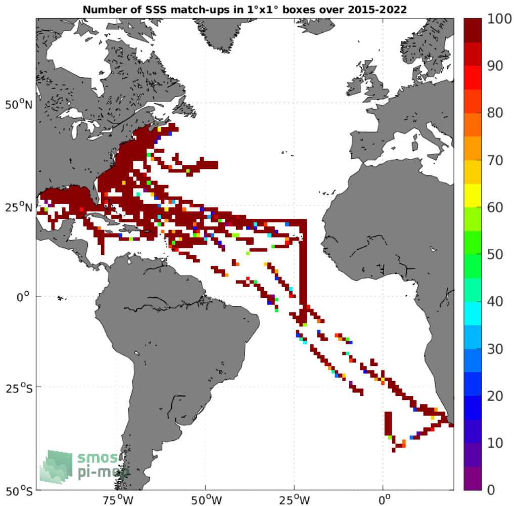
Figure 4: Number of SSS match-ups between TSG (SAMOS) SSS and the SMAP SSS L2 v5 (RSS) SSS product for the Atlantic Ocean Pi-MEP region over 1^\circ \times 1^\circ boxes and for the full satellite product period.
