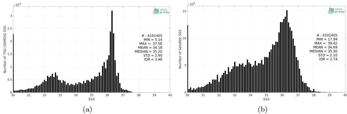
Figure 2: Histograms of SSS from TSG (SAMOS) (a) and SMAP SSS L2 v5 (RSS) (b) considering all match-up pairs per bins of 0.1 over the Atlantic Ocean Pi-MEP region and for the full satellite product period.
