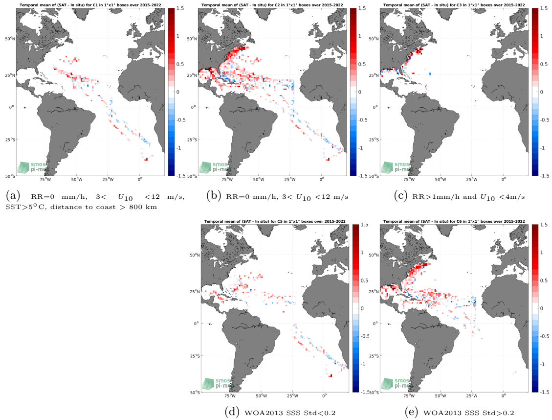
Figure 12: Temporal mean gridded over spatial boxes of size 1^\circ \times 1^\circ of \Delta SSS (SMAP SSS L2 v5 (RSS) - TSG (SAMOS)) for 5 different subdatasets corresponding to:RR=0 mm/h, 3 < U_{10} < 12 m/s, SST >5^\circ\text{C} , distance to coast > 800 km (a), RR=0 mm/h, 3 < U_{10} < 12 m/s (b), RR >1 mm/h and U_{10} < 4 m/s (c), WOA2013 SSS Std <0.2 (d), WOA2013 SSS Std >0.2 (e).
