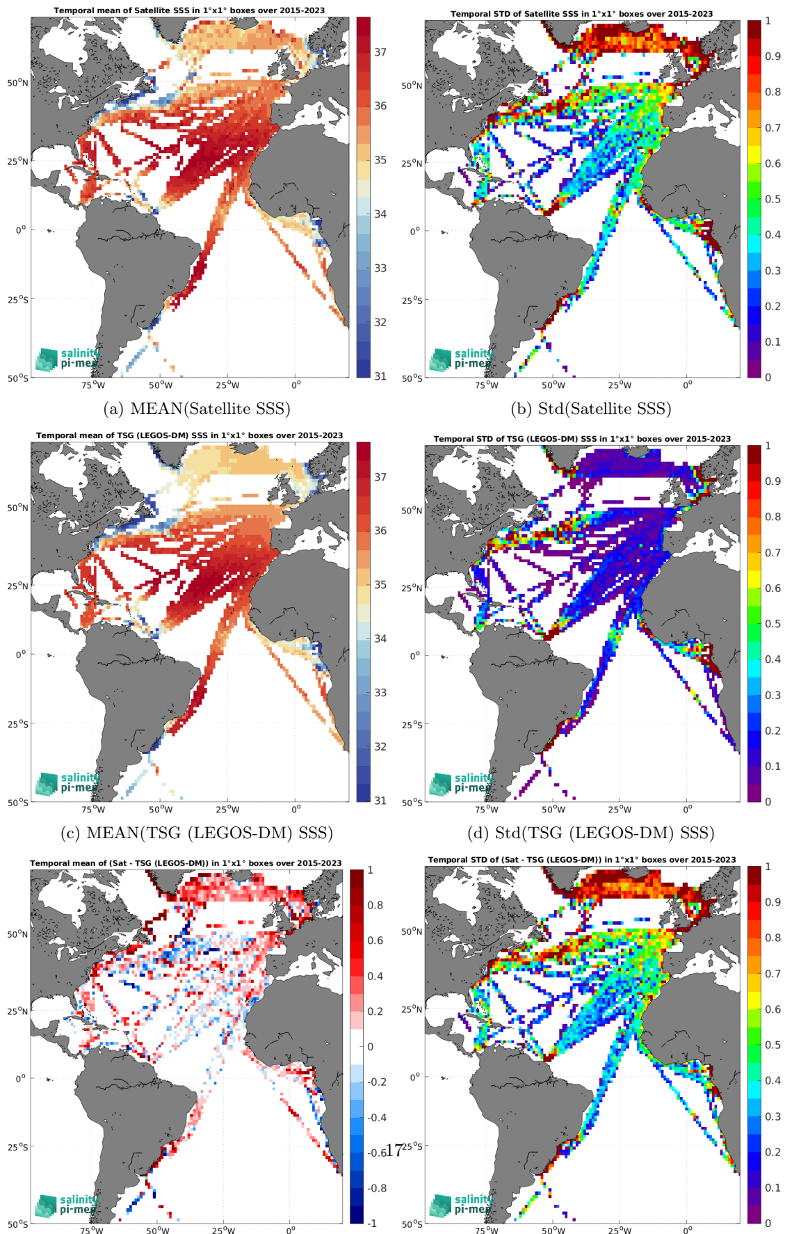
(e) MEAN( \Delta SSS) (Satellite - TSG (LEGOS-DM)) (f) Std( \Delta SSS) (Satellite - TSG (LEGOS-DM)) Figure 6: Temporal mean (left) and Std (right) of SSS from SMAP SSS L2 v5 (RSS) (top), TSG (LEGOS-DM) (middle), and of \Delta SSS (Satellite - TSG (LEGOS-DM)). Only match-up pairs are used to generate these maps.
