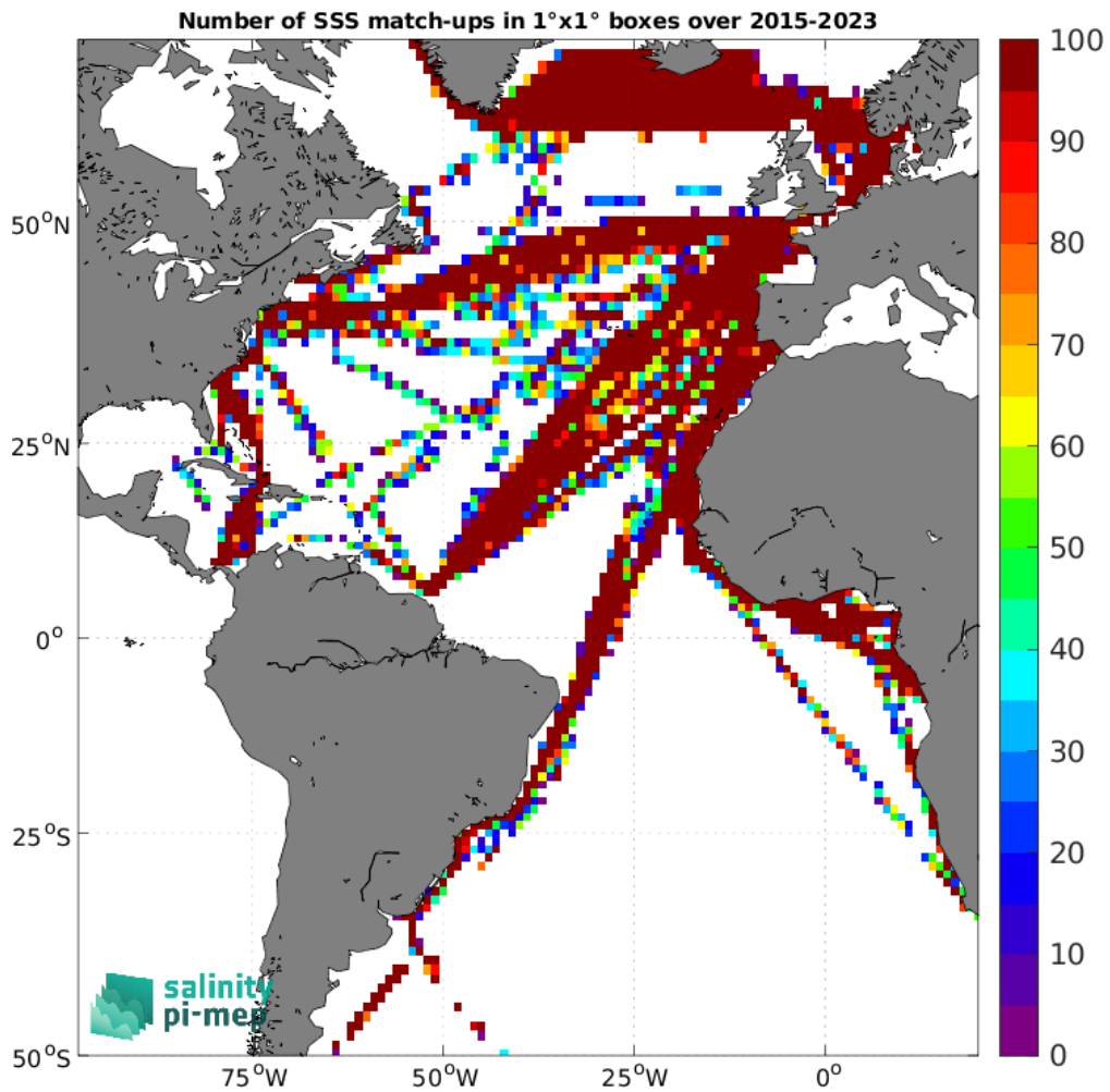
Figure 4: Number of SSS match-ups between TSG (LEGOS-DM) SSS and the SMAP SSS L2 v5 (RSS) SSS product for the Atlantic Ocean Pi-MEP region over 1^\circ \times 1^\circ boxes and for the full satellite product period.
