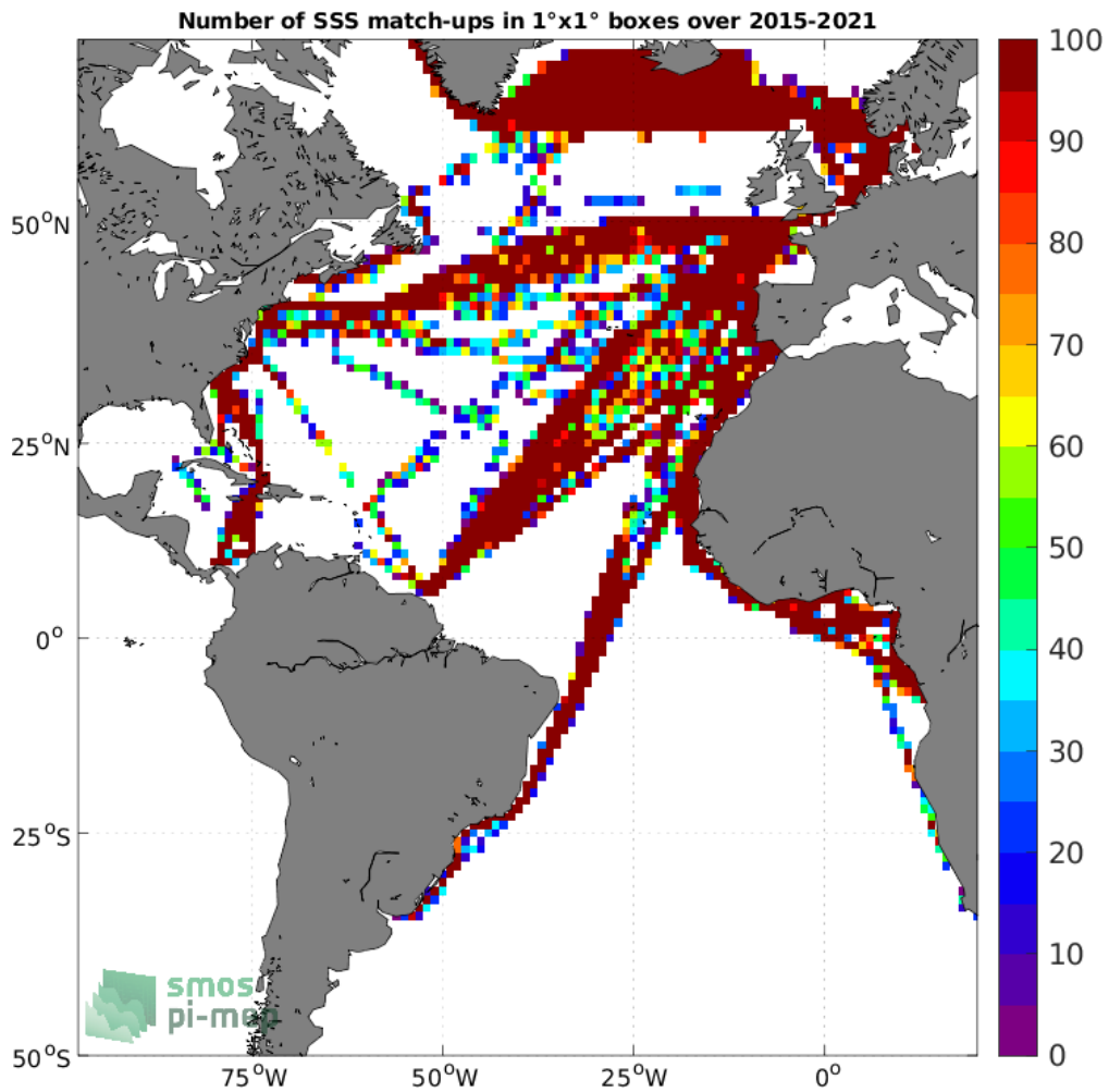
Figure 4: Number of SSS match-ups between TSG (LEGOS-DM) SSS and the SMAP SSS L2 v5 (RSS) SSS product for the Atlantic Ocean Pi-MEP region over 1°x1° boxes and for the full satellite product period.
