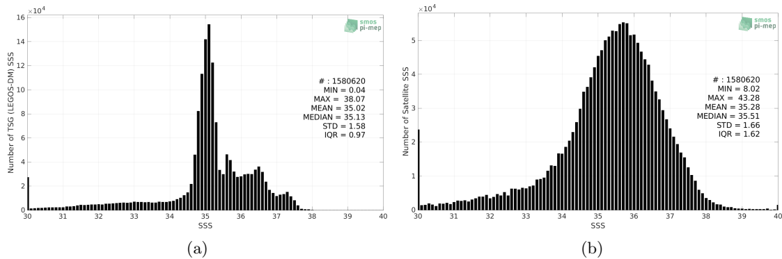
Figure 2: Histograms of SSS from TSG (LEGOS-DM) (a) and SMAP SSS L2 v5 (RSS) (b) considering all match-up pairs per bins of 0.1 over the Atlantic Ocean Pi-MEP region and for the full satellite product period.
