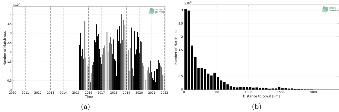
Figure 1: Number of match-ups between TSG (LEGOS-DM) and SMAP SSS L2 v5 (RSS) SSS as a function of time (a) and as function of the distance to coast (b) over the Atlantic Ocean Pi-MEP region and for the full satellite product period.
