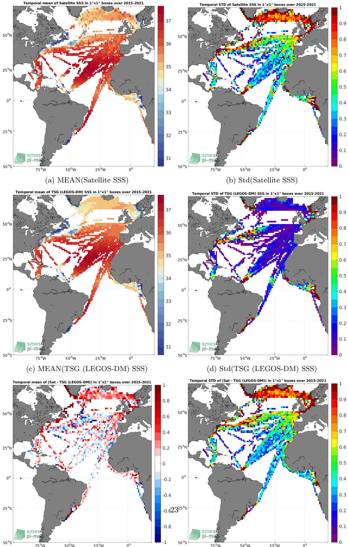
Figure 6: Temporal mean (left) and Std (right) of SSS from SMAP SSS L2 v5 (RSS) (top), TSG (LEGOS-DM) (middle), and of \Delta SSS (Satellite - TSG (LEGOS-DM)). Only match-up pairs are used to generate these maps.
