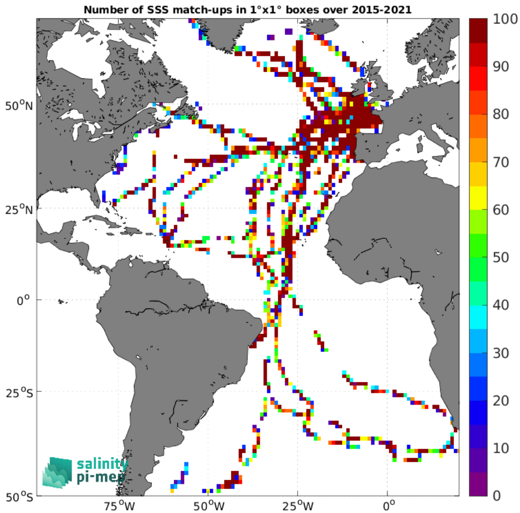
Figure 4: Number of SSS match-ups between TSG (GOSUD-Sailing-ship) SSS and the SMAP SSS L2 v5 (RSS) SSS product for the Atlantic Ocean Pi-MEP region over 1^\circ \times 1^\circ boxes and for the full satellite product period.
