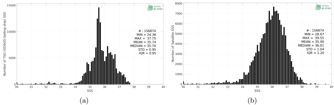
Figure 2: Histograms of SSS from TSG (GOSUD-Sailing-ship) (a) and SMAP SSS L2 v5 (RSS) (b) considering all match-up pairs per bins of 0.1 over the Atlantic Ocean Pi-MEP region and for the full satellite product period.
