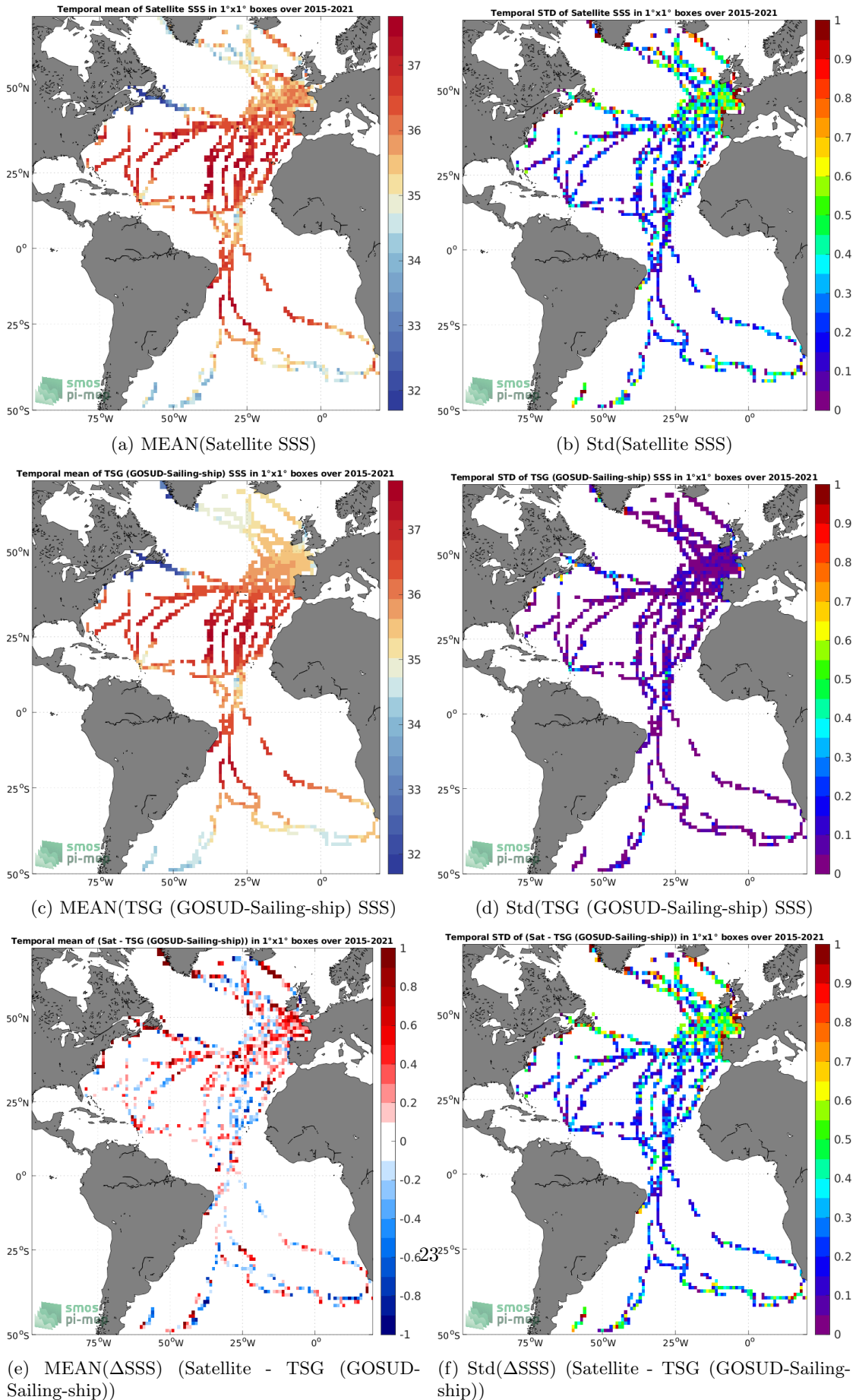
Figure 6: Temporal mean (left) and Std (right) of SSS from SMAP SSS L2 v5 (RSS) (top), TSG (GOSUD-Sailing-ship) (middle), and of \Delta SSS (Satellite - TSG (GOSUD-Sailing-ship)). Only match-up pairs are used to generate these maps.
