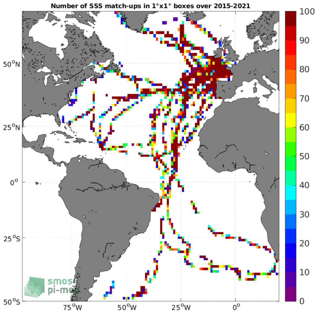
Figure 4: Number of SSS match-ups between TSG (GOSUD-Sailing-ship) SSS and the SMAP SSS L2 v5 (RSS) SSS product for the Atlantic Ocean Pi-MEP region over 1°x1° boxes and for the full satellite product period.
