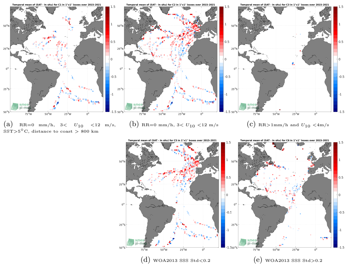
Figure 12: Temporal mean gridded over spatial boxes of size 1^\circ \times 1^\circ of \Delta SSS (SMAP SSS L2 v5 (RSS) - TSG (GOSUD-Sailing-ship)) for 5 different subdatasets corresponding to:RR=0 mm/h, 3 < U_{10} < 12 m/s, SST>5°C, distance to coast > 800 km (a), RR=0 mm/h, 3 < U_{10} < 12 m/s (b), RR>1mm/h and U_{10} < 4 m/s (c), WOA2013 SSS Std<0.2 (d), WOA2013 SSS Std>0.2 (e).
