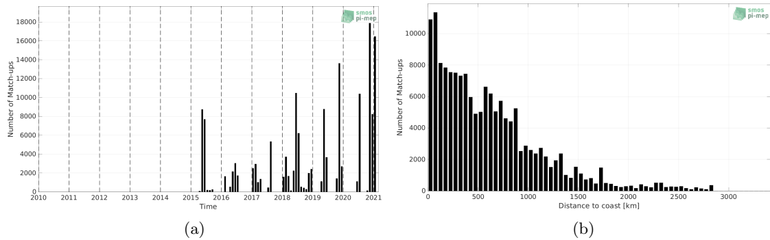
Figure 1: Number of match-ups between TSG (GOSUD-Sailing-ship) and SMAP SSS L2 v5 (RSS) SSS as a function of time (a) and as function of the distance to coast (b) over the Atlantic Ocean Pi-MEP region and for the full satellite product period.
