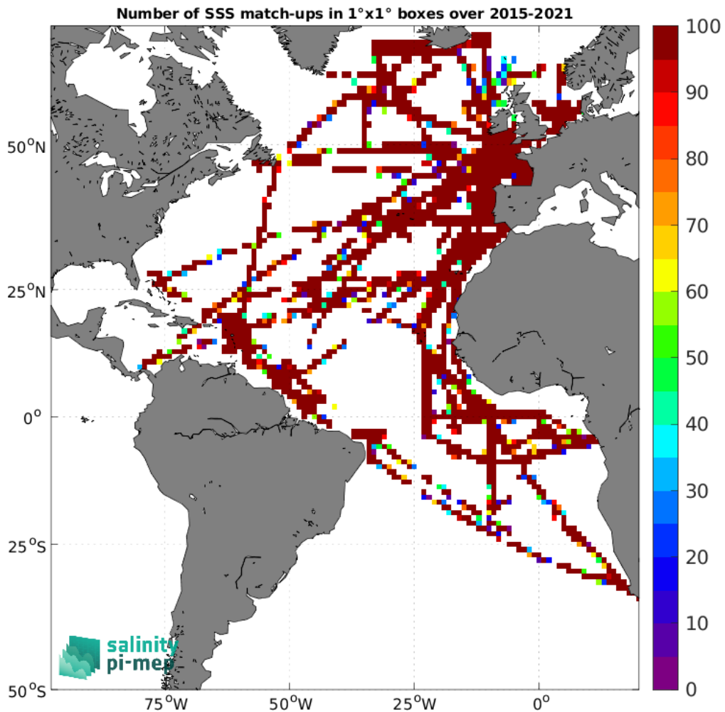
Figure 4: Number of SSS match-ups between TSG (GOSUD-Research-vessel) SSS and the SMAP SSS L2 v5 (RSS) SSS product for the Atlantic Ocean Pi-MEP region over 1^{\circ} \times 1^{\circ} boxes and for the full satellite product period.
