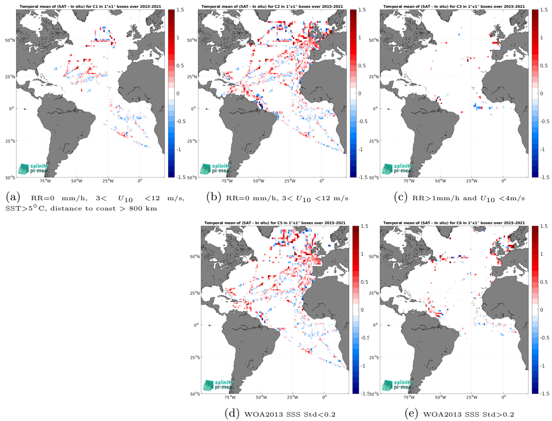
Figure 12: Temporal mean gridded over spatial boxes of size 1^\circ \times 1^\circ of \Delta\text{SSS} (SMAP SSS L2 v5 (RSS) - TSG (GOSUD-Research-vessel)) for 5 different subdatasets corresponding to:RR=0 mm/h, 3 < U_{10} < 12 m/s, SST>5°C, distance to coast > 800 km (a), RR=0 mm/h, 3 < U_{10} < 12 m/s (b), RR>1mm/h and U_{10} < 4 m/s (c), WOA2013 SSS Std<0.2 (d), WOA2013 SSS Std>0.2 (e).
