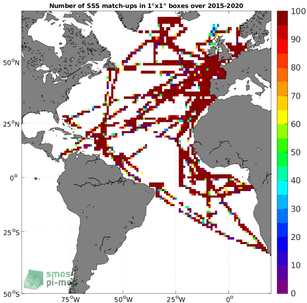
Figure 4: Number of SSS match-ups between TSG (GOSUD-Research-vessel) SSS and the SMAP SSS L2 v5 (RSS) SSS product for the Atlantic Ocean Pi-MEP region over 1°x1° boxes and for the full satellite product period.
