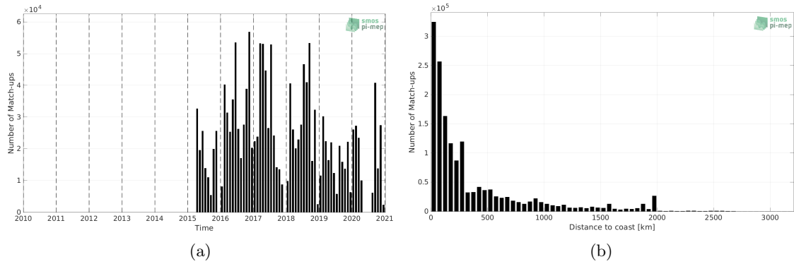
Figure 1: Number of match-ups between TSG (GOSUD-Research-vessel) and SMAP SSS L2 v5 (RSS) SSS as a function of time (a) and as function of the distance to coast (b) over the Atlantic Ocean Pi-MEP region and for the full satellite product period.
