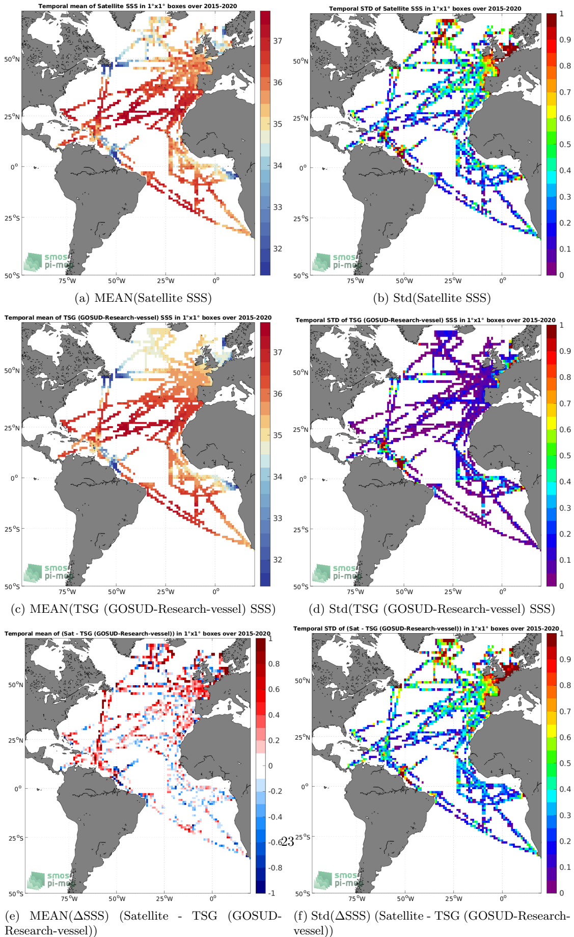
Figure 6: Temporal mean (left) and Std (right) of SSS from SMAP SSS L2 v5 (RSS) (top), TSG (GOSUD-Research-vessel) (middle), and of \Delta SSS (Satellite - TSG (GOSUD-Research-vessel)). Only match-up pairs are used to generate these maps.
