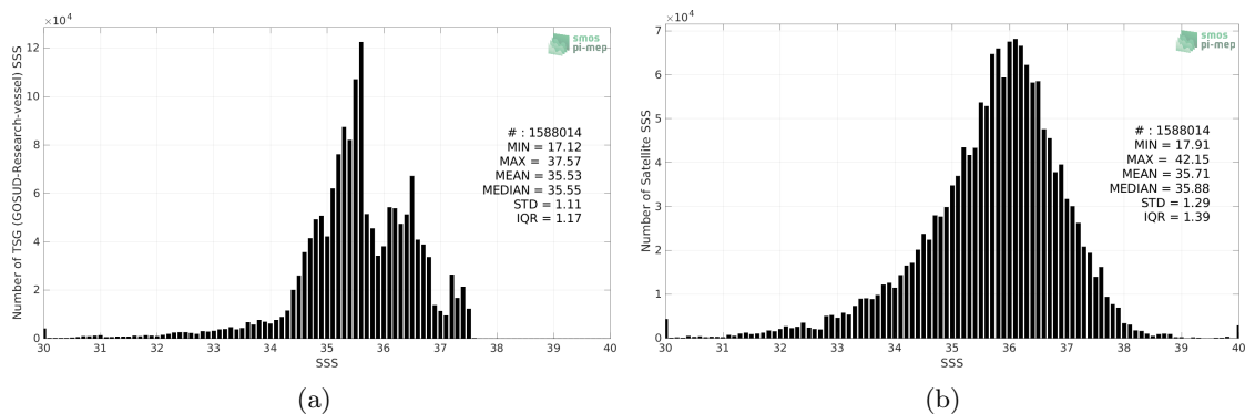
Figure 2: Histograms of SSS from TSG (GOSUD-Research-vessel) (a) and SMAP SSS L2 v5 (RSS) (b) considering all match-up pairs per bins of 0.1 over the Atlantic Ocean Pi-MEP region and for the full satellite product period.
