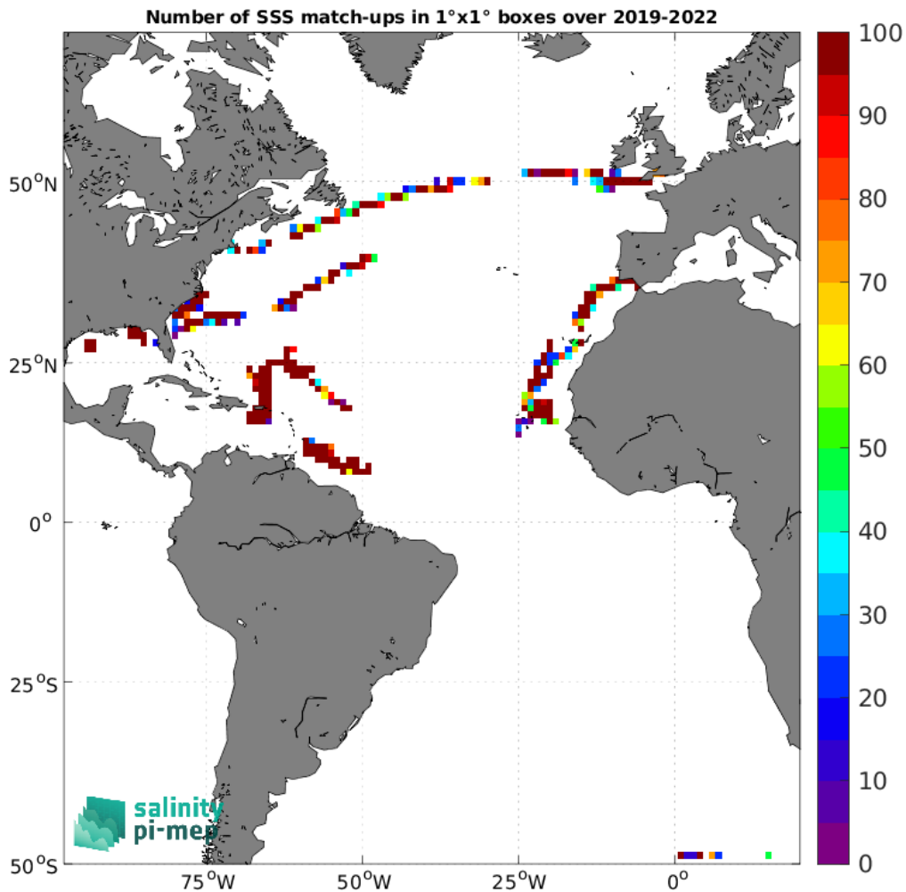
Figure 4: Number of SSS match-ups between Saildrone SSS and the SMAP SSS L2 v5 (RSS) SSS product for the Atlantic Ocean Pi-MEP region over 1°×1° boxes and for the full satellite product period.
