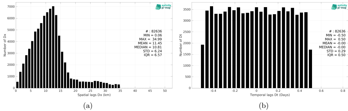
Figure 5: Histograms of the spatial (a) and temporal (b) lags between the location/time of the Sairdrone measurement and the date of the corresponding SMAP SSS L2 v5 (RSS) SSS pixel.
