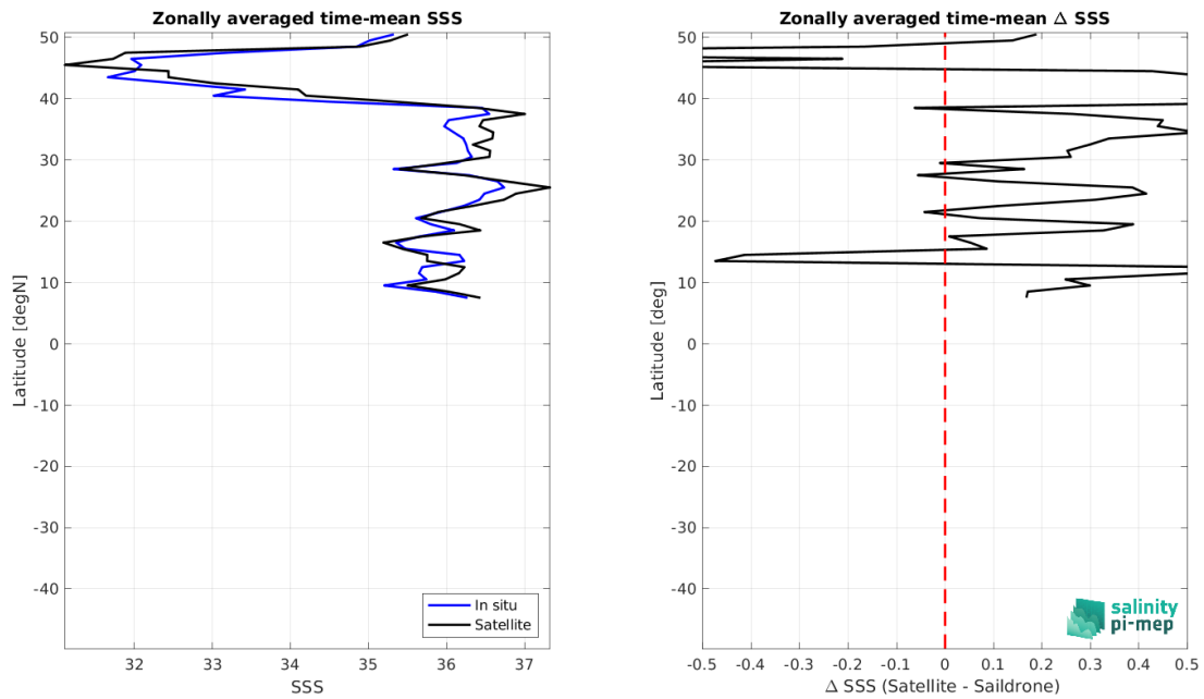
Figure 8: Left panel: Zonal mean SSS from SMAP SSS L2 v5 (RSS) satellite product (black) and from Saildrone (blue). Right panel: Zonal mean of \Delta SSS (Satellite - Saildrone) for all the collected Pi-MEP match-up pairs estimated over the full satellite product period.
