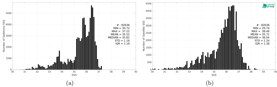
Figure 2: Histograms of SSS from Saildrone (a) and SMAP SSS L2 v5 (RSS) (b) considering all match-up pairs per bins of 0.1 over the Atlantic Ocean Pi-MEP region and for the full satellite product period.
