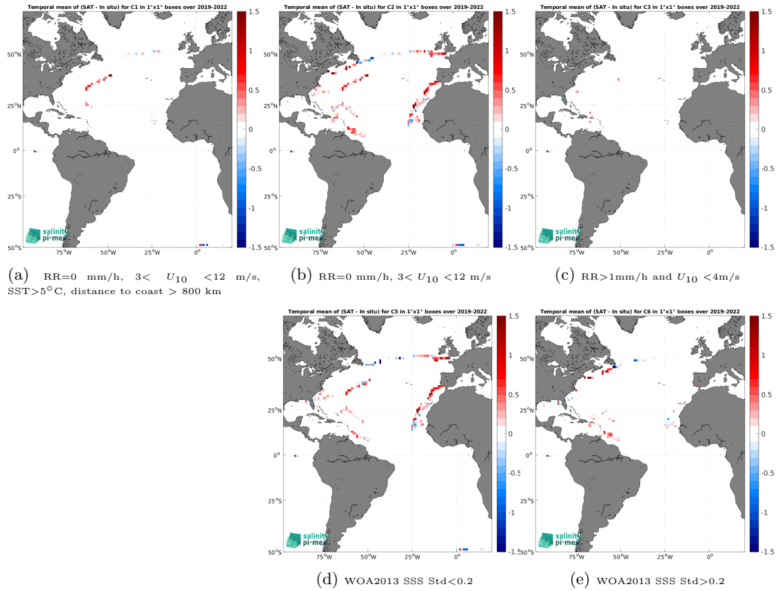
Figure 12: Temporal mean gridded over spatial boxes of size 1^\circ \times 1^\circ of \Delta SSS (SMAP SSS L2 v5 (RSS) - Saildrone) for 5 different subdatasets corresponding to:RR=0 mm/h, 3 < U_{10} < 12 m/s, SST >5^\circ\text{C} , distance to coast > 800 km (a), RR=0 mm/h, 3 < U_{10} < 12 m/s (b), RR >1 mm/h and U_{10} < 4 m/s (c), WOA2013 SSS Std <0.2 (d), WOA2013 SSS Std >0.2 (e).
