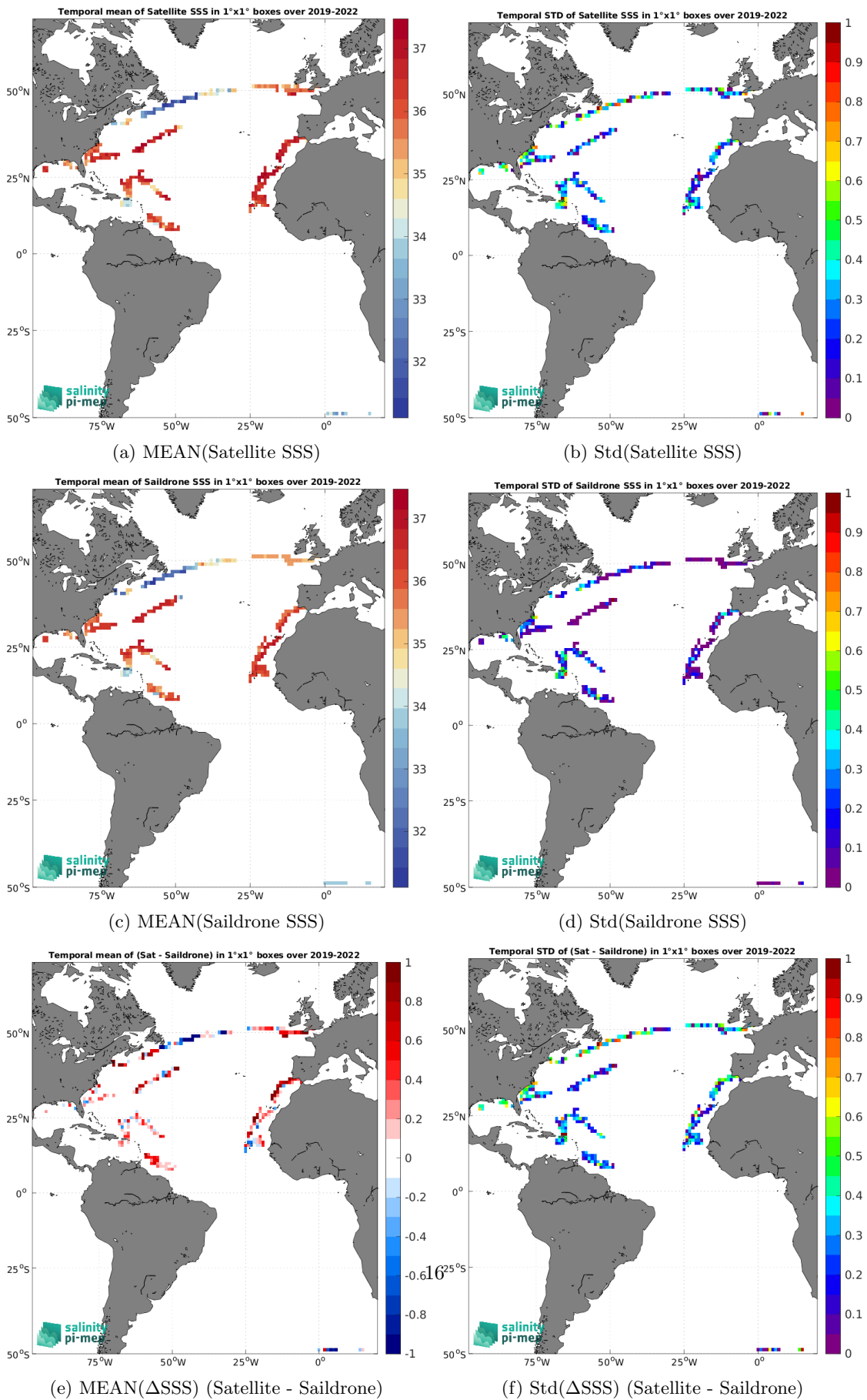
Figure 6: Temporal mean (left) and Std (right) of SSS from SMAP SSS L2 v5 (RSS) (top), Saildrone (middle), and of \Delta SSS (Satellite - Saildrone). Only match-up pairs are used to generate these maps.
