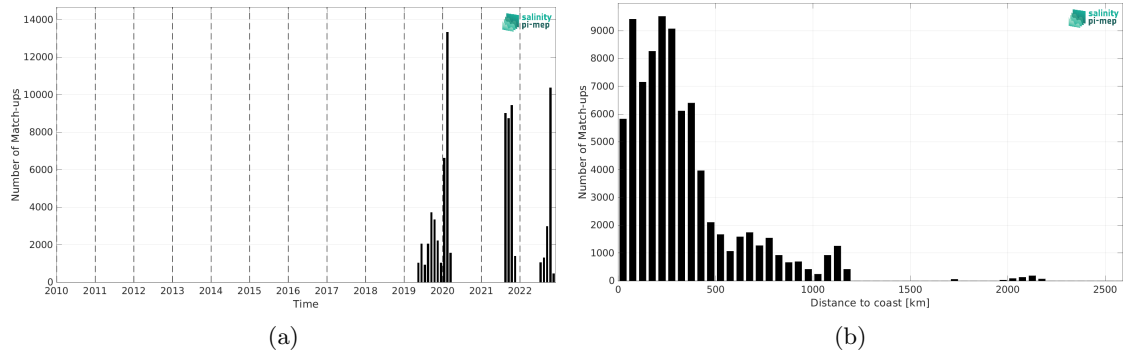
Figure 1: Number of match-ups between Saildrone and SMAP SSS L2 v5 (RSS) SSS as a function of time (a) and as function of the distance to coast (b) over the Atlantic Ocean Pi-MEP region and for the full satellite product period.
