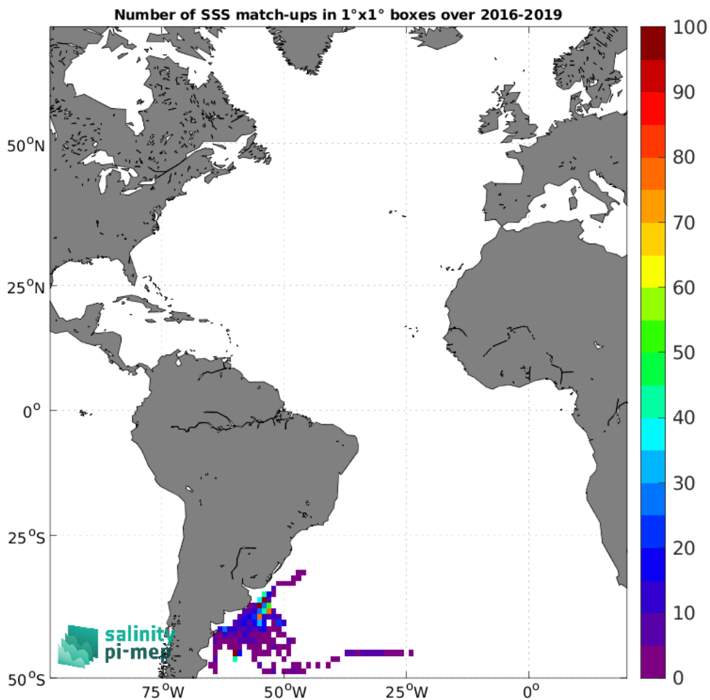
Figure 4: Number of SSS match-ups between Marine mammals SSS and the SMAP SSS L2 v5 (RSS) SSS product for the Atlantic Ocean Pi-MEP region over 1°×1° boxes and for the full satellite product period.
