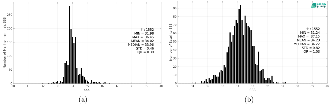
Figure 2: Histograms of SSS from Marine mammals (a) and SMAP SSS L2 v5 (RSS) (b) considering all match-up pairs per bins of 0.1 over the Atlantic Ocean Pi-MEP region and for the full satellite product period.
