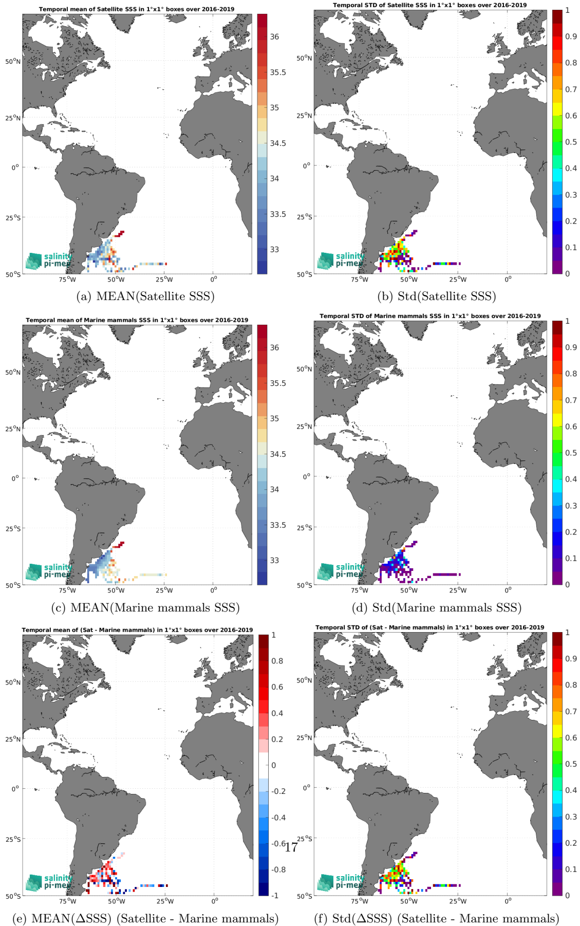
Figure 6: Temporal mean (left) and Std (right) of SSS from SMAP SSS L2 v5 (RSS) (top), Marine mammals (middle), and of \Delta SSS (Satellite - Marine mammals). Only match-up pairs are used to generate these maps.
