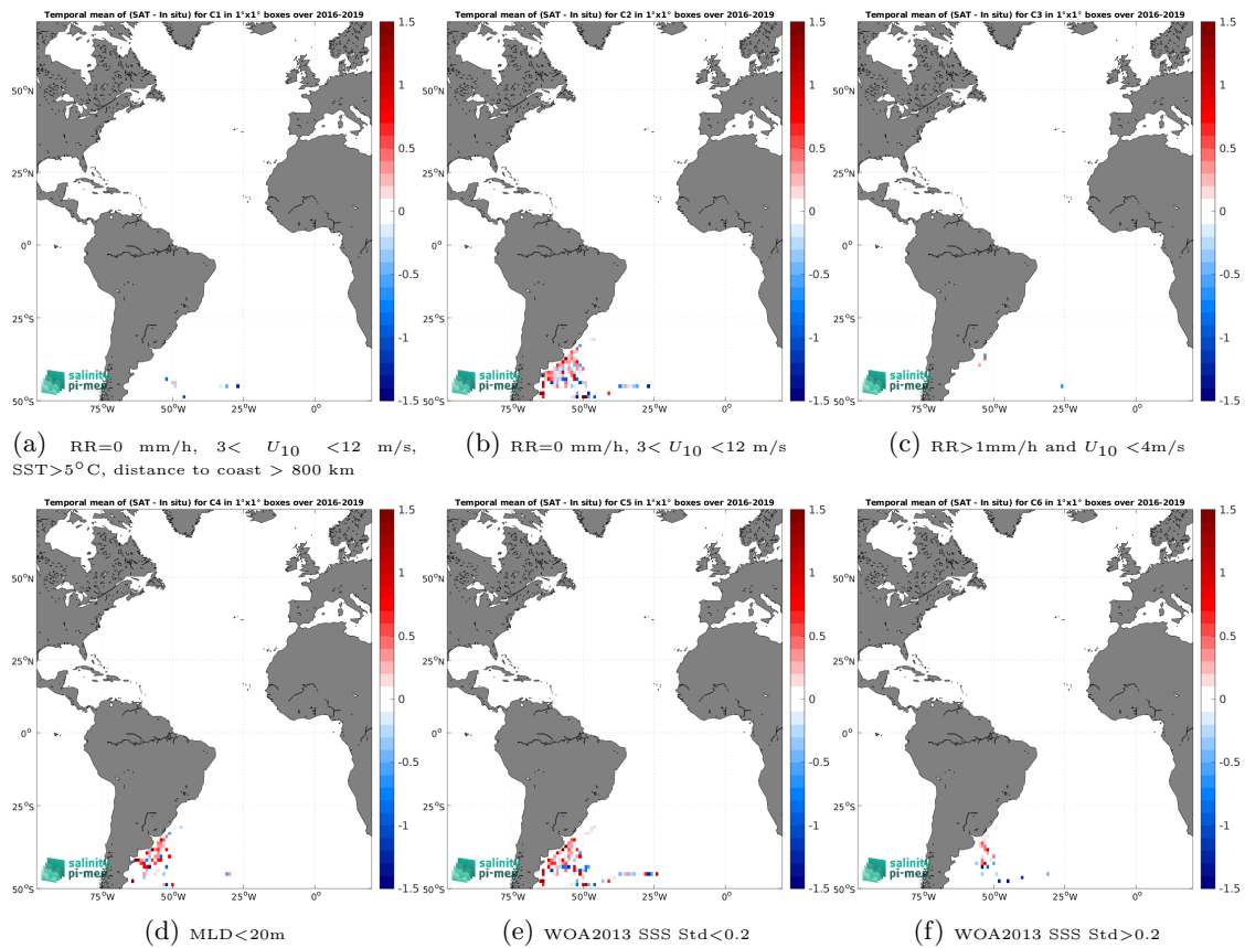
Figure 12: Temporal mean gridded over spatial boxes of size 1^\circ \times 1^\circ of \Delta SSS (SMAP SSS L2 v5 (RSS) - Marine mammals) for 6 different subdatasets corresponding to:RR=0 mm/h, 3 < U_{10} < 12 m/s, SST >5^\circ\text{C} , distance to coast > 800 km (a), RR=0 mm/h, 3 < U_{10} < 12 m/s (b), RR >1 mm/h and U_{10} < 4 m/s (c),MLD <20 m (d),WOA2013 SSS Std <0.2 (e),WOA2013 SSS Std >0.2 (f).
