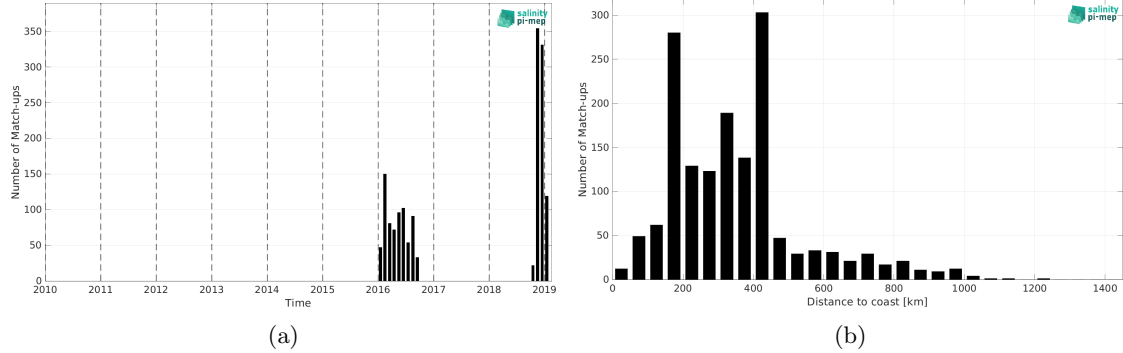
Figure 1: Number of match-ups between Marine mammals and SMAP SSS L2 v5 (RSS) SSS as a function of time (a) and as function of the distance to coast (b) over the Atlantic Ocean Pi-MEP region and for the full satellite product period.
