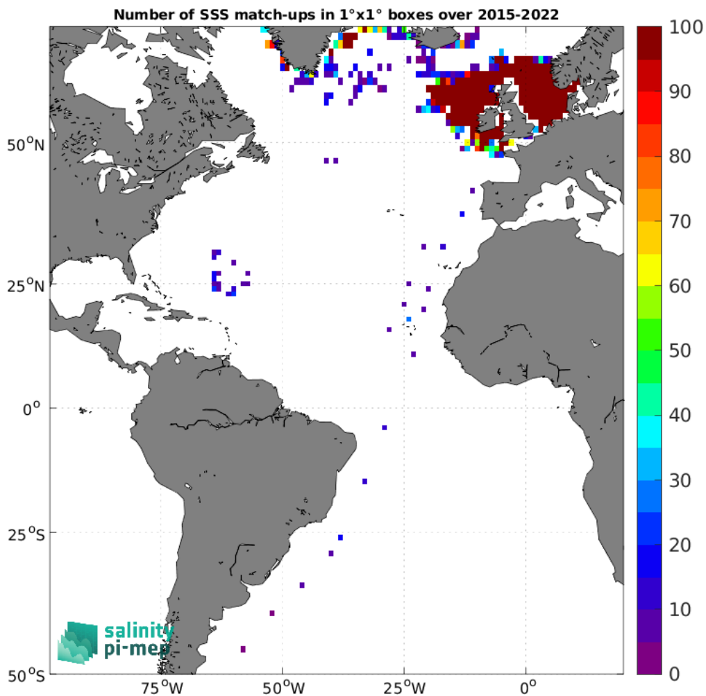
Figure 4: Number of SSS match-ups between ICES SSS and the SMAP SSS L2 v5 (RSS) SSS product for the Atlantic Ocean Pi-MEP region over 1^{\circ} \times 1^{\circ} boxes and for the full satellite product period.
