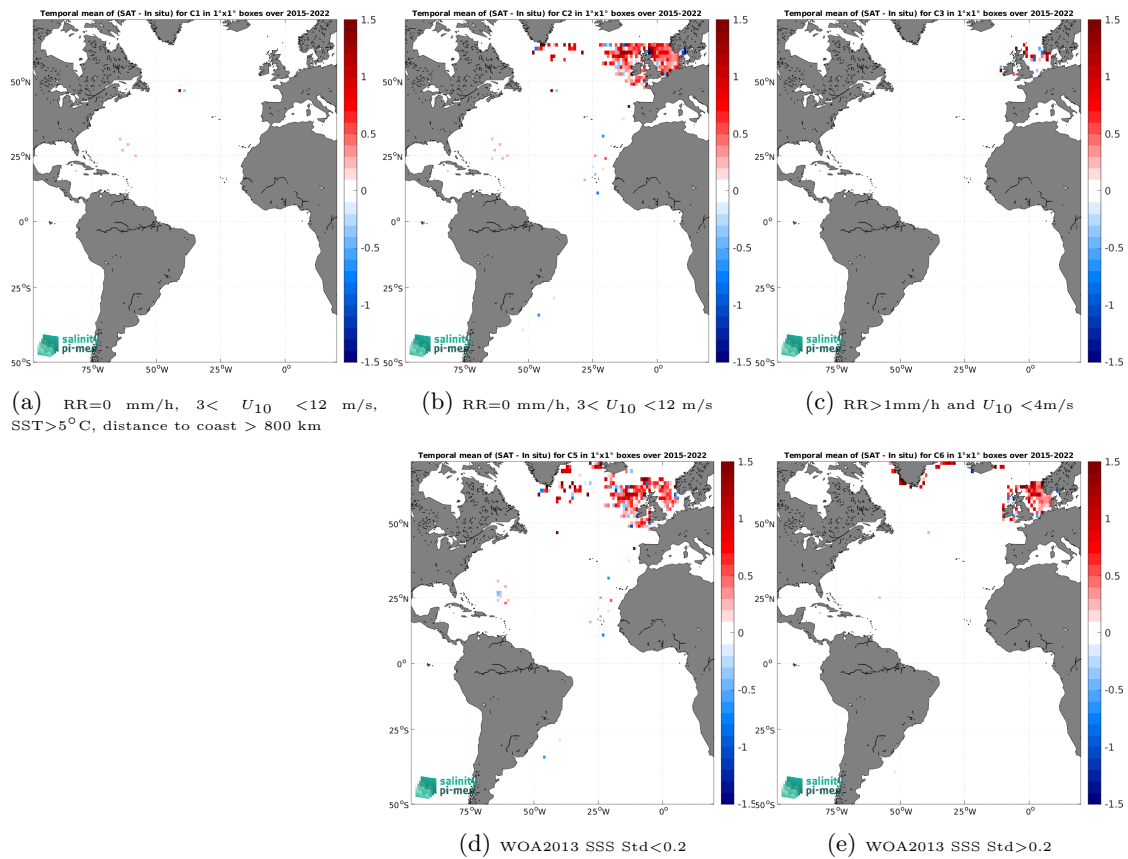
Figure 12: Temporal mean gridded over spatial boxes of size 1^\circ \times 1^\circ of \Delta SSS (SMAP SSS L2 v5 (RSS) - ICES) for 5 different subdatasets corresponding to:RR=0 mm/h, 3 < U_{10} < 12 m/s, SST >5^\circ\text{C} , distance to coast > 800 km (a), RR=0 mm/h, 3 < U_{10} < 12 m/s (b), RR >1 mm/h and U_{10} < 4 m/s (c), WOA2013 SSS Std <0.2 (d), WOA2013 SSS Std >0.2 (e).
