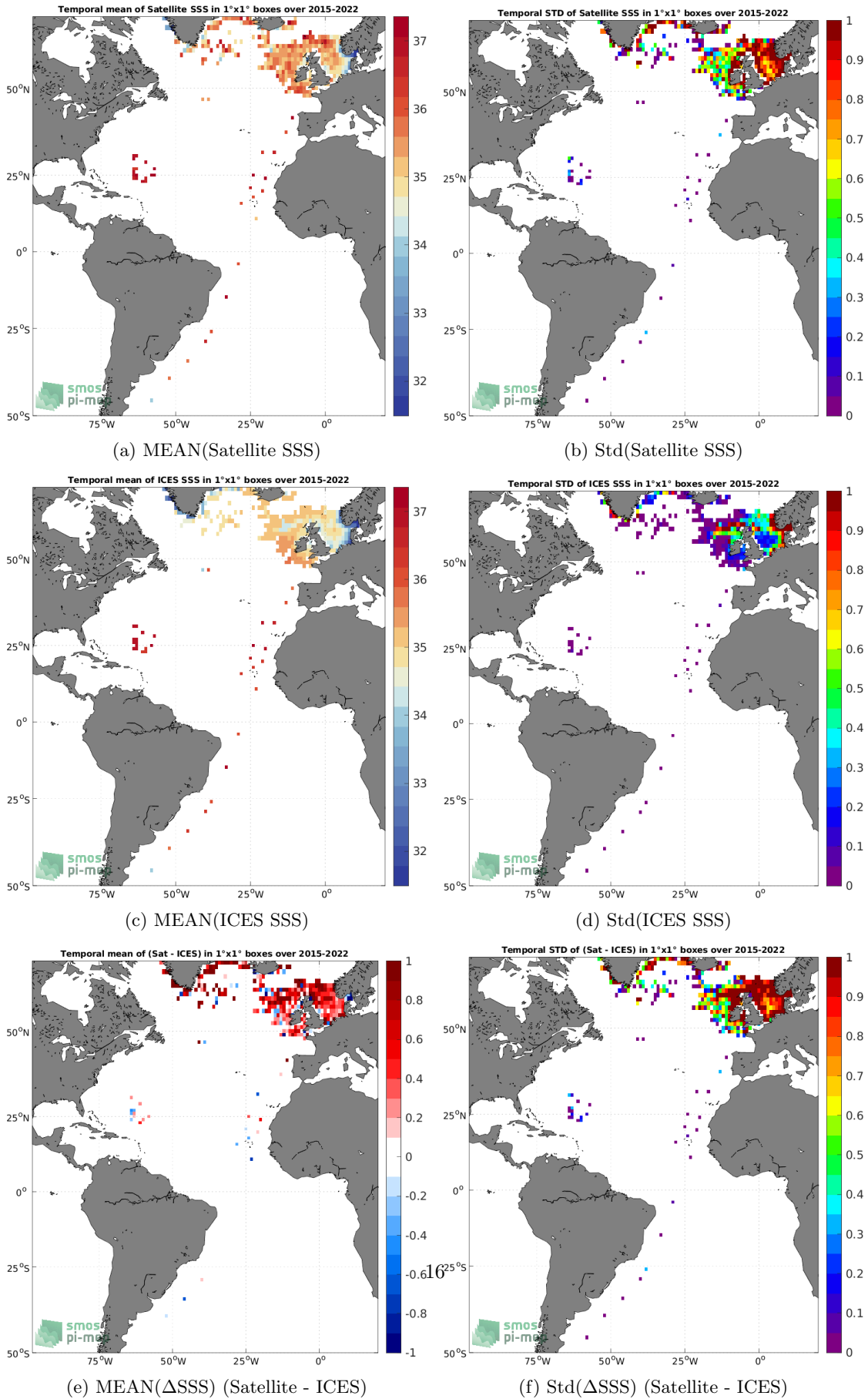
Figure 6: Temporal mean (left) and Std (right) of SSS from SMAP SSS L2 v5 (RSS) (top), ICES (middle), and of \Delta SSS (Satellite - ICES). Only match-up pairs are used to generate these maps.
