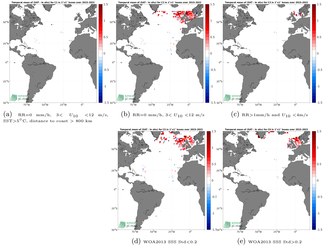
Figure 12: Temporal mean gridded over spatial boxes of size 1^\circ \times 1^\circ of \Delta SSS (SMAP SSS L2 v5 (RSS) - ICES) for 5 different subdatasets corresponding to:RR=0 mm/h, 3 < U_{10} < 12 m/s, SST >5^\circ C, distance to coast > 800 km (a), RR=0 mm/h, 3 < U_{10} < 12 m/s (b), RR >1 mm/h and U_{10} < 4 m/s (c), WOA2013 SSS Std <0.2 (d), WOA2013 SSS Std >0.2 (e).
