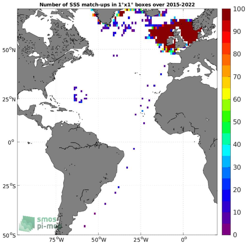
Figure 4: Number of SSS match-ups between ICES SSS and the SMAP SSS L2 v5 (RSS) SSS product for the Atlantic Ocean Pi-MEP region over 1°x1° boxes and for the full satellite product period.
