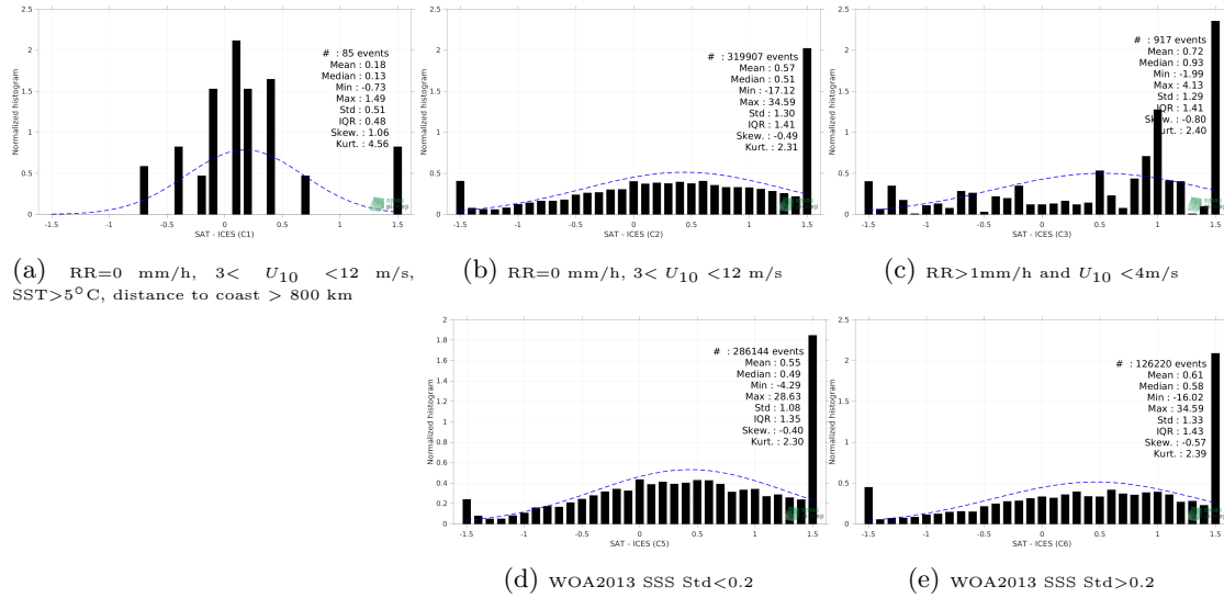
Figure 13: Normalized histogram of \Delta\text{SSS} (SMAP SSS L2 v5 (RSS) - ICES) for 5 different subdatasets corresponding to: RR=0 mm/h, 3 < U_{10} < 12 m/s, SST>5°C, distance to coast > 800 km (a), RR=0 mm/h, 3 < U_{10} < 12 m/s (b), RR>1mm/h and U_{10} < 4 m/s (c), WOA2013 SSS Std<0.2 (d), WOA2013 SSS Std>0.2 (e).
