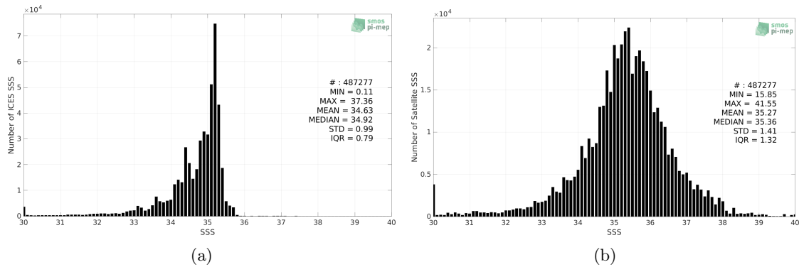
Figure 2: Histograms of SSS from ICES (a) and SMAP SSS L2 v5 (RSS) (b) considering all match-up pairs per bins of 0.1 over the Atlantic Ocean Pi-MEP region and for the full satellite product period.
