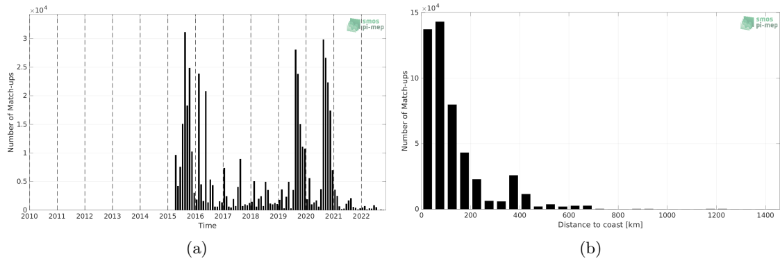
Figure 1: Number of match-ups between ICES and SMAP SSS L2 v5 (RSS) SSS as a function of time (a) and as function of the distance to coast (b) over the Atlantic Ocean Pi-MEP region and for the full satellite product period.
