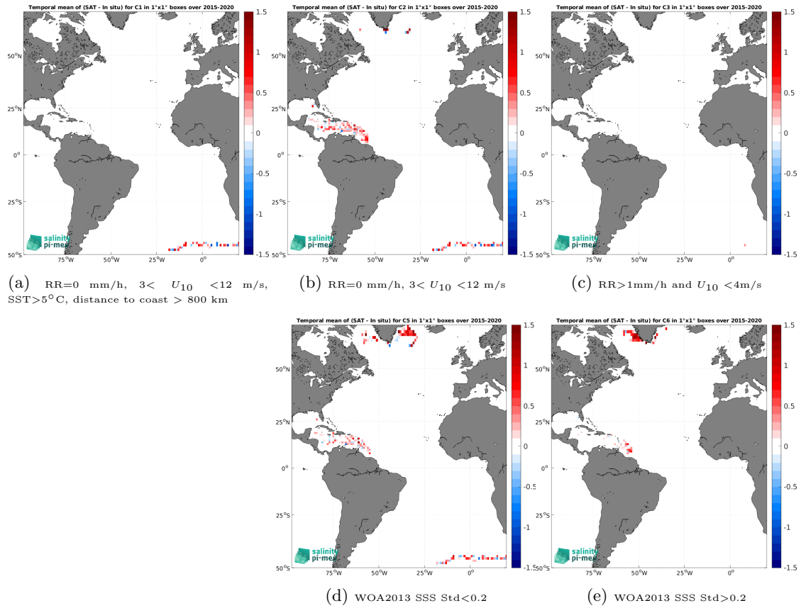
Figure 11: Temporal mean gridded over spatial boxes of size 1^\circ \times 1^\circ of \Delta SSS (SMAP SSS L2 v5 (RSS) - Surface drifters) for 5 different subdatasets corresponding to:RR=0 mm/h, 3 < U_{10} < 12 m/s, SST >5^\circ\text{C} , distance to coast > 800 km (a), RR=0 mm/h, 3 < U_{10} < 12 m/s (b), RR >1 mm/h and U_{10} < 4 m/s (c), WOA2013 SSS Std <0.2 (d), WOA2013 SSS Std >0.2 (e).
