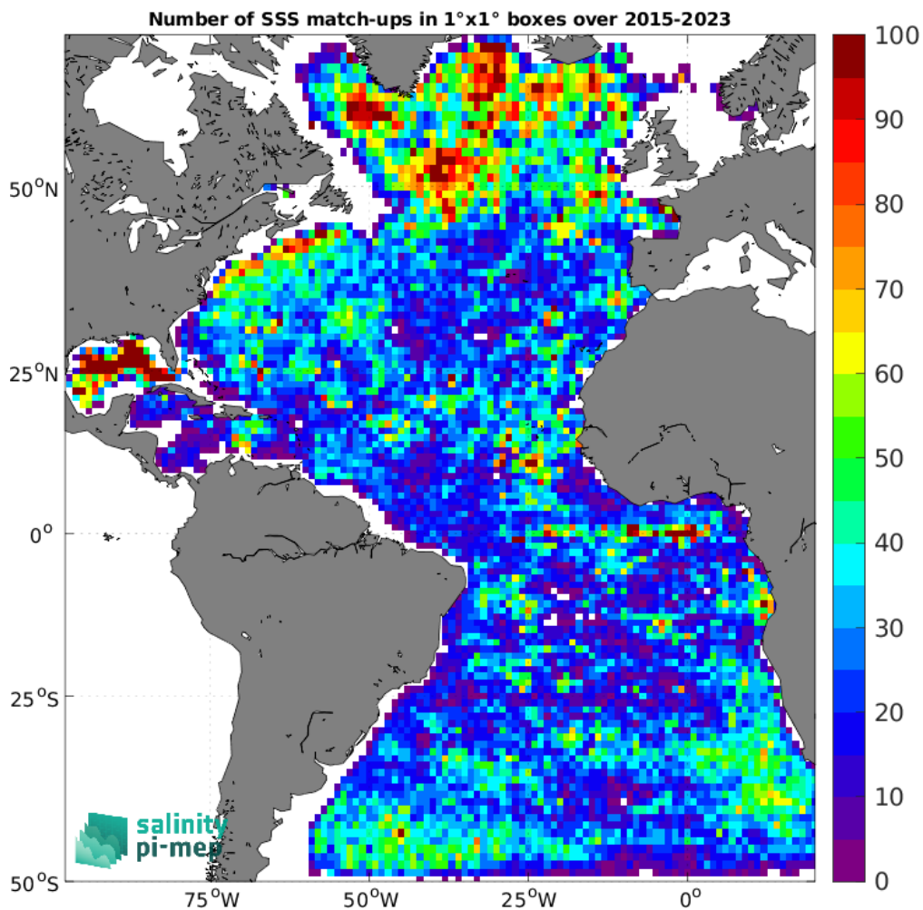
Figure 4: Number of SSS match-ups between Argo SSS and the SMAP SSS L2 v5 (RSS) SSS product for the Atlantic Ocean Pi-MEP region over 1^\circ \times 1^\circ boxes and for the full satellite product period.
