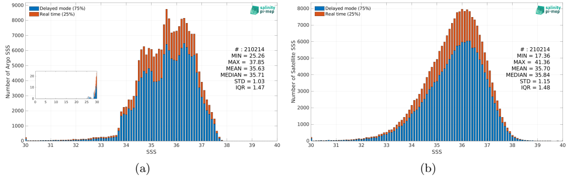
Figure 2: Histograms of SSS from Argo (a) and SMAP SSS L2 v5 (RSS) (b) considering all match-up pairs per bins of 0.1 over the Atlantic Ocean Pi-MEP region and for the full satellite product period.
