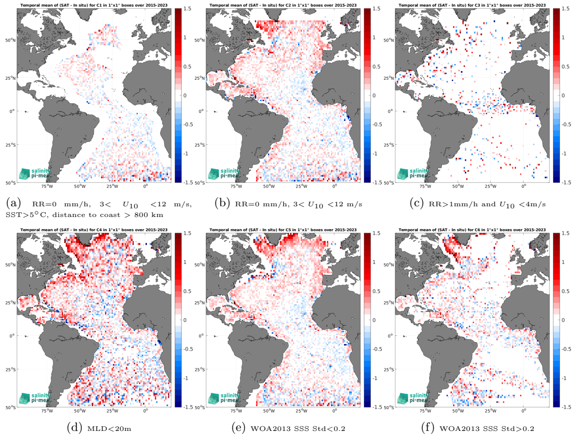
Figure 12: Temporal mean gridded over spatial boxes of size 1^\circ \times 1^\circ of \Delta SSS (SMAP SSS L2 v5 (RSS) - Argo) for 6 different subdatasets corresponding to:RR=0 mm/h, 3 < U_{10} < 12 m/s, SST >5^\circ C, distance to coast > 800 km (a), RR=0 mm/h, 3 < U_{10} < 12 m/s (b), RR >1 mm/h and U_{10} < 4 m/s (c),MLD <20 m (d),WOA2013 SSS Std <0.2 (e),WOA2013 SSS Std >0.2 (f).
