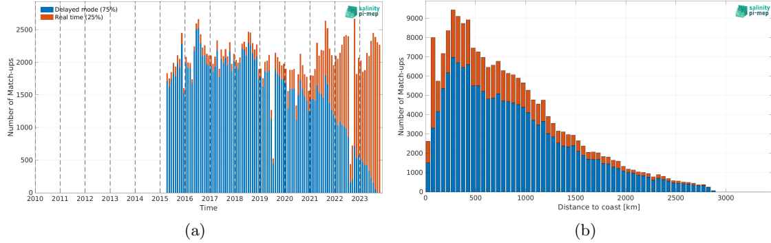
Figure 1: Number of match-ups between Argo and SMAP SSS L2 v5 (RSS) SSS as a function of time (a) and as function of the distance to coast (b) over the Atlantic Ocean Pi-MEP region and for the full satellite product period.
