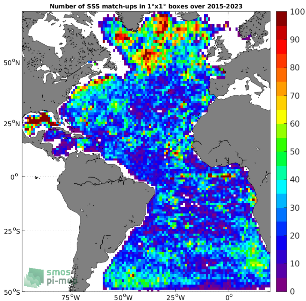
Figure 4: Number of SSS match-ups between Argo SSS and the SMAP SSS L2 v5 (RSS) SSS product for the Atlantic Ocean Pi-MEP region over 1°×1° boxes and for the full satellite product period.
