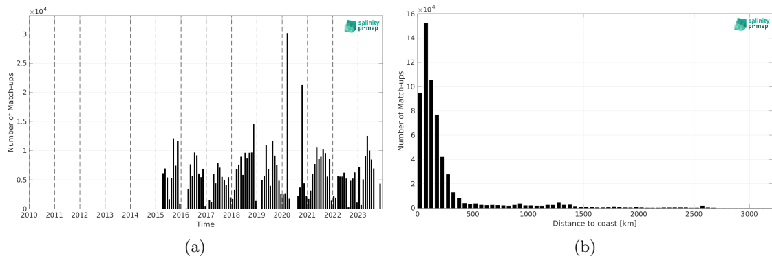
Figure 2: Number of match-ups between TSG (SAMOS) and SMAP SSS L2 v5.3 (RSS) SSS as a function of time (a) and as function of the distance to coast (b) over the Atlantic Ocean Pi-MEP region and for the full satellite product period.
