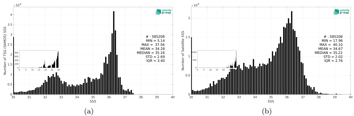
Figure 3: Histograms of SSS from TSG (SAMOS) (a) and SMAP SSS L2 v5.3 (RSS) (b) considering all match-up pairs per bins of 0.1 over the Atlantic Ocean Pi-MEP region and for the full satellite product period.
