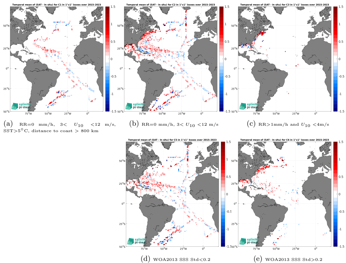
Figure 14: Temporal mean gridded over spatial boxes of size 1^\circ \times 1^\circ of \Delta\text{SSS} (SMAP SSS L2 v5.3 (RSS) - TSG (SAMOS)) for 5 different subdatasets corresponding to:RR=0 mm/h, 3 < U_{10} < 12 m/s, SST >5^\circ\text{C} , distance to coast > 800 km (a), RR=0 mm/h, 3 < U_{10} < 12 m/s (b), RR >1 mm/h and U_{10} < 4 m/s (c), WOA2013 SSS Std <0.2 (d), WOA2013 SSS Std >0.2 (e).
