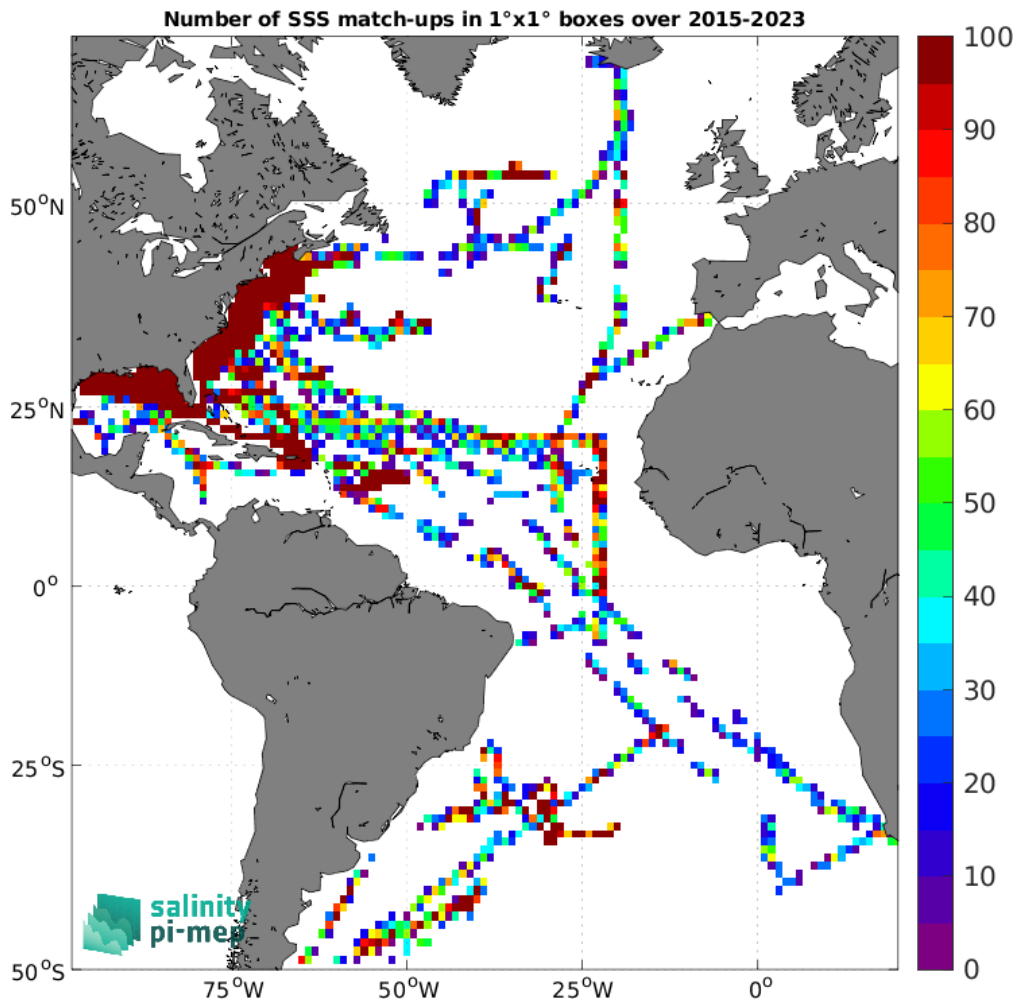
Figure 5: Number of SSS match-ups between TSG (SAMOS) SSS and the SMAP SSS L2 v5.3 (RSS) SSS product for the Atlantic Ocean Pi-MEP region over 1^\circ \times 1^\circ boxes and for the full satellite product period.
