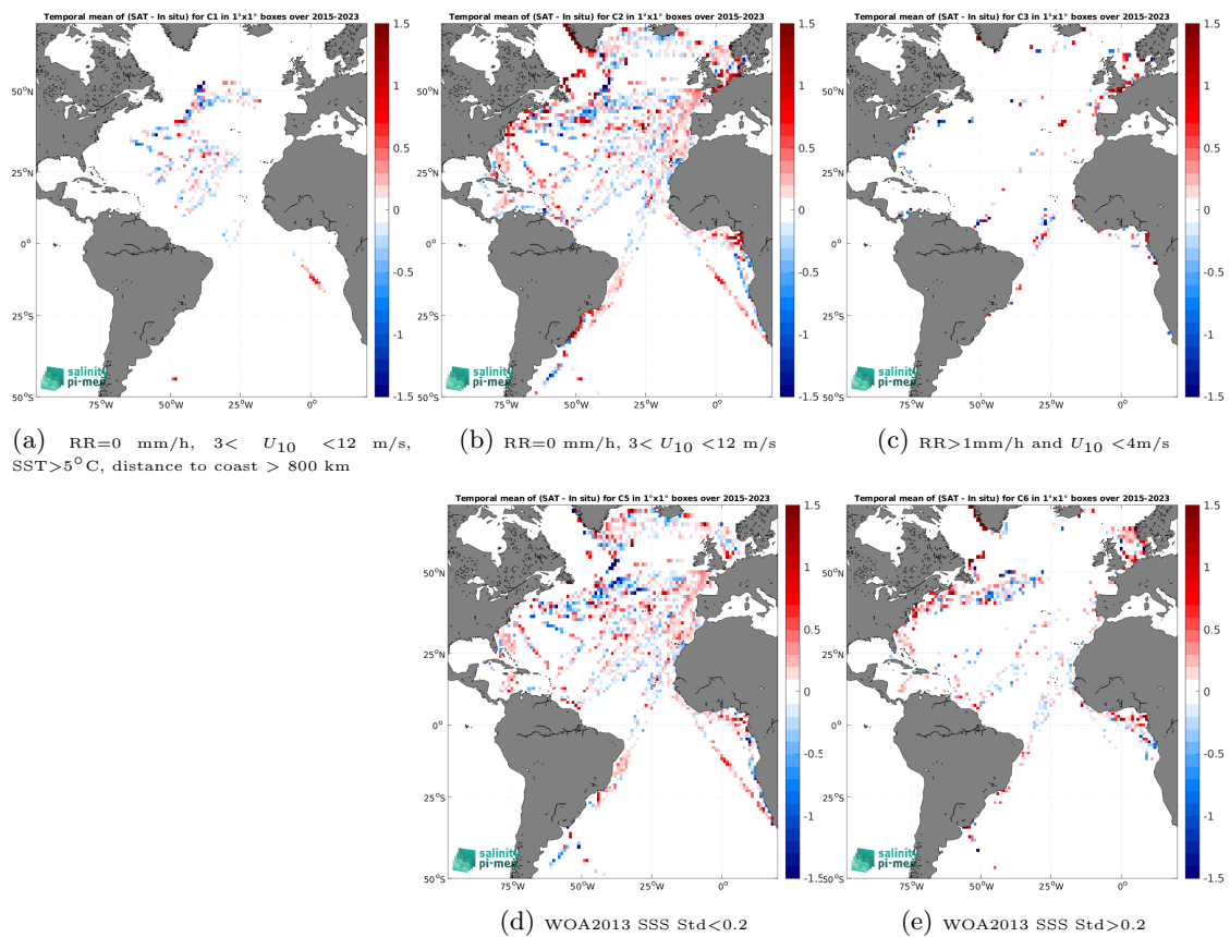
Figure 14: Temporal mean gridded over spatial boxes of size 1^\circ \times 1^\circ of \Delta\text{SSS} (SMAP SSS L2 v5.3 (RSS) - TSG (LEGOS-DM)) for 5 different subdatasets corresponding to:RR=0 mm/h, 3 < U_{10} < 12 m/s, SST >5^\circ\text{C} , distance to coast > 800 km (a), RR=0 mm/h, 3 < U_{10} < 12 m/s (b), RR >1 mm/h and U_{10} < 4 m/s (c), WOA2013 SSS Std <0.2 (d), WOA2013 SSS Std >0.2 (e).
