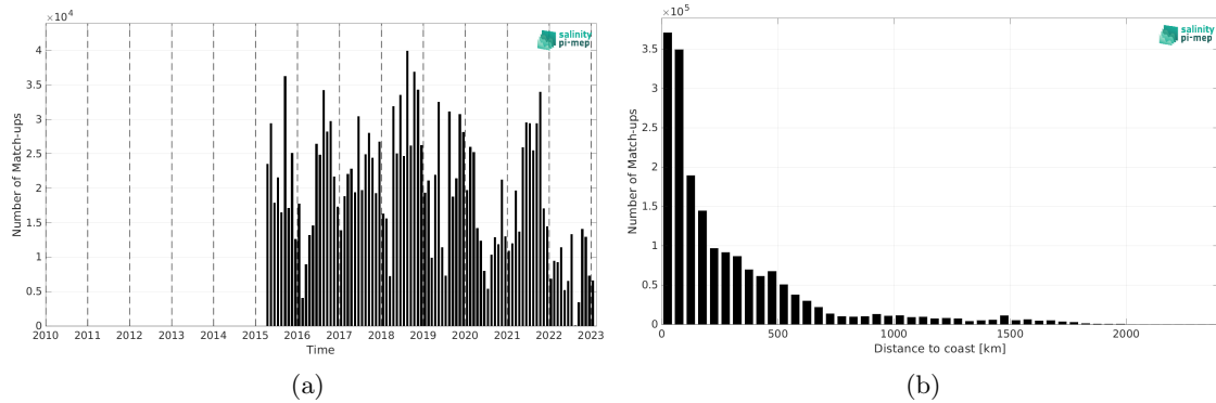
Figure 2: Number of match-ups between TSG (LEGOS-DM) and SMAP SSS L2 v5.3 (RSS) SSS as a function of time (a) and as function of the distance to coast (b) over the Atlantic Ocean Pi-MEP region and for the full satellite product period.
