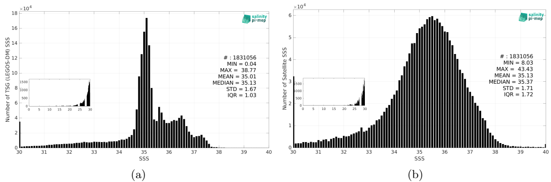
Figure 3: Histograms of SSS from TSG (LEGOS-DM) (a) and SMAP SSS L2 v5.3 (RSS) (b) considering all match-up pairs per bins of 0.1 over the Atlantic Ocean Pi-MEP region and for the full satellite product period.
