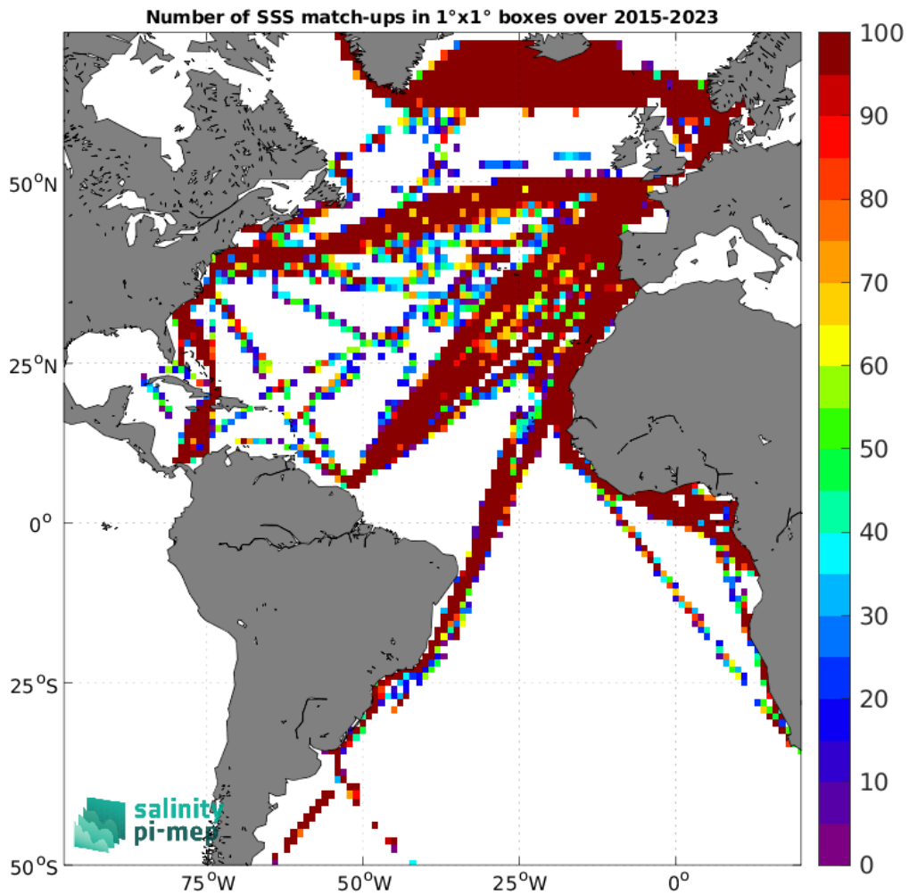
Figure 5: Number of SSS match-ups between TSG (LEGOS-DM) SSS and the SMAP SSS L2 v5.3 (RSS) SSS product for the Atlantic Ocean Pi-MEP region over 1^\circ \times 1^\circ boxes and for the full satellite product period.
