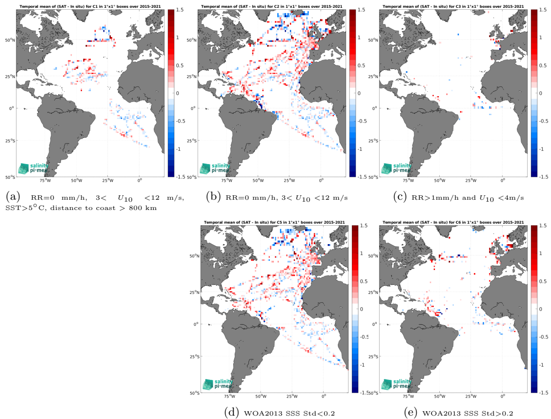
Figure 14: Temporal mean gridded over spatial boxes of size 1^\circ \times 1^\circ of \Delta\text{SSS} (SMAP SSS L2 v5.3 (RSS) - TSG (GOSUD-Research-vessel)) for 5 different subdatasets corresponding to:RR=0 mm/h, 3 < U_{10} < 12 m/s, SST>5°C, distance to coast > 800 km (a), RR=0 mm/h, 3 < U_{10} < 12 m/s (b), RR>1mm/h and U_{10} < 4 m/s (c), WOA2013 SSS Std<0.2 (d), WOA2013 SSS Std>0.2 (e).
