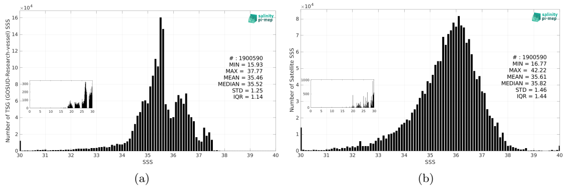
Figure 3: Histograms of SSS from TSG (GOSUD-Research-vessel) (a) and SMAP SSS L2 v5.3 (RSS) (b) considering all match-up pairs per bins of 0.1 over the Atlantic Ocean Pi-MEP region and for the full satellite product period.
