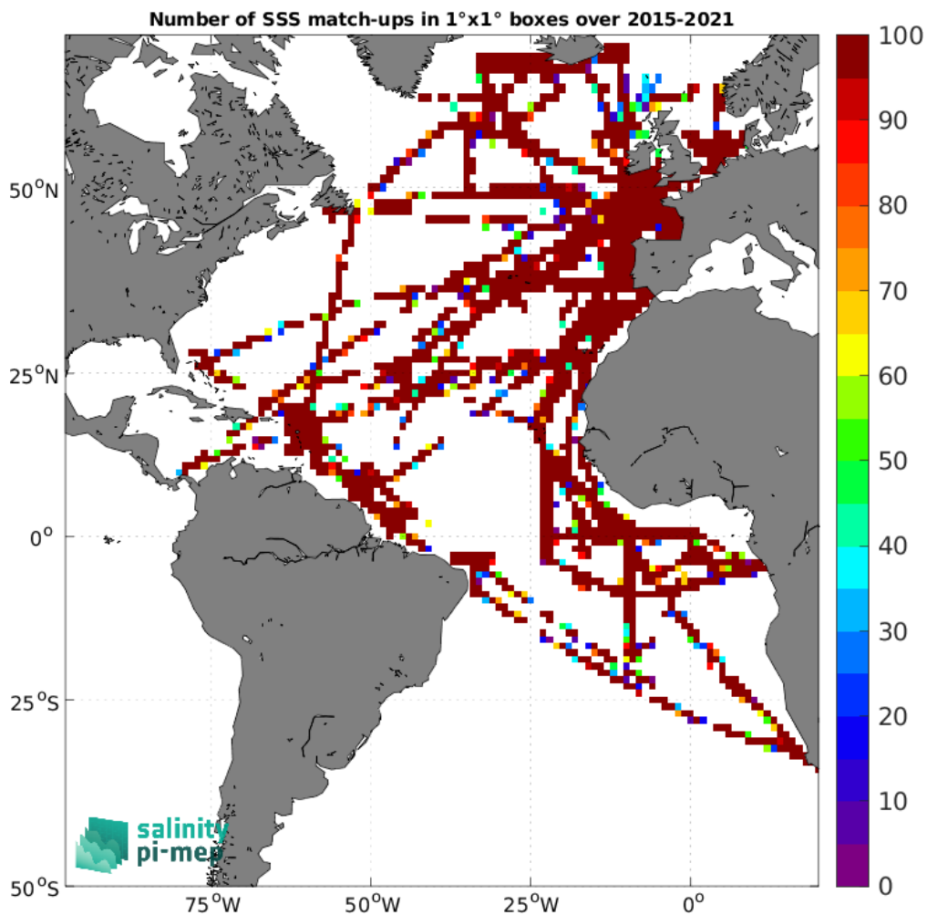
Figure 5: Number of SSS match-ups between TSG (GOSUD-Research-vessel) SSS and the SMAP SSS L2 v5.3 (RSS) SSS product for the Atlantic Ocean Pi-MEP region over 1^\circ \times 1^\circ boxes and for the full satellite product period.
