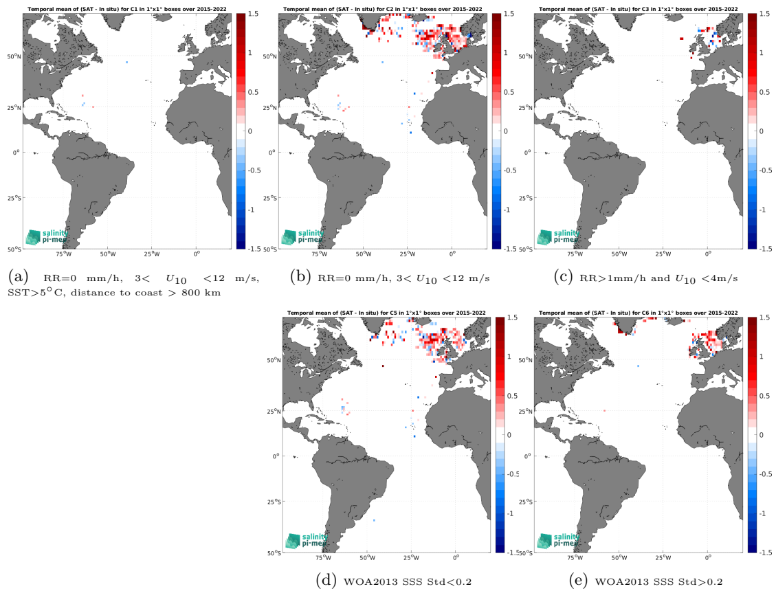
Figure 14: Temporal mean gridded over spatial boxes of size 1^\circ \times 1^\circ of \Delta\text{SSS} (SMAP SSS L2 v5.3 (RSS) - ICES) for 5 different subdatasets corresponding to:RR=0 mm/h, 3 < U_{10} < 12 m/s, SST >5^\circ\text{C} , distance to coast > 800 km (a), RR=0 mm/h, 3 < U_{10} < 12 m/s (b), RR >1 mm/h and U_{10} < 4 m/s (c), WOA2013 SSS Std <0.2 (d), WOA2013 SSS Std >0.2 (e).
