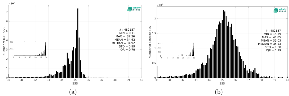
Figure 3: Histograms of SSS from ICES (a) and SMAP SSS L2 v5.3 (RSS) (b) considering all match-up pairs per bins of 0.1 over the Atlantic Ocean Pi-MEP region and for the full satellite product period.
