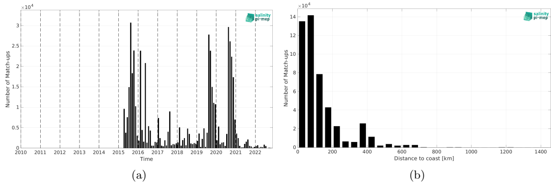
Figure 2: Number of match-ups between ICES and SMAP SSS L2 v5.3 (RSS) SSS as a function of time (a) and as function of the distance to coast (b) over the Atlantic Ocean Pi-MEP region and for the full satellite product period.
