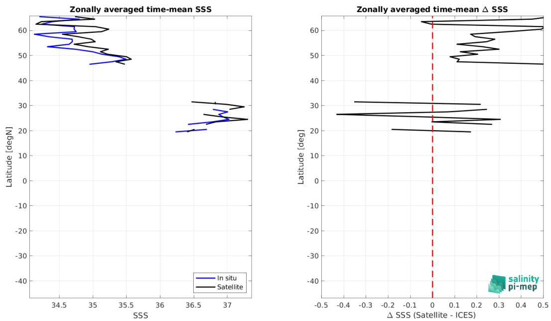
Figure 9: Left panel: Zonal mean SSS from SMAP SSS L2 v5.3 (RSS) satellite product (black) and from ICES (blue). Right panel: Zonal mean of \Delta SSS (Satellite - ICES) for all the collected Pi-MEP match-up pairs estimated over the full satellite product period.
