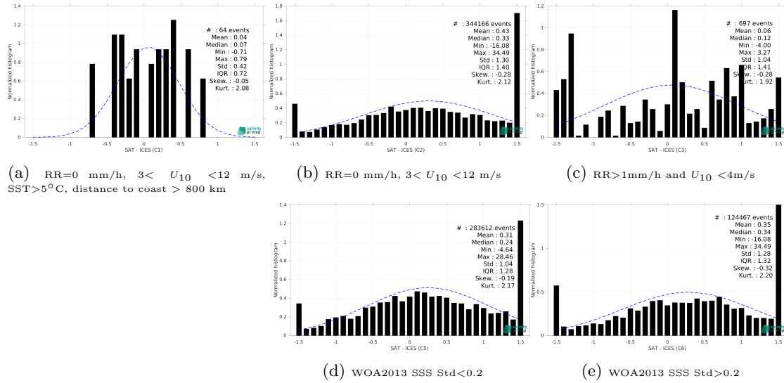
Figure 15: Normalized histogram of \Delta SSS (SMAP SSS L2 v5.3 (RSS) - ICES) for 5 different subdatasets corresponding to: RR=0 mm/h, 3 < U_{10} < 12 m/s, SST>5°C, distance to coast > 800 km (a), RR=0 mm/h, 3 < U_{10} < 12 m/s (b), RR>1mm/h and U_{10} < 4 m/s (c), WOA2013 SSS Std<0.2 (d), WOA2013 SSS Std>0.2 (e).
