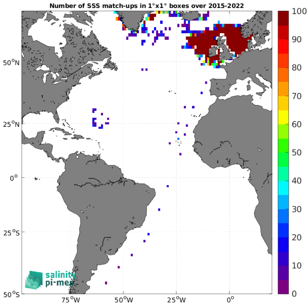
Figure 5: Number of SSS match-ups between ICES SSS and the SMAP SSS L2 v5.3 (RSS) SSS product for the Atlantic Ocean Pi-MEP region over 1^{\circ} \times 1^{\circ} boxes and for the full satellite product period.
