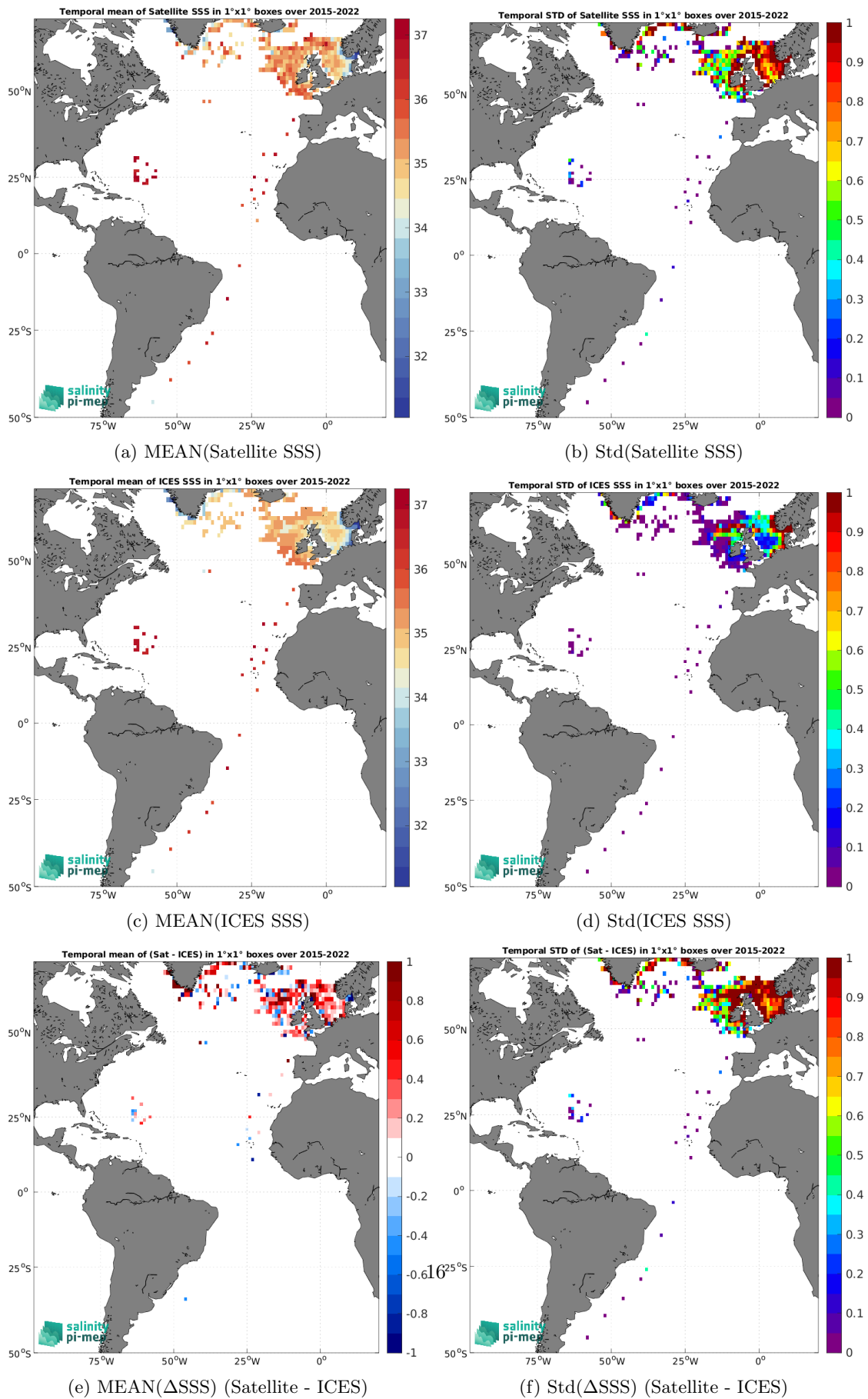
Figure 7: Temporal mean (left) and Std (right) of SSS from SMAP SSS L2 v5.3 (RSS) (top), ICES (middle), and of \Delta SSS (Satellite - ICES). Only match-up pairs are used to generate these maps.
