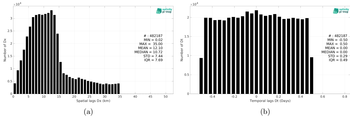
Figure 6: Histograms of the spatial (a) and temporal (b) lags between the location/time of the ICES measurement and the date of the corresponding SMAP SSS L2 v5.3 (RSS) SSS pixel.
