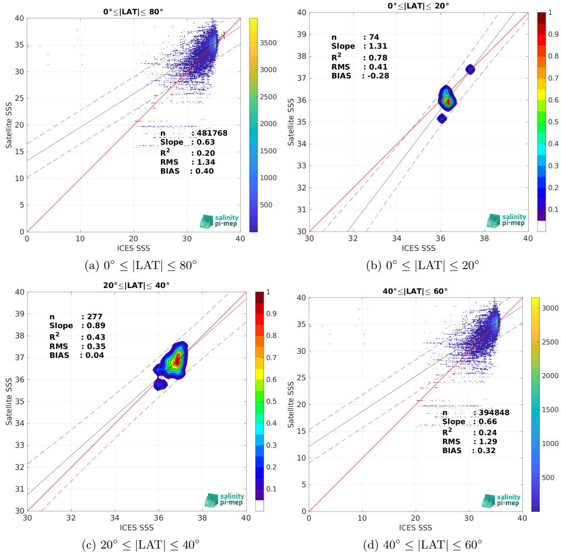
Figure 10: Contour maps of the concentration of SMAP SSS L2 v5.3 (RSS) SSS (y-axis) versus ICES SSS (x-axis) at match-up pairs for different latitude bands. For each plot, the red line shows x=y . The black thin and dashed lines indicate a linear fit through the data cloud and the \pm 95\% confidence levels, respectively. The number match-up pairs n , the slope and R^2 coefficient of the linear fit, the root mean square (RMS) and the mean bias between satellite and in situ data are indicated for each latitude band in each plots.
