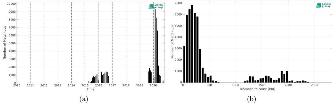
Figure 2: Number of match-ups between Surface drifters and SMAP SSS L2 v5.3 (RSS) SSS as a function of time (a) and as function of the distance to coast (b) over the Atlantic Ocean Pi-MEP region and for the full satellite product period.
