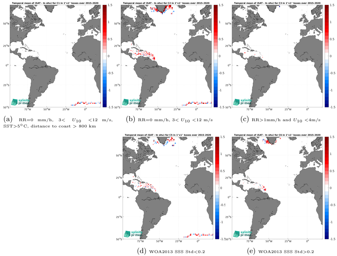
Figure 13: Temporal mean gridded over spatial boxes of size 1^\circ \times 1^\circ of \Delta SSS (SMAP SSS L2 v5.3 (RSS) - Surface drifters) for 5 different subdatasets corresponding to:RR=0 mm/h, 3 < U_{10} < 12 m/s, SST >5^\circ\text{C} , distance to coast > 800 km (a), RR=0 mm/h, 3 < U_{10} < 12 m/s (b), RR >1 mm/h and U_{10} < 4 m/s (c), WOA2013 SSS Std <0.2 (d), WOA2013 SSS Std >0.2 (e).
