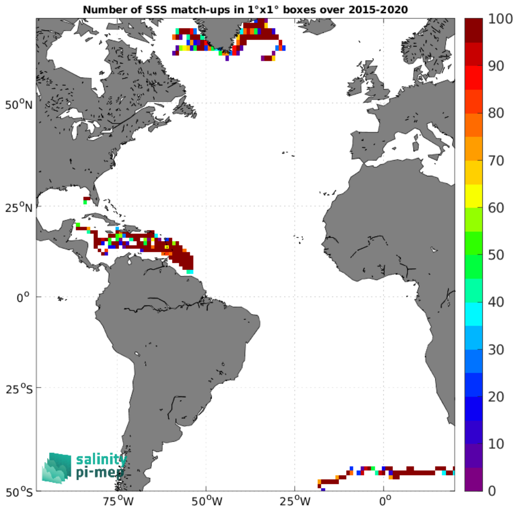
Figure 4: Number of SSS match-ups between Surface drifters SSS and the SMAP SSS L2 v5.3 (RSS) SSS product for the Atlantic Ocean Pi-MEP region over 1^{\circ} \times 1^{\circ} boxes and for the full satellite product period.
