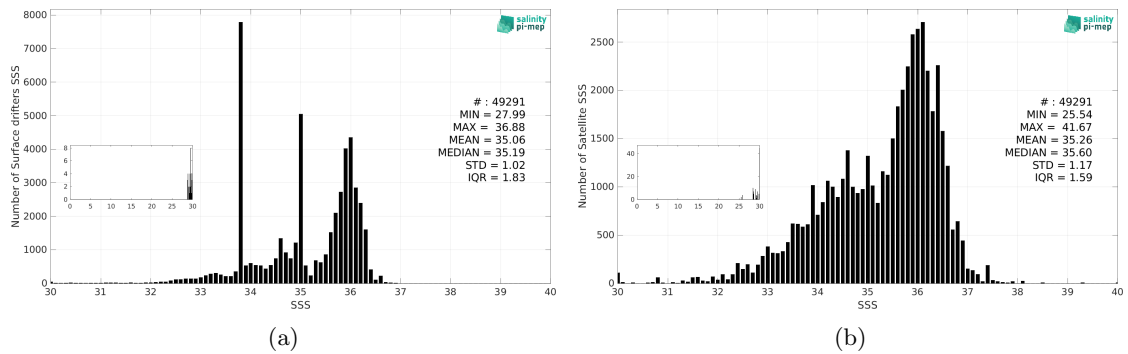
Figure 3: Histograms of SSS from Surface drifters (a) and SMAP SSS L2 v5.3 (RSS) (b) considering all match-up pairs per bins of 0.1 over the Atlantic Ocean Pi-MEP region and for the full satellite product period.
