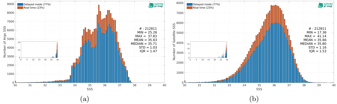
Figure 3: Histograms of SSS from Argo (a) and SMAP SSS L2 v5.3 (RSS) (b) considering all match-up pairs per bins of 0.1 over the Atlantic Ocean Pi-MEP region and for the full satellite product period.
