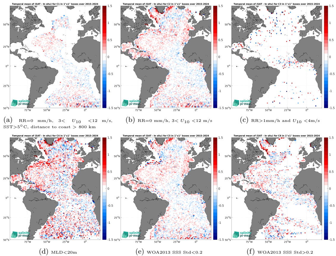
Figure 14: Temporal mean gridded over spatial boxes of size 1^\circ \times 1^\circ of \Delta SSS (SMAP SSS L2 v5.3 (RSS) - Argo) for 6 different subdatasets corresponding to:RR=0 mm/h, 3 < U_{10} < 12 m/s, SST > 5^\circ\text{C} , distance to coast > 800 km (a), RR=0 mm/h, 3 < U_{10} < 12 m/s (b), RR > 1 mm/h and U_{10} < 4 m/s (c),MLD < 20 m (d),WOA2013 SSS Std < 0.2 (e),WOA2013 SSS Std > 0.2 (f).
