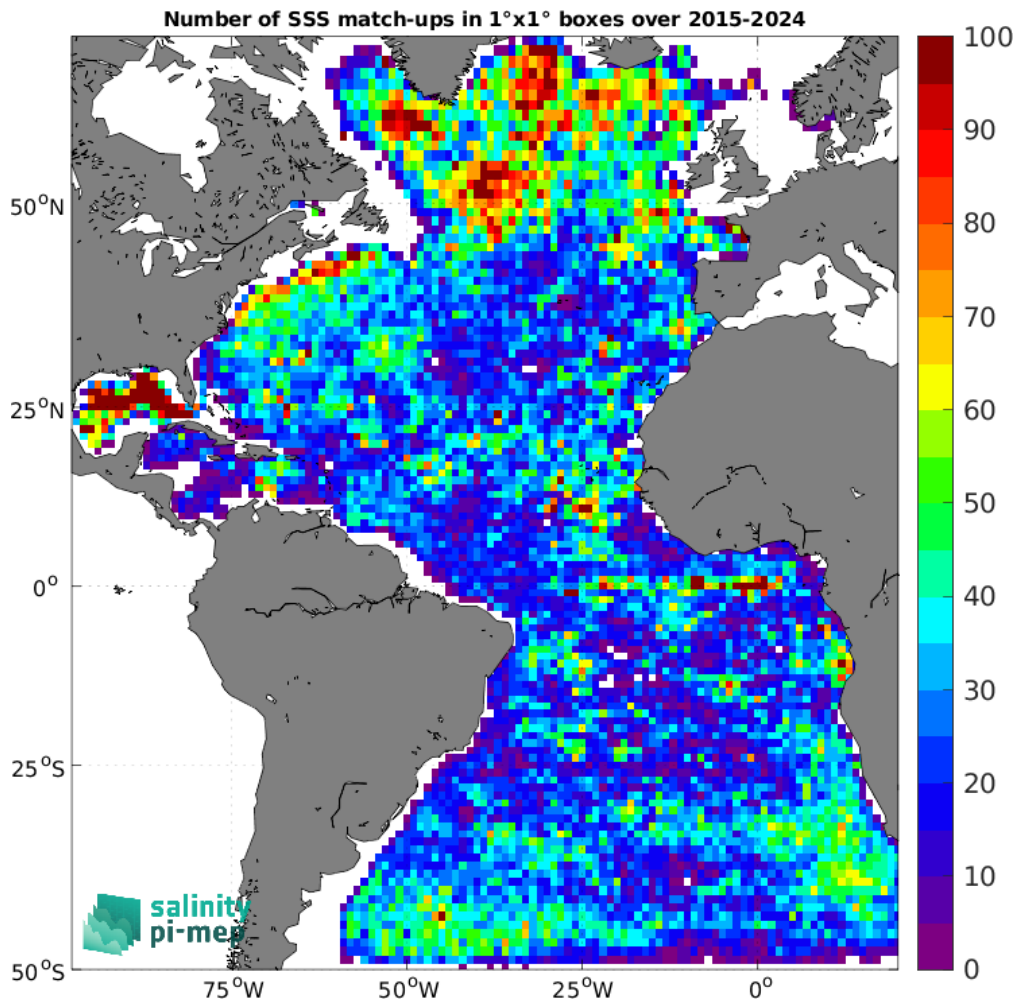
Figure 5: Number of SSS match-ups between Argo SSS and the SMAP SSS L2 v5.3 (RSS) SSS product for the Atlantic Ocean Pi-MEP region over 1^\circ \times 1^\circ boxes and for the full satellite product period.
