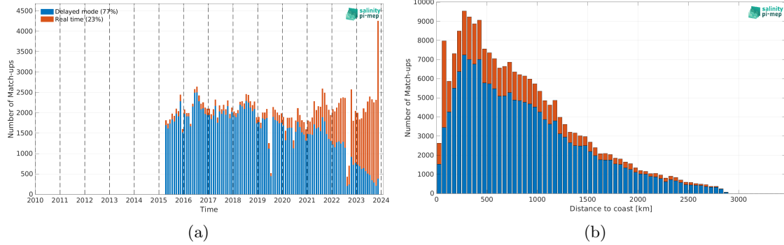
Figure 2: Number of match-ups between Argo and SMAP SSS L2 v5.3 (RSS) SSS as a function of time (a) and as function of the distance to coast (b) over the Atlantic Ocean Pi-MEP region and for the full satellite product period.
