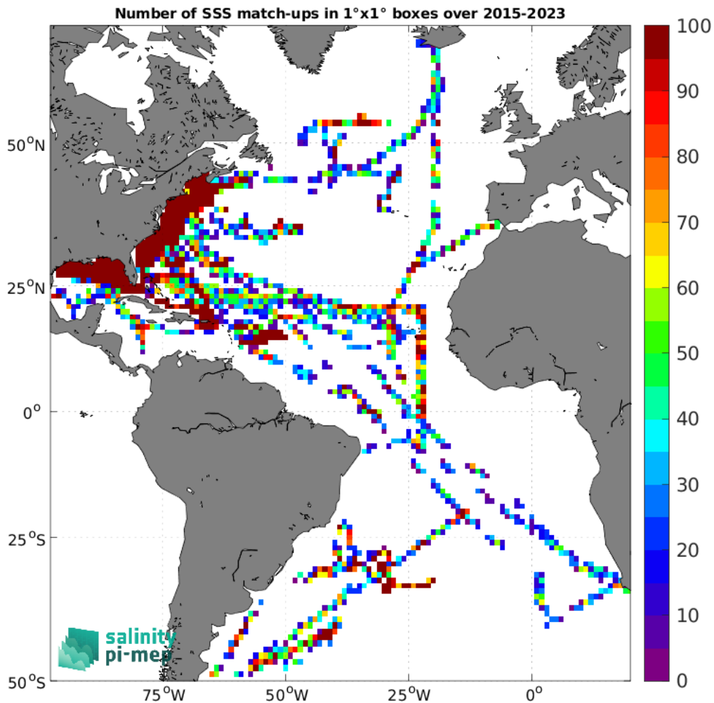
Figure 5: Number of SSS match-ups between TSG (SAMOS) SSS and the SMAP SSS L2 v5.3 - 40 km (RSS) SSS product for the Atlantic Ocean Pi-MEP region over 1^\circ \times 1^\circ boxes and for the full satellite product period.
