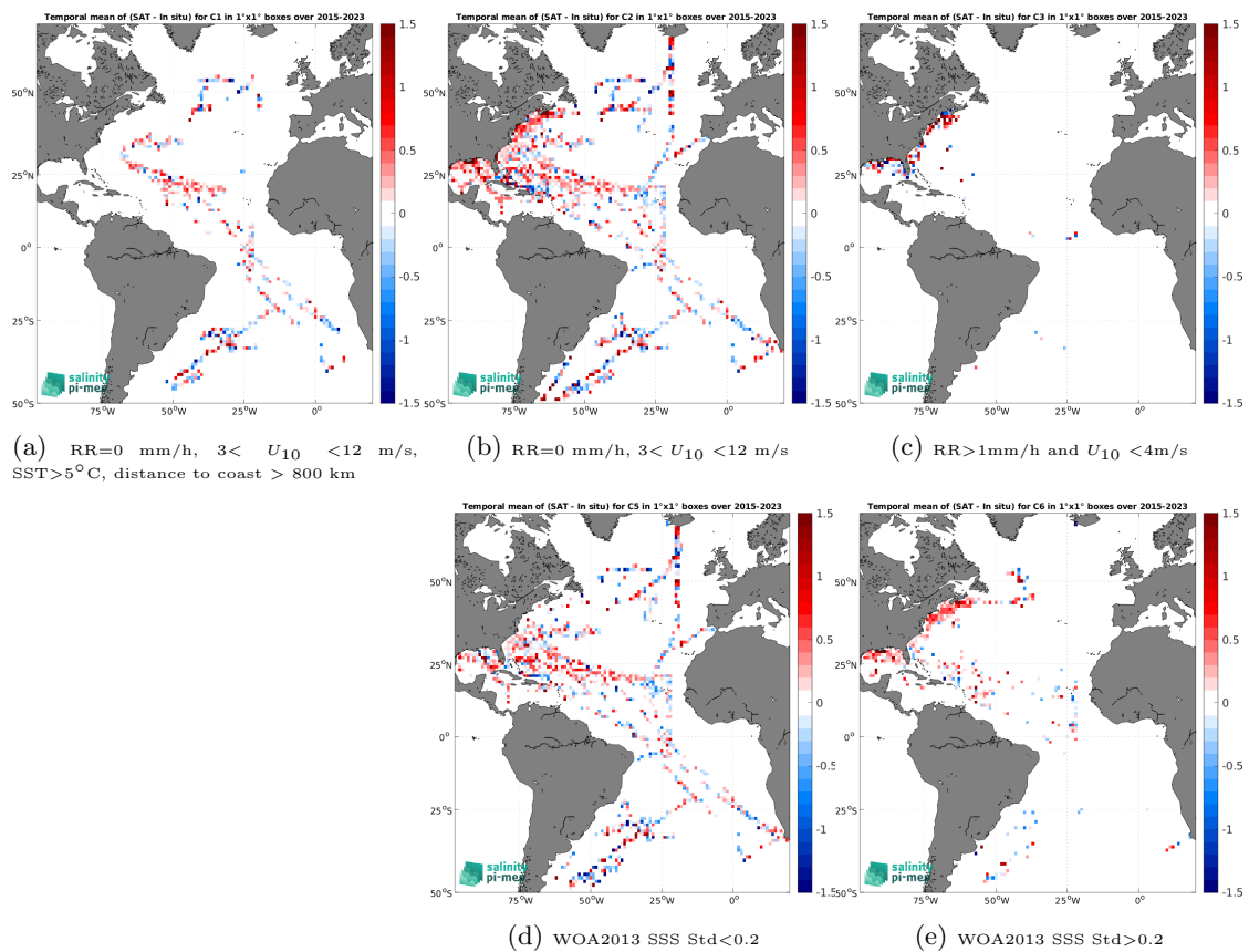
Figure 14: Temporal mean gridded over spatial boxes of size 1^\circ \times 1^\circ of \Delta\text{SSS} (SMAP SSS L2 v5.3 - 40 km (RSS) - TSG (SAMOS)) for 5 different subdatasets corresponding to:RR=0 mm/h, 3 < U_{10} < 12 m/s, SST>5°C, distance to coast > 800 km (a), RR=0 mm/h, 3 < U_{10} < 12 m/s (b), RR>1mm/h and U_{10} < 4 m/s (c), WOA2013 SSS Std<0.2 (d), WOA2013 SSS Std>0.2 (e).
