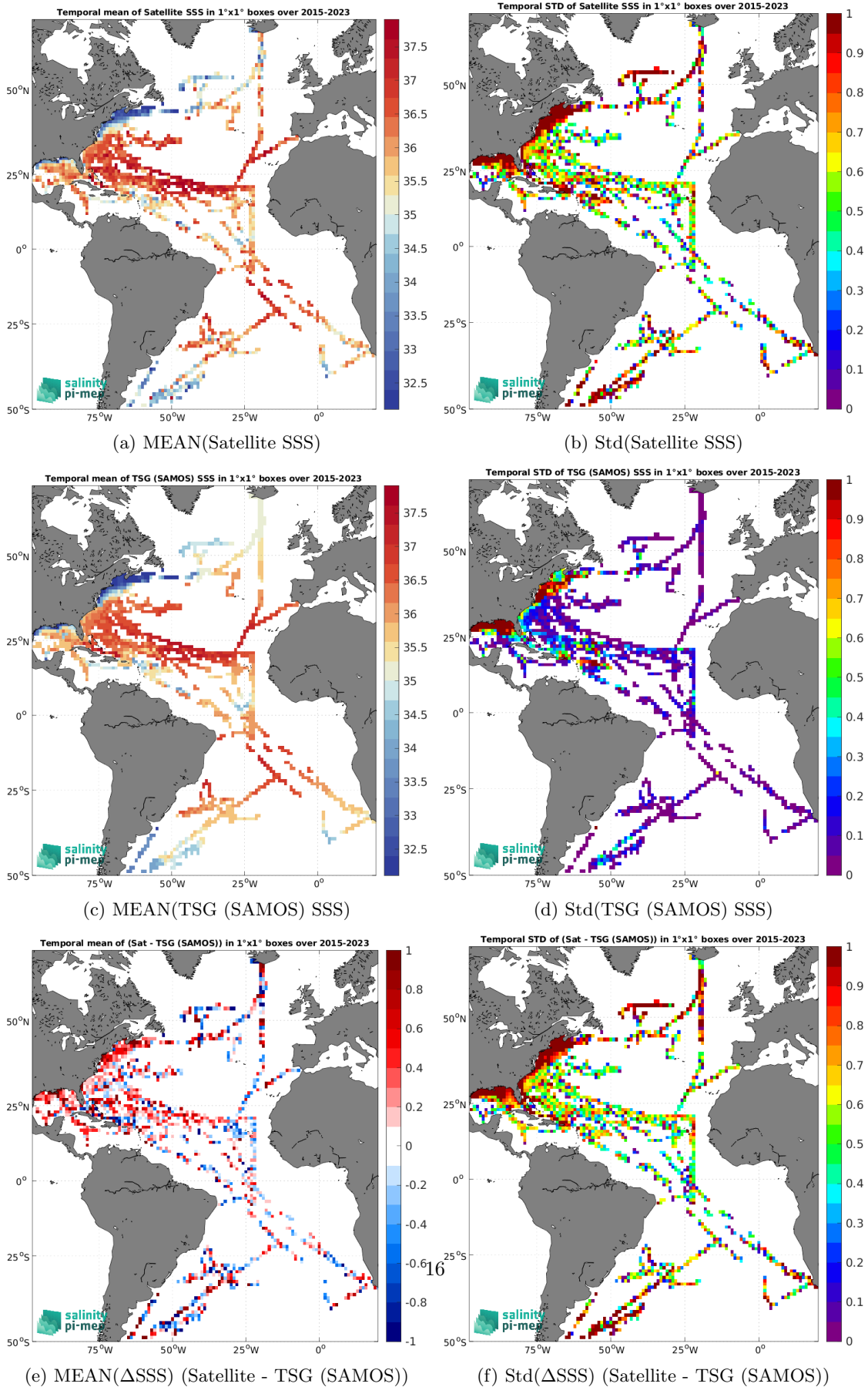
Figure 7: Temporal mean (left) and Std (right) of SSS from SMAP SSS L2 v5.3 - 40 km (RSS) (top), TSG (SAMOS) (middle), and of \Delta SSS (Satellite - TSG (SAMOS)). Only match-up pairs are used to generate these maps.
