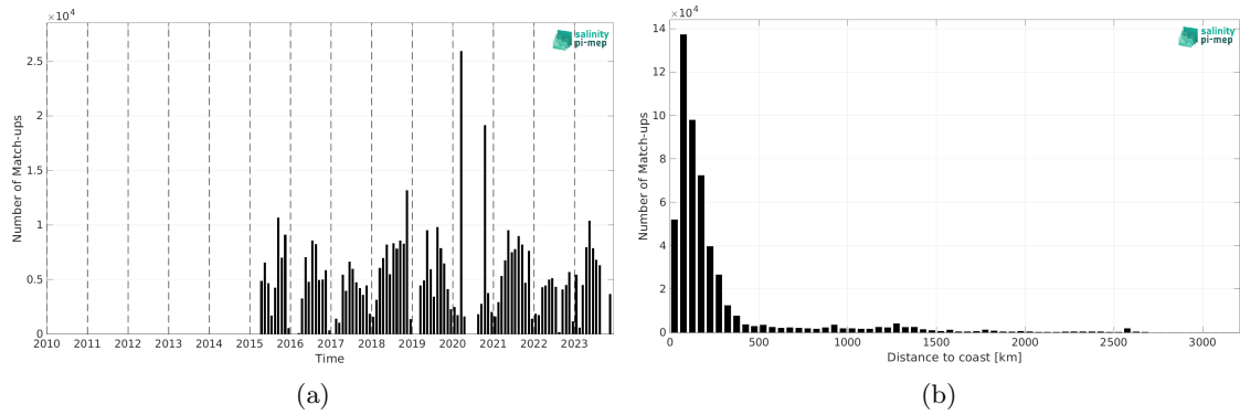
Figure 2: Number of match-ups between TSG (SAMOS) and SMAP SSS L2 v5.3 - 40 km (RSS) SSS as a function of time (a) and as function of the distance to coast (b) over the Atlantic Ocean Pi-MEP region and for the full satellite product period.
