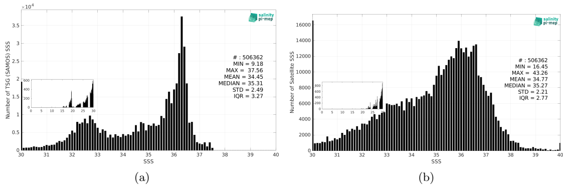
Figure 3: Histograms of SSS from TSG (SAMOS) (a) and SMAP SSS L2 v5.3 - 40 km (RSS) (b) considering all match-up pairs per bins of 0.1 over the Atlantic Ocean Pi-MEP region and for the full satellite product period.
