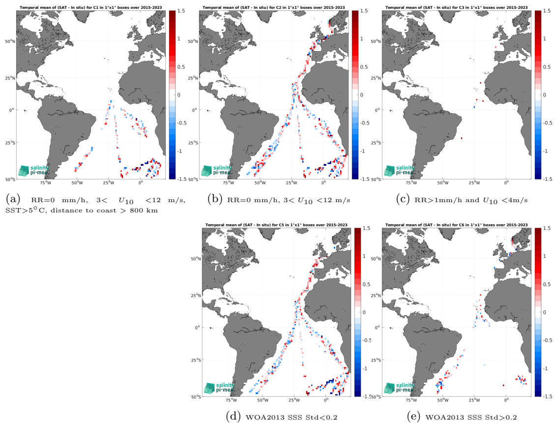
Figure 14: Temporal mean gridded over spatial boxes of size 1^\circ \times 1^\circ of \Delta\text{SSS} (SMAP SSS L2 v5.3 - 40 km (RSS) - TSG (Polarstern)) for 5 different subdatasets corresponding to:RR=0 mm/h, 3 < U_{10} < 12 m/s, SST>5°C, distance to coast > 800 km (a), RR=0 mm/h, 3 < U_{10} < 12 m/s (b), RR>1mm/h and U_{10} < 4 m/s (c), WOA2013 SSS Std<0.2 (d), WOA2013 SSS Std>0.2 (e).
