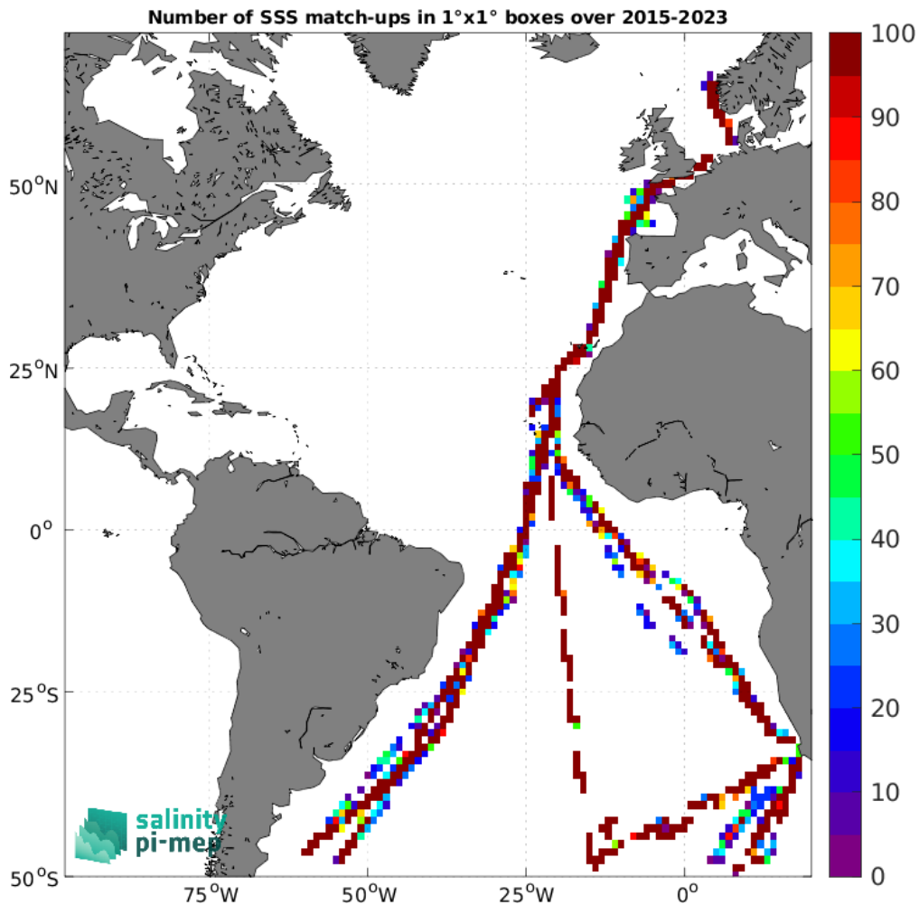
Figure 5: Number of SSS match-ups between TSG (Polarstern) SSS and the SMAP SSS L2 v5.3 - 40 km (RSS) SSS product for the Atlantic Ocean Pi-MEP region over 1°×1° boxes and for the full satellite product period.
