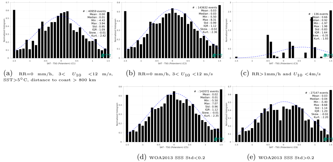
Figure 15: Normalized histogram of \Delta SSS (SMAP SSS L2 v5.3 - 40 km (RSS) - TSG (Polarstern)) for 5 different subdatasets corresponding to: RR=0 mm/h, 3 < U_{10} < 12 m/s, SST > 5°C, distance to coast > 800 km (a), RR=0 mm/h, 3 < U_{10} < 12 m/s (b), RR > 1mm/h and U_{10} < 4 m/s (c), WOA2013 SSS Std < 0.2 (d), WOA2013 SSS Std > 0.2 (e).
