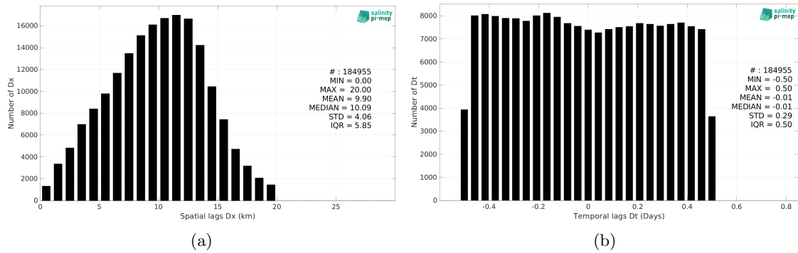
Figure 6: Histograms of the spatial (a) and temporal (b) lags between the location/time of the TSG (Polarstern) measurement and the date of the corresponding SMAP SSS L2 v5.3 - 40 km (RSS) SSS pixel.
