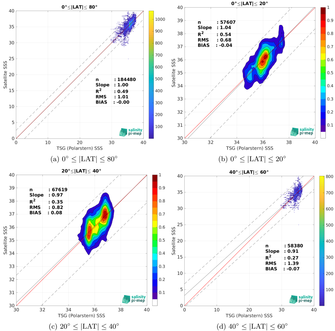
Figure 10: Contour maps of the concentration of SMAP SSS L2 v5.3 - 40 km (RSS) SSS (y-axis) versus TSG (Polarstern) SSS (x-axis) at match-up pairs for different latitude bands. For each plot, the red line shows x=y . The black thin and dashed lines indicate a linear fit through the data cloud and the \pm 95\% confidence levels, respectively. The number match-up pairs n , the slope and R^2 coefficient of the linear fit, the root mean square (RMS) and the mean bias between satellite and in situ data are indicated for each latitude band in each plots.
