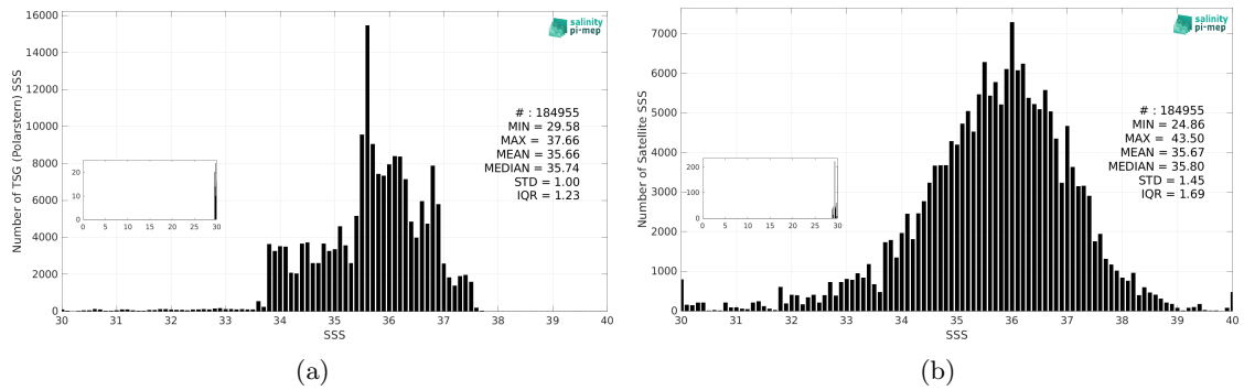
Figure 3: Histograms of SSS from TSG (Polarstern) (a) and SMAP SSS L2 v5.3 - 40 km (RSS) (b) considering all match-up pairs per bins of 0.1 over the Atlantic Ocean Pi-MEP region and for the full satellite product period.
