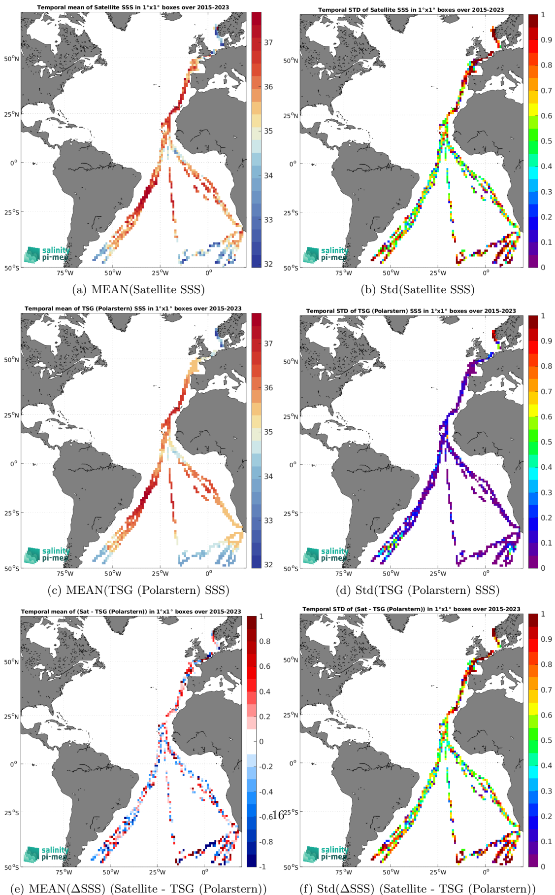
Figure 7: Temporal mean (left) and Std (right) of SSS from SMAP SSS L2 v5.3 - 40 km (RSS) (top), TSG (Polarstern) (middle), and of \Delta SSS (Satellite - TSG (Polarstern)). Only match-up pairs are used to generate these maps.
