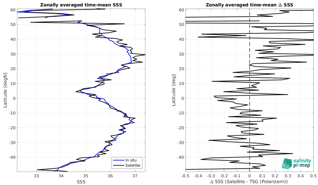
Figure 9: Left panel: Zonal mean SSS from SMAP SSS L2 v5.3 - 40 km (RSS) satellite product (black) and from TSG (Polarstern) (blue). Right panel: Zonal mean of \Delta SSS (Satellite - TSG (Polarstern)) for all the collected Pi-MEP match-up pairs estimated over the full satellite product period.
