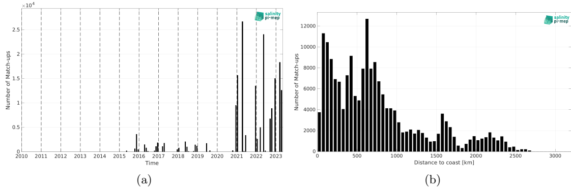
Figure 2: Number of match-ups between TSG (Polarstern) and SMAP SSS L2 v5.3 - 40 km (RSS) SSS as a function of time (a) and as function of the distance to coast (b) over the Atlantic Ocean Pi-MEP region and for the full satellite product period.
