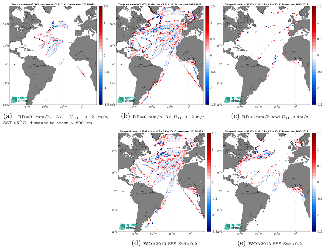
Figure 14: Temporal mean gridded over spatial boxes of size 1^\circ \times 1^\circ of \Delta\text{SSS} (SMAP SSS L2 v5.3 - 40 km (RSS) - TSG (LEGOS-DM)) for 5 different subdatasets corresponding to:RR=0 mm/h, 3 < U_{10} < 12 m/s, SST>5°C, distance to coast > 800 km (a), RR=0 mm/h, 3 < U_{10} < 12 m/s (b), RR>1mm/h and U_{10} < 4 m/s (c), WOA2013 SSS Std<0.2 (d), WOA2013 SSS Std>0.2 (e).
