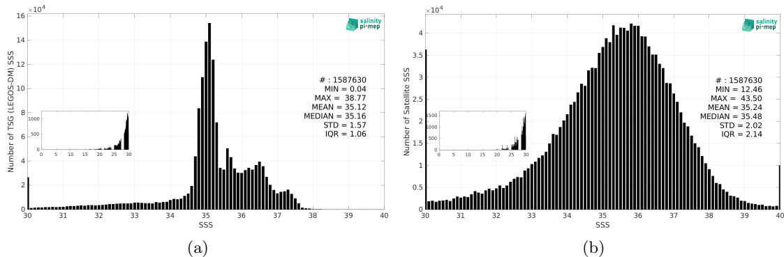
Figure 3: Histograms of SSS from TSG (LEGOS-DM) (a) and SMAP SSS L2 v5.3 - 40 km (RSS) (b) considering all match-up pairs per bins of 0.1 over the Atlantic Ocean Pi-MEP region and for the full satellite product period.
