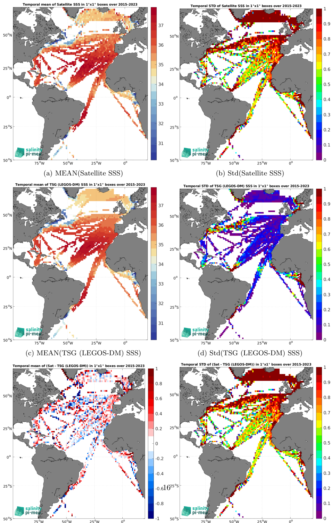
Figure 7: Temporal mean (left) and Std (right) of SSS from SMAP SSS L2 v5.3 - 40 km (RSS) (top), TSG (LEGOS-DM) (middle), and of \Delta SSS (Satellite - TSG (LEGOS-DM)). Only match-pairs are used to generate these maps.
