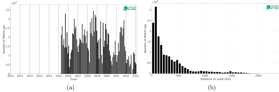
Figure 2: Number of match-ups between TSG (LEGOS-DM) and SMAP SSS L2 v5.3 - 40 km (RSS) SSS as a function of time (a) and as function of the distance to coast (b) over the Atlantic Ocean Pi-MEP region and for the full satellite product period.
