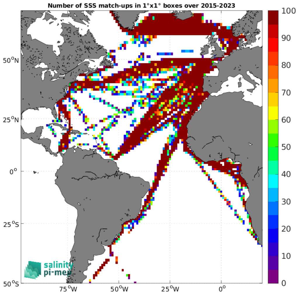
Figure 5: Number of SSS match-ups between TSG (LEGOS-DM) SSS and the SMAP SSS L2 v5.3 - 40 km (RSS) SSS product for the Atlantic Ocean Pi-MEP region over 1^\circ \times 1^\circ boxes and for the full satellite product period.
