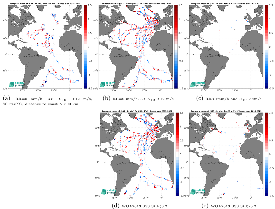
Figure 14: Temporal mean gridded over spatial boxes of size 1^\circ \times 1^\circ of \Delta\text{SSS} (SMAP SSS L2 v5.3 - 40 km (RSS) - TSG (GOSUD-Sailing-ship)) for 5 different subdatasets corresponding to:RR=0 mm/h, 3 < U_{10} < 12 m/s, SST >5^\circ\text{C} , distance to coast > 800 km (a), RR=0 mm/h, 3 < U_{10} < 12 m/s (b), RR >1 mm/h and U_{10} < 4 m/s (c), WOA2013 SSS Std <0.2 (d), WOA2013 SSS Std >0.2 (e).
