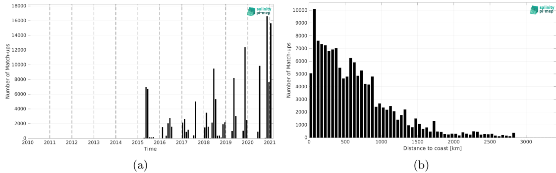
Figure 2: Number of match-ups between TSG (GOSUD-Sailing-ship) and SMAP SSS L2 v5.3 - 40 km (RSS) SSS as a function of time (a) and as function of the distance to coast (b) over the Atlantic Ocean Pi-MEP region and for the full satellite product period.
