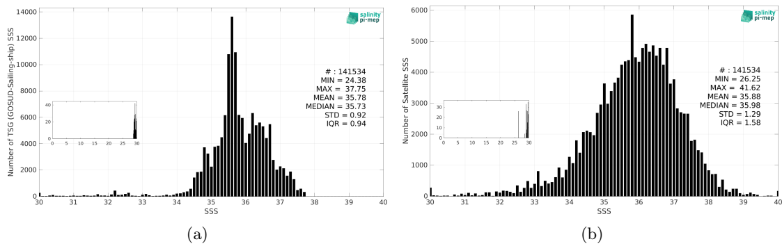
Figure 3: Histograms of SSS from TSG (GOSUD-Sailing-ship) (a) and SMAP SSS L2 v5.3 - 40 km (RSS) (b) considering all match-up pairs per bins of 0.1 over the Atlantic Ocean Pi-MEP region and for the full satellite product period.
