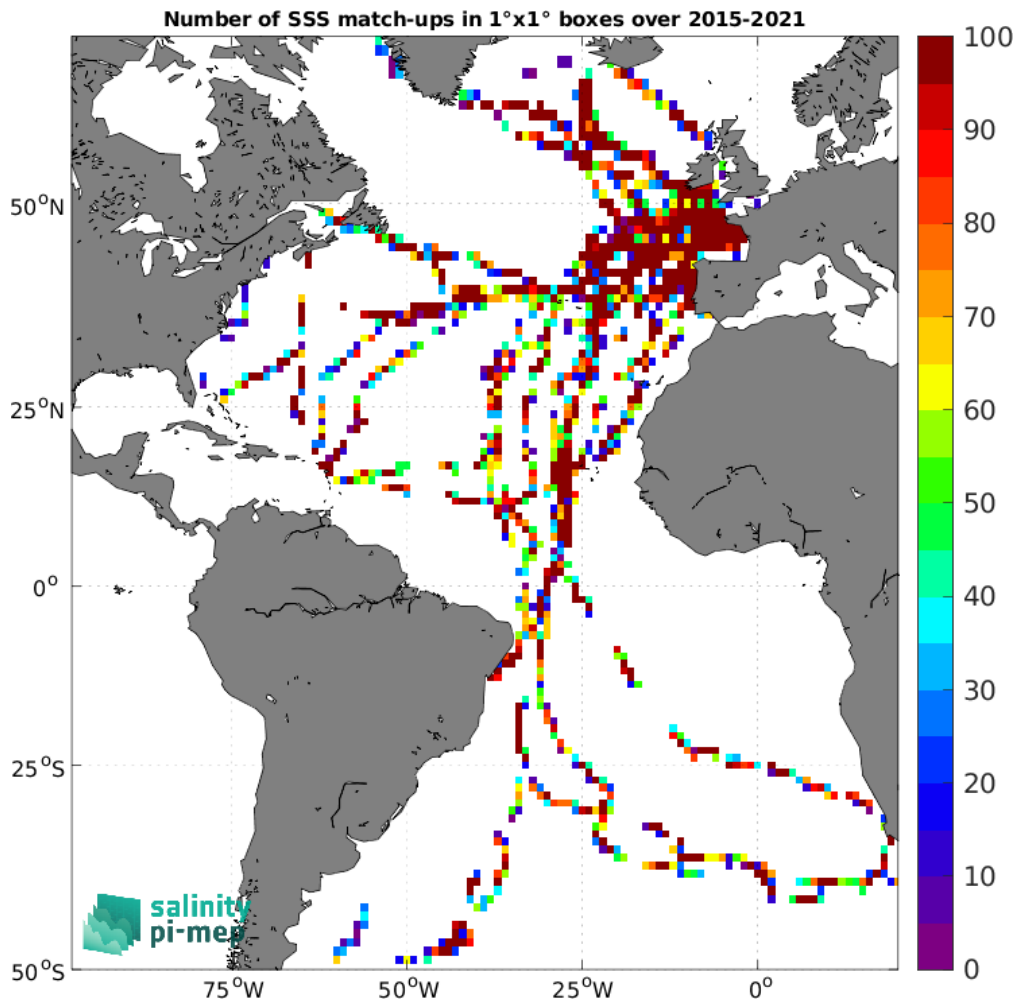
Figure 5: Number of SSS match-ups between TSG (GOSUD-Sailing-ship) SSS and the SMAP SSS L2 v5.3 - 40 km (RSS) SSS product for the Atlantic Ocean Pi-MEP region over 1^\circ \times 1^\circ boxes and for the full satellite product period.
