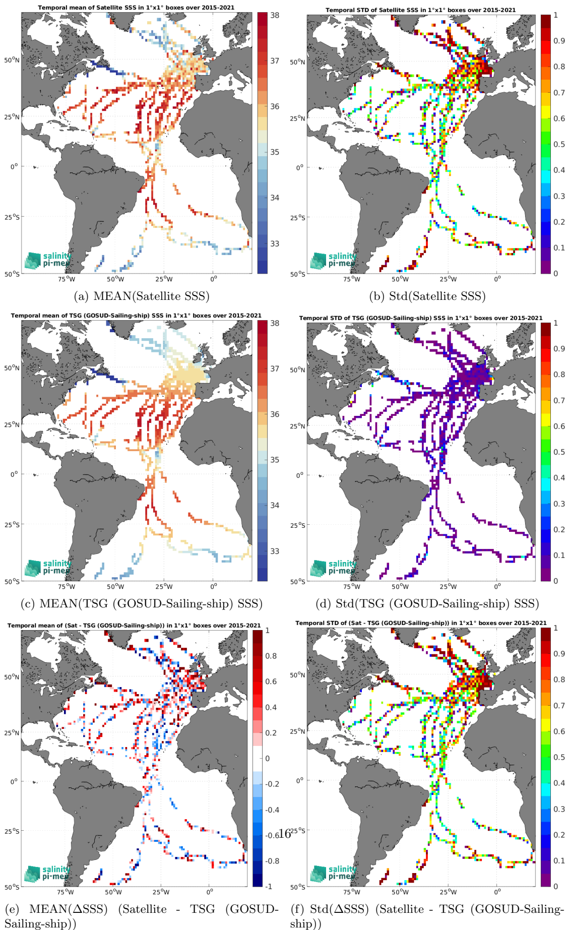
Figure 7: Temporal mean (left) and Std (right) of SSS from SMAP SSS L2 v5.3 - 40 km (RSS) (top), TSG (GOSUD-Sailing-ship) (middle), and of \Delta SSS (Satellite - TSG (GOSUD-Sailing-ship)). Only match-up pairs are used to generate these maps.
