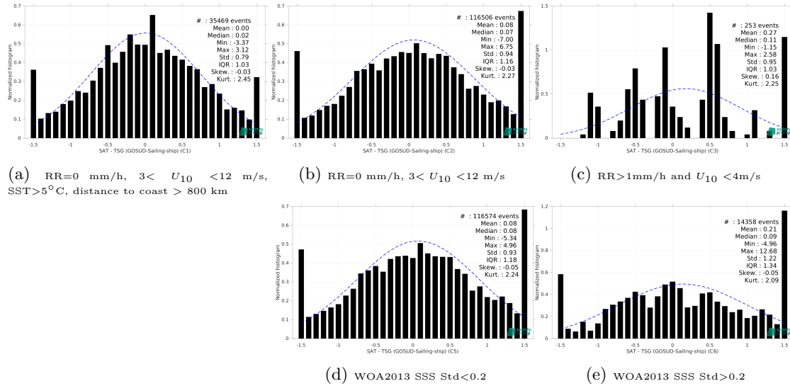
Figure 15: Normalized histogram of \Delta\text{SSS} (SMAP SSS L2 v5.3 - 40 km (RSS) - TSG (GOSUD-Sailing-ship)) for 5 different subdatasets corresponding to: RR=0 mm/h, 3 < U_{10} < 12 m/s, SST>5°C, distance to coast > 800 km (a), RR=0 mm/h, 3 < U_{10} < 12 m/s (b), RR>1mm/h and U_{10} < 4 m/s (c), WOA2013 SSS Std<0.2 (d), WOA2013 SSS Std>0.2 (e).
