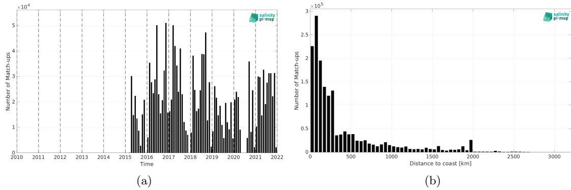
Figure 2: Number of match-ups between TSG (GOSUD-Research-vessel) and SMAP SSS L2 v5.3 - 40 km (RSS) SSS as a function of time (a) and as function of the distance to coast (b) over the Atlantic Ocean Pi-MEP region and for the full satellite product period.
