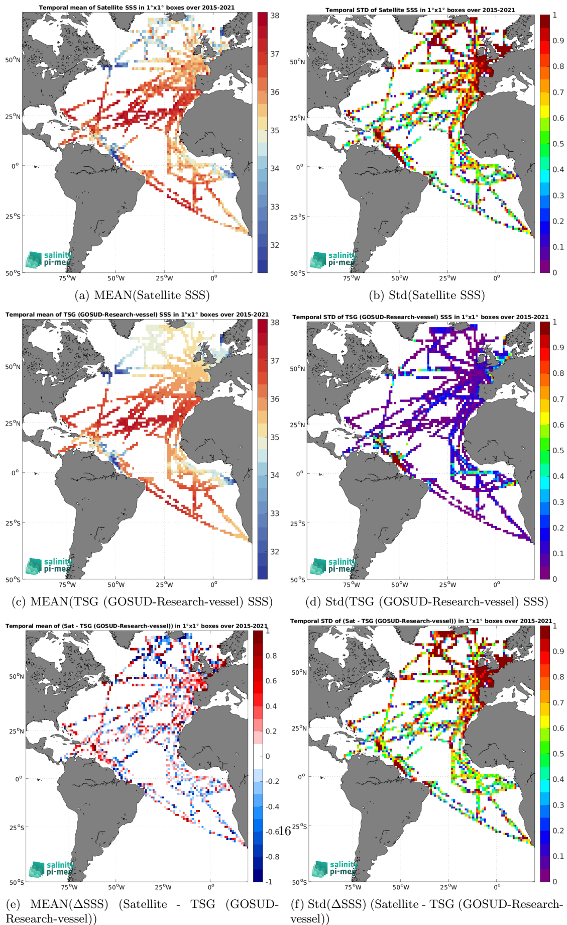
Figure 7: Temporal mean (left) and Std (right) of SSS from SMAP SSS L2 v5.3 - 40 km (RSS) (top), TSG (GOSUD-Research-vessel) (middle), and of \Delta SSS (Satellite - TSG (GOSUD-Research-vessel)). Only match-up pairs are used to generate these maps.
