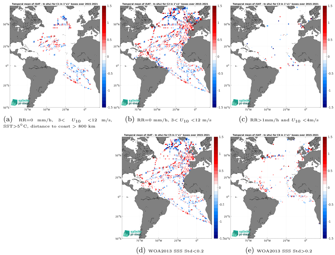
Figure 14: Temporal mean gridded over spatial boxes of size 1^\circ \times 1^\circ of \Delta SSS (SMAP SSS L2 v5.3 - 40 km (RSS) - TSG (GOSUD-Research-vessel)) for 5 different subdatasets corresponding to:RR=0 mm/h, 3 < U_{10} < 12 m/s, SST>5°C, distance to coast > 800 km (a), RR=0 mm/h, 3 < U_{10} < 12 m/s (b), RR>1mm/h and U_{10} < 4 m/s (c), WOA2013 SSS Std<0.2 (d), WOA2013 SSS Std>0.2 (e).
