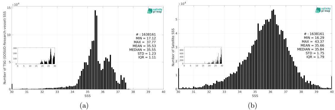
Figure 3: Histograms of SSS from TSG (GOSUD-Research-vessel) (a) and SMAP SSS L2 v5.3 - 40 km (RSS) (b) considering all match-up pairs per bins of 0.1 over the Atlantic Ocean Pi-MEP region and for the full satellite product period.
