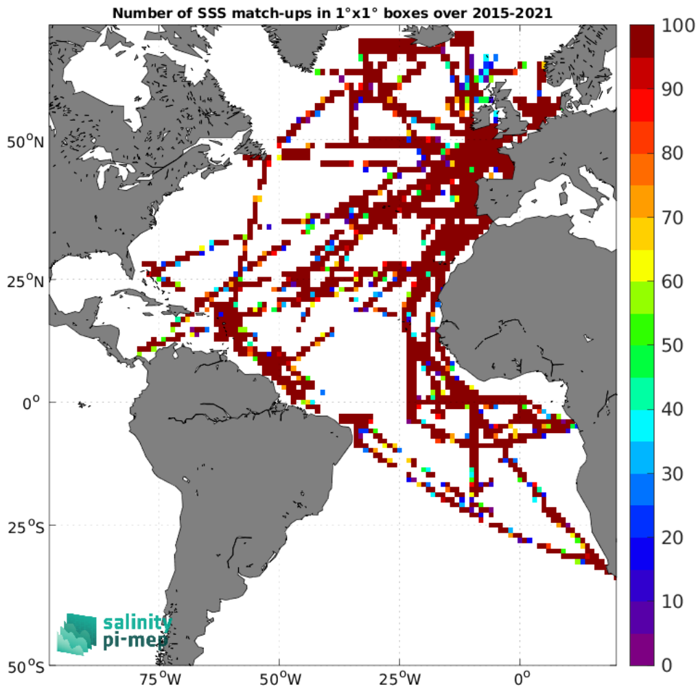
Figure 5: Number of SSS match-ups between TSG (GOSUD-Research-vessel) SSS and the SMAP SSS L2 v5.3 - 40 km (RSS) SSS product for the Atlantic Ocean Pi-MEP region over 1^\circ \times 1^\circ boxes and for the full satellite product period.
