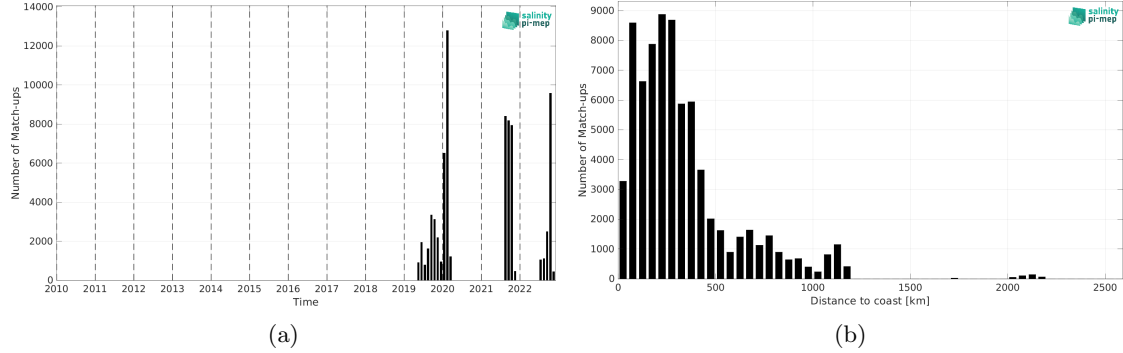
Figure 2: Number of match-ups between Saildrone and SMAP SSS L2 v5.3 - 40 km (RSS) SSS as a function of time (a) and as function of the distance to coast (b) over the Atlantic Ocean Pi-MEP region and for the full satellite product period.
