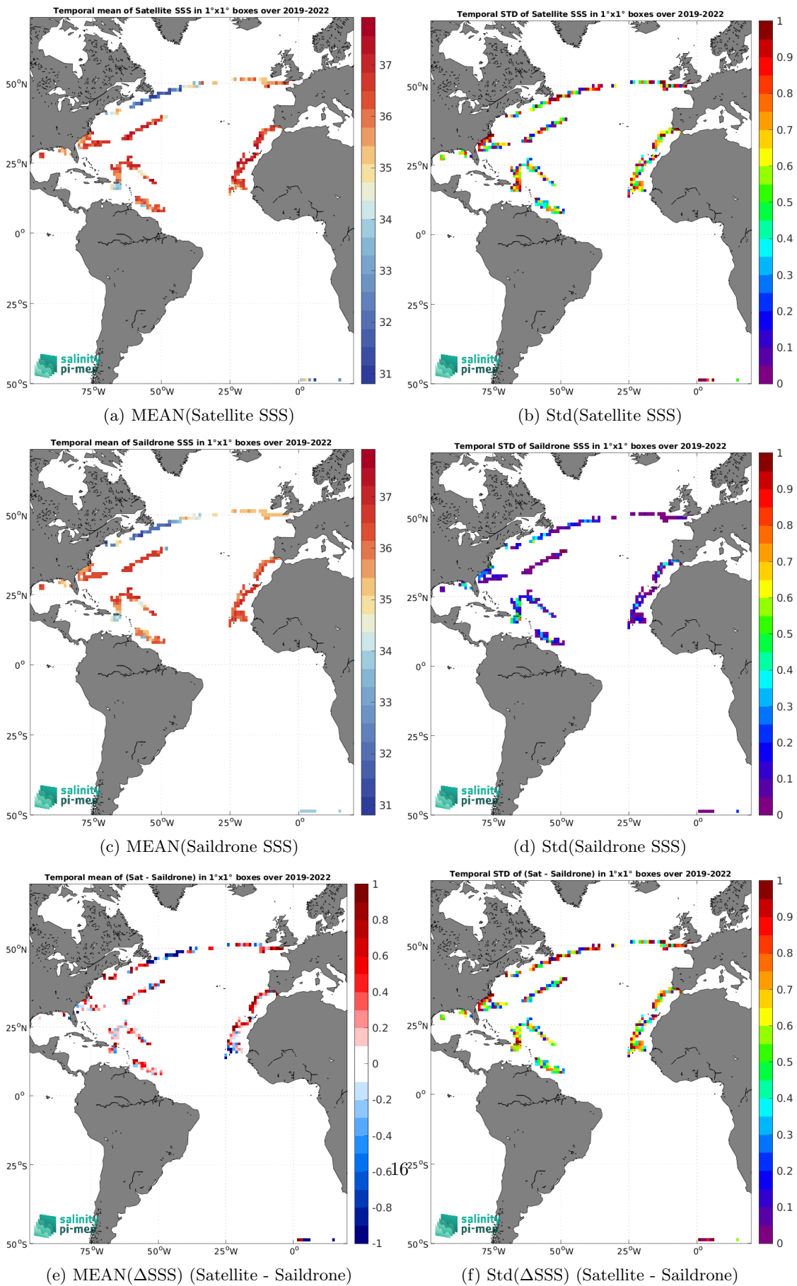
Figure 7: Temporal mean (left) and Std (right) of SSS from SMAP SSS L2 v5.3 - 40 km (RSS) (top), Saildrone (middle), and of \Delta SSS (Satellite - Saildrone). Only match-up pairs are used to generate these maps.
