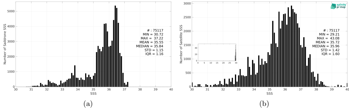
Figure 3: Histograms of SSS from Saildrone (a) and SMAP SSS L2 v5.3 - 40 km (RSS) (b) considering all match-up pairs per bins of 0.1 over the Atlantic Ocean Pi-MEP region and for the full satellite product period.
