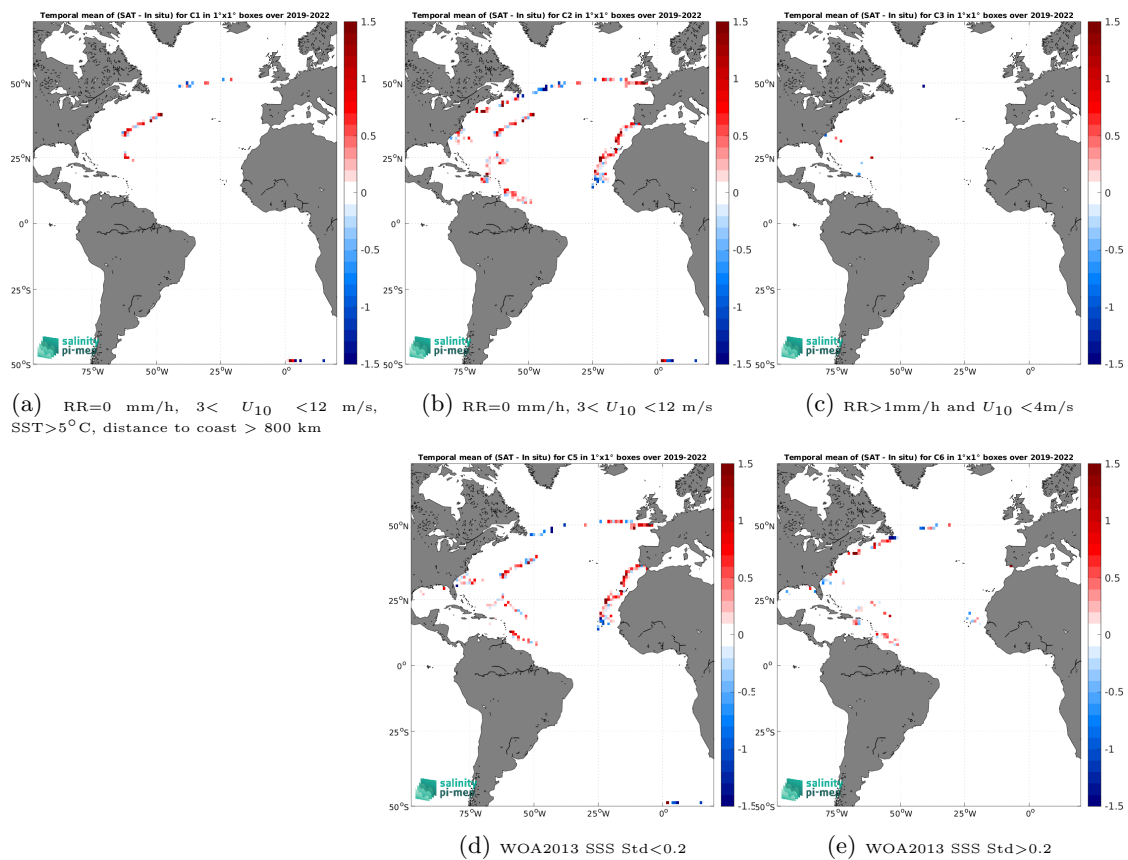
Figure 14: Temporal mean gridded over spatial boxes of size 1^\circ \times 1^\circ of \Delta SSS (SMAP SSS L2 v5.3 - 40 km (RSS) - Sailability) for 5 different subdatasets corresponding to:RR=0 mm/h, 3 < U_{10} < 12 m/s, SST >5^\circ\text{C} , distance to coast > 800 km (a), RR=0 mm/h, 3 < U_{10} < 12 m/s (b), RR >1 mm/h and U_{10} < 4 m/s (c), WOA2013 SSS Std <0.2 (d), WOA2013 SSS Std >0.2 (e).
