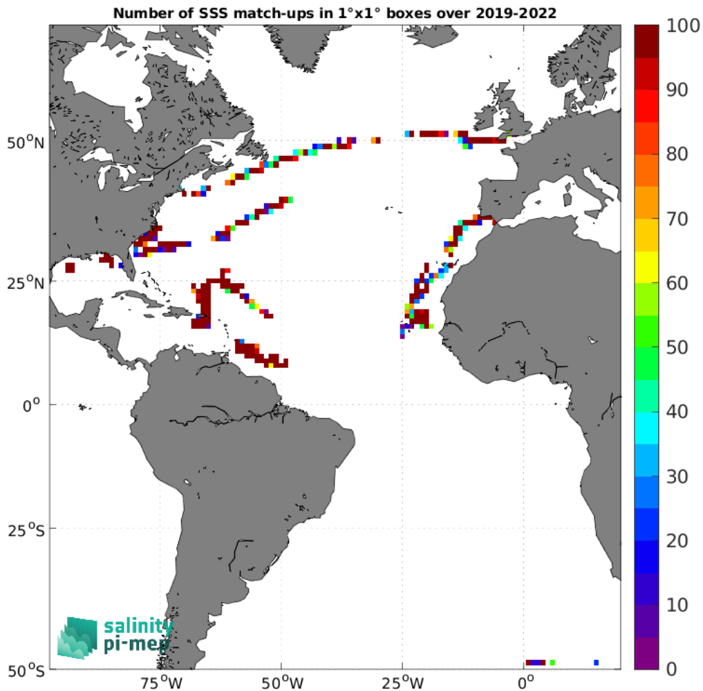
Figure 5: Number of SSS match-ups between Saildrone SSS and the SMAP SSS L2 v5.3 - 40 km (RSS) SSS product for the Atlantic Ocean Pi-MEP region over 1^\circ \times 1^\circ boxes and for the full satellite product period.
