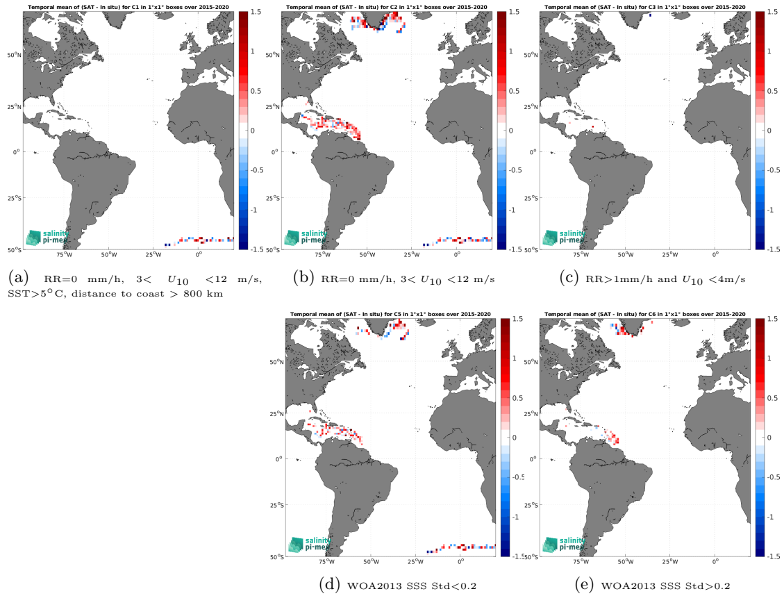
Figure 13: Temporal mean gridded over spatial boxes of size 1^\circ \times 1^\circ of \Delta SSS (SMAP SSS L2 v5.3 - 40 km (RSS) - Surface drifters) for 5 different subdatasets corresponding to:RR=0 mm/h, 3 < U_{10} < 12 m/s, SST >5^\circ\text{C} , distance to coast > 800 km (a), RR=0 mm/h, 3 < U_{10} < 12 m/s (b), RR >1 mm/h and U_{10} < 4 m/s (c), WOA2013 SSS Std <0.2 (d), WOA2013 SSS Std >0.2 (e).
