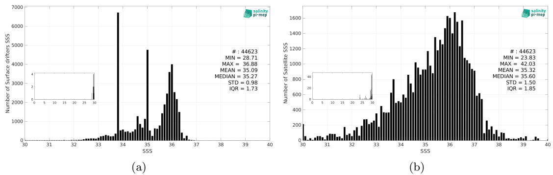
Figure 3: Histograms of SSS from Surface drifters (a) and SMAP SSS L2 v5.3 - 40 km (RSS) (b) considering all match-up pairs per bins of 0.1 over the Atlantic Ocean Pi-MEP region and for the full satellite product period.
