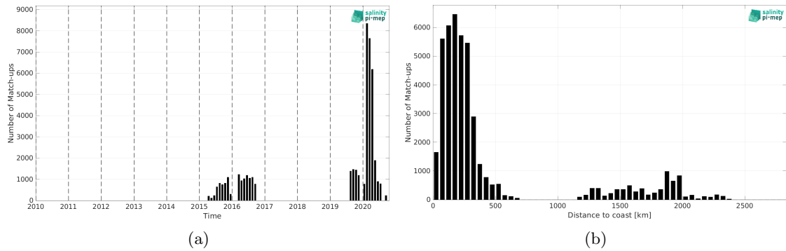
Figure 2: Number of match-ups between Surface drifters and SMAP SSS L2 v5.3 - 40 km (RSS) SSS as a function of time (a) and as function of the distance to coast (b) over the Atlantic Ocean Pi-MEP region and for the full satellite product period.
