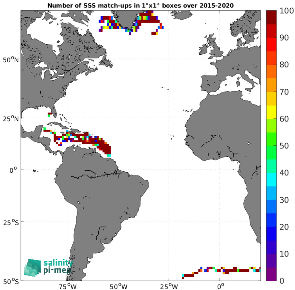
Figure 4: Number of SSS match-ups between Surface drifters SSS and the SMAP SSS L2 v5.3 - 40 km (RSS) SSS product for the Atlantic Ocean Pi-MEP region over 1°×1° boxes and for the full satellite product period.
